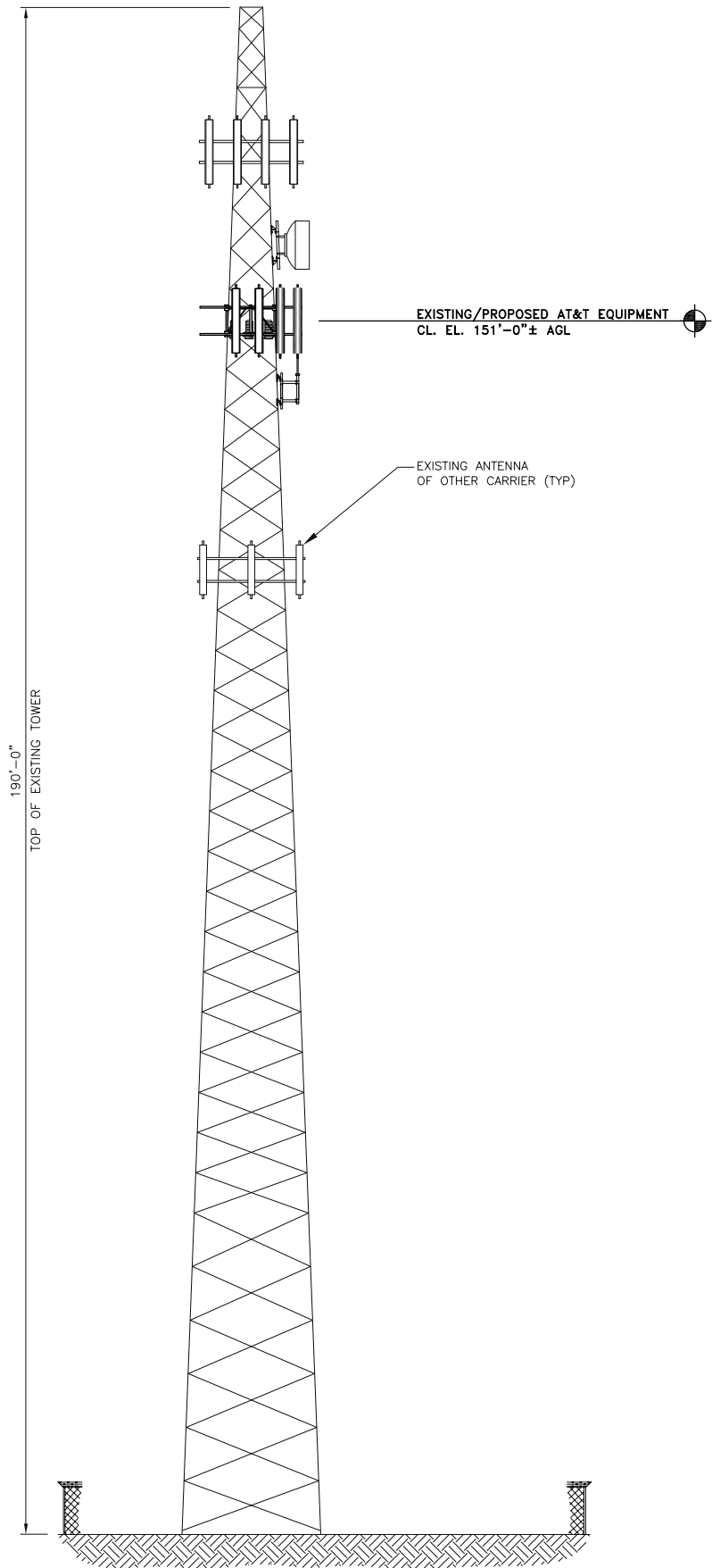
FINAL ELEVATION
