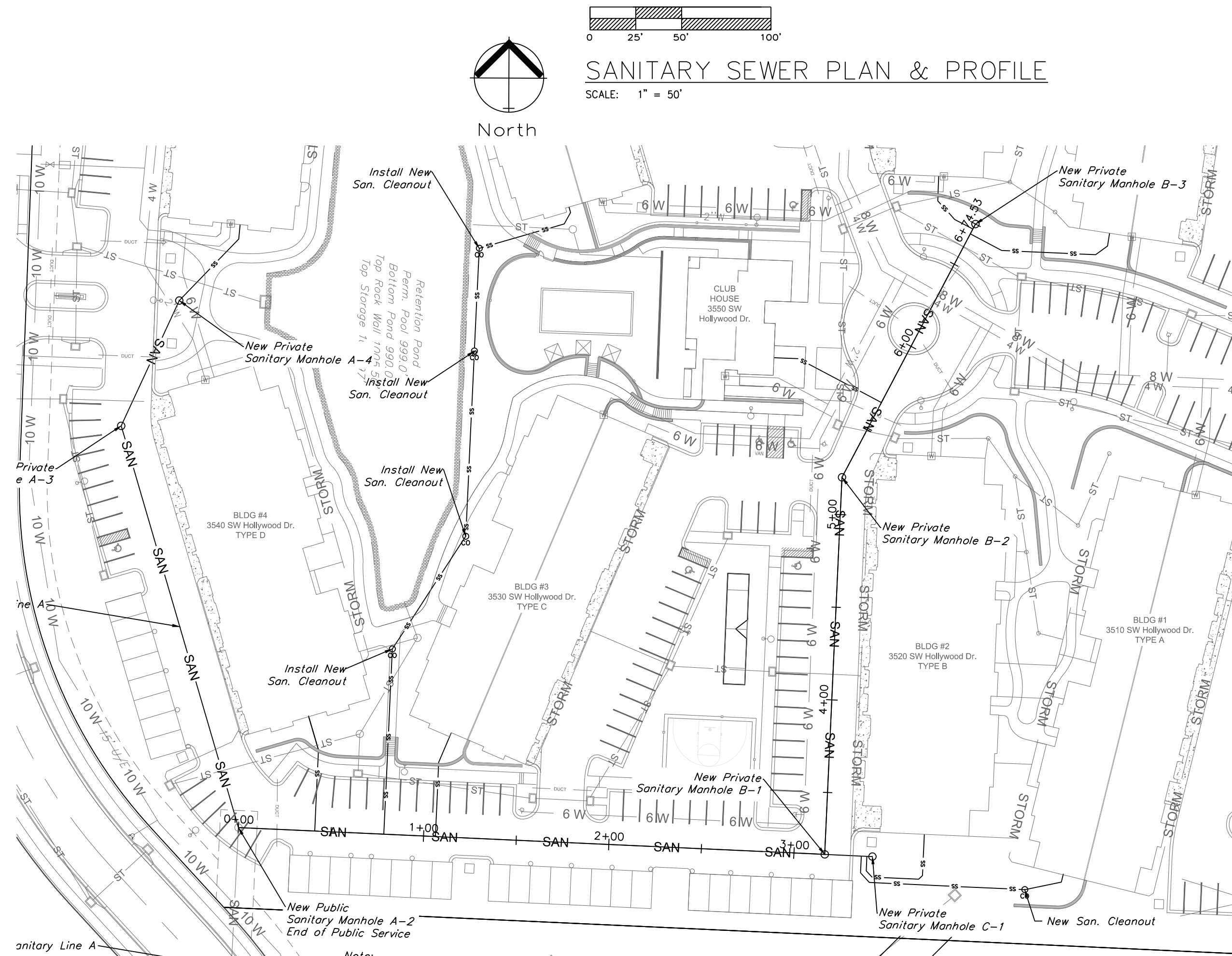
PRIVATE SANITARY LINE B
