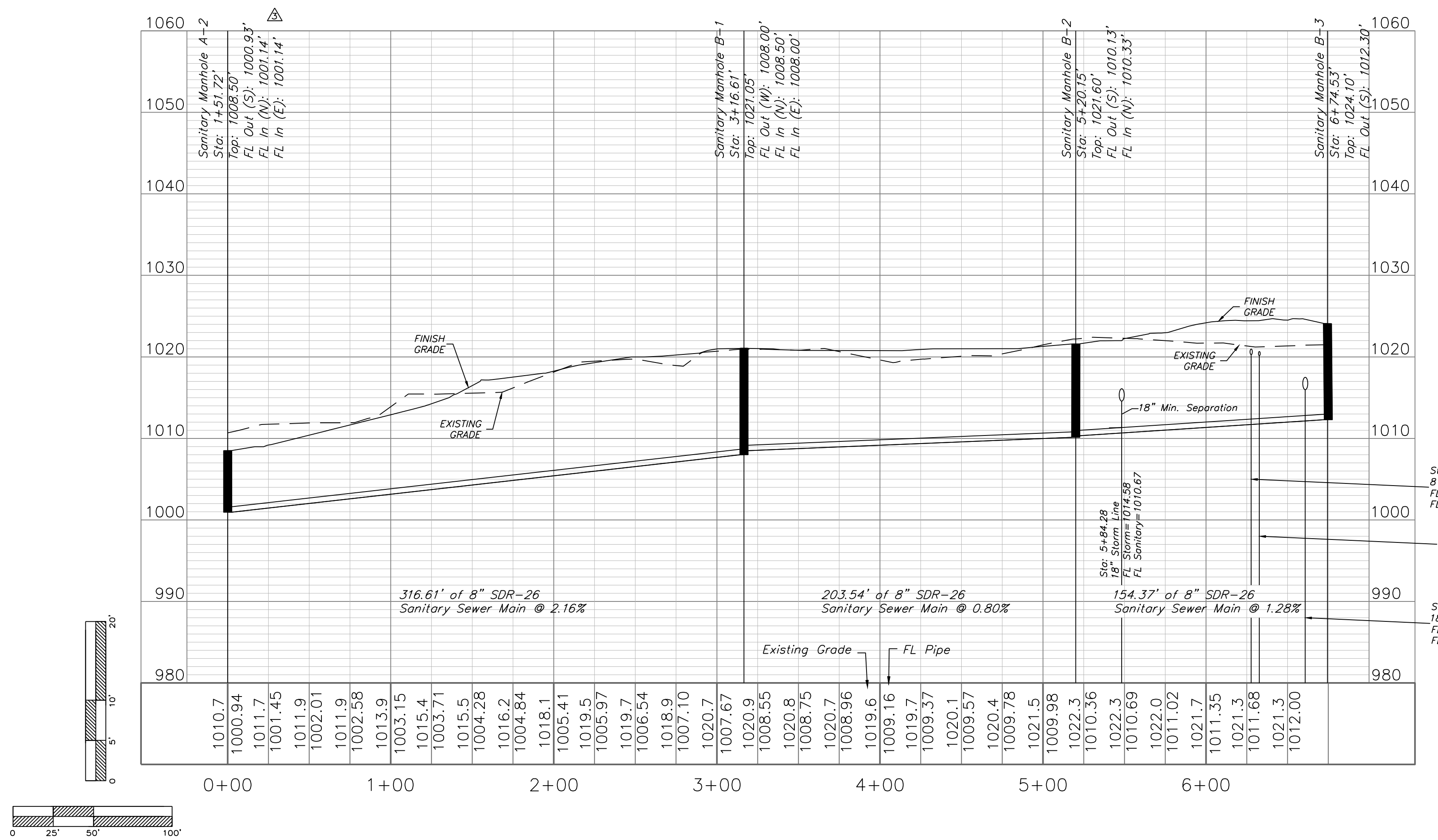
PRIVATE SANITARY LINE B
