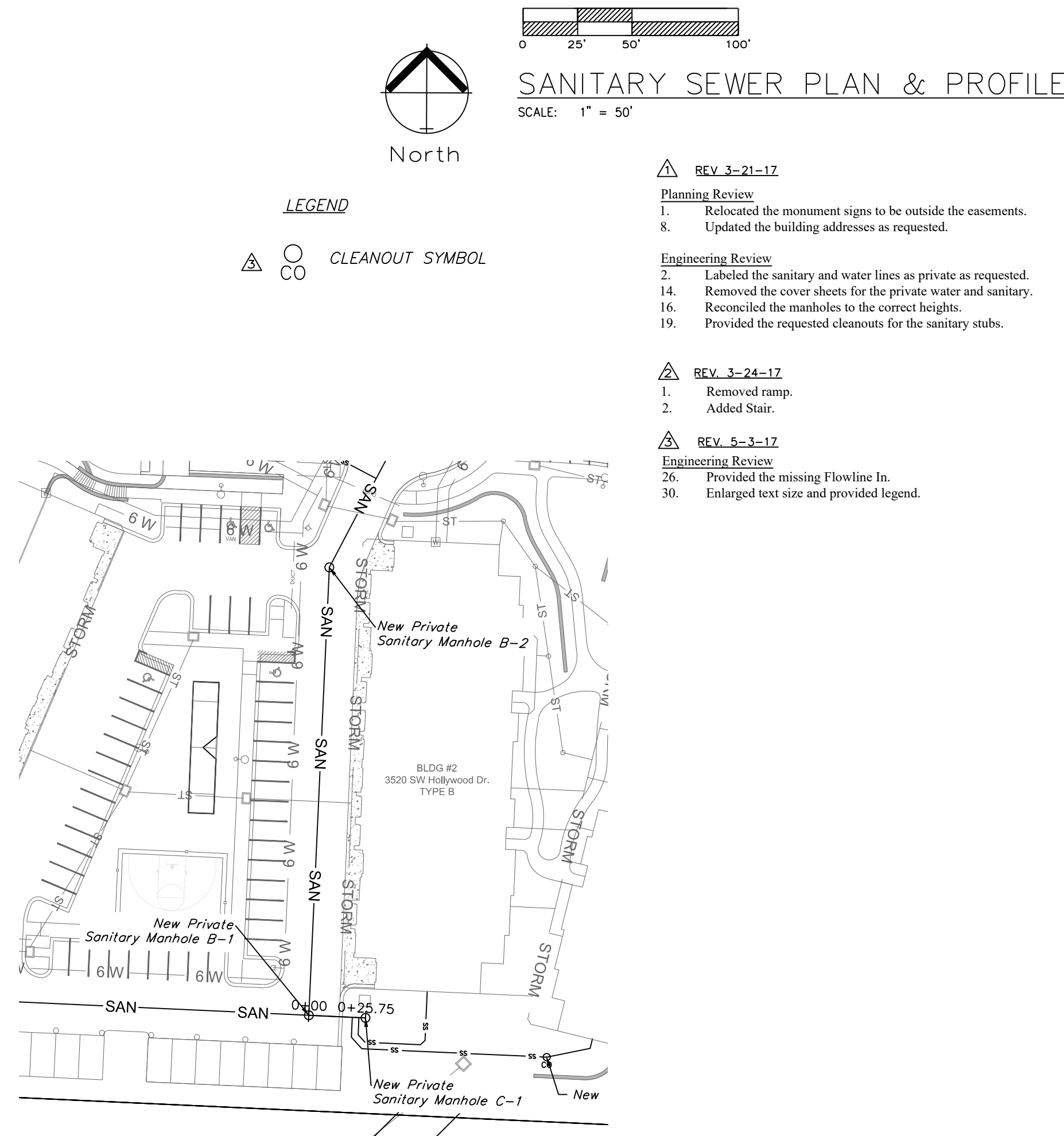
PRIVATE SANITARY LINE C
