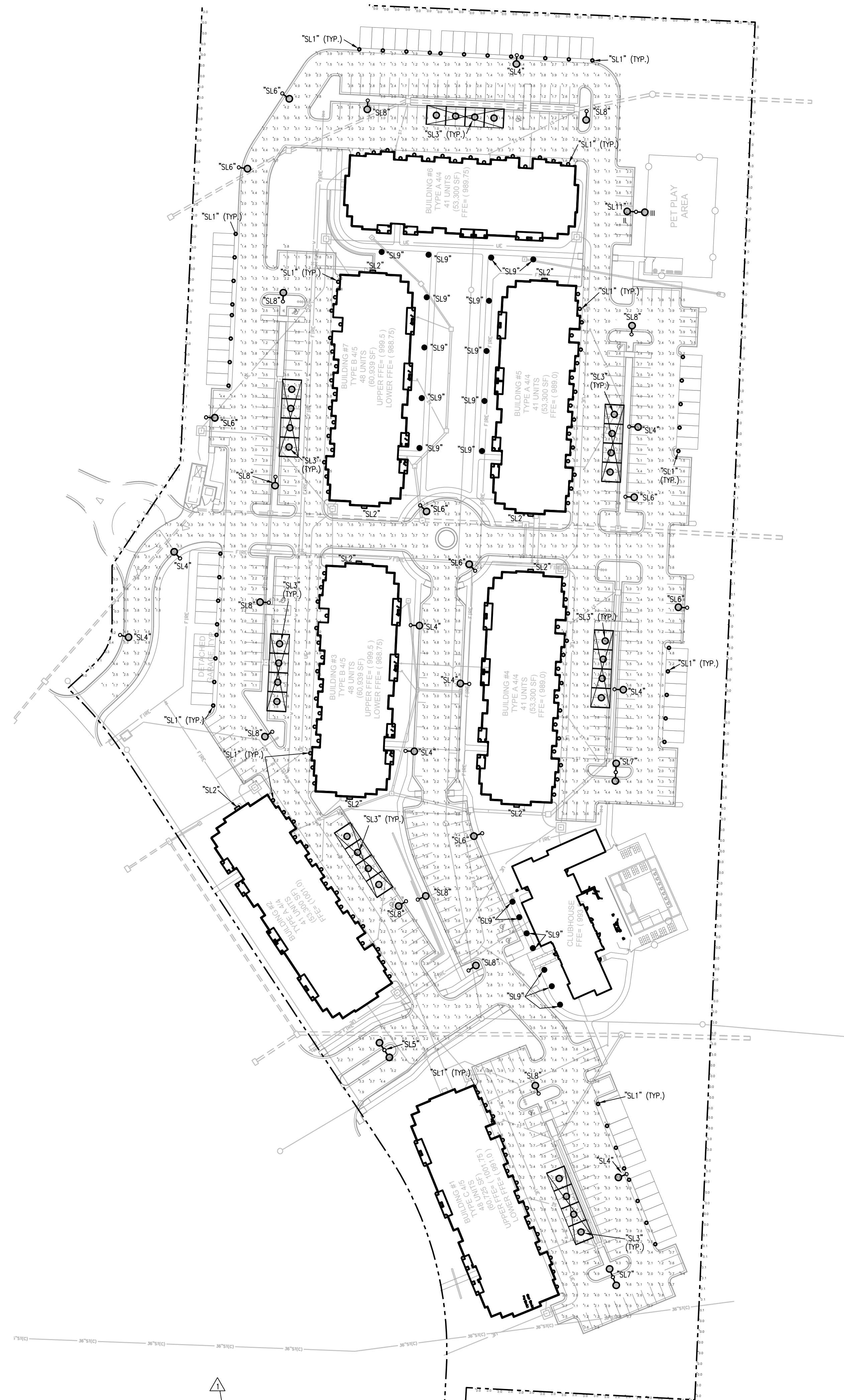
1 PHOTOMETRIC SITE PLAN 1"=60'-0" NORTH
