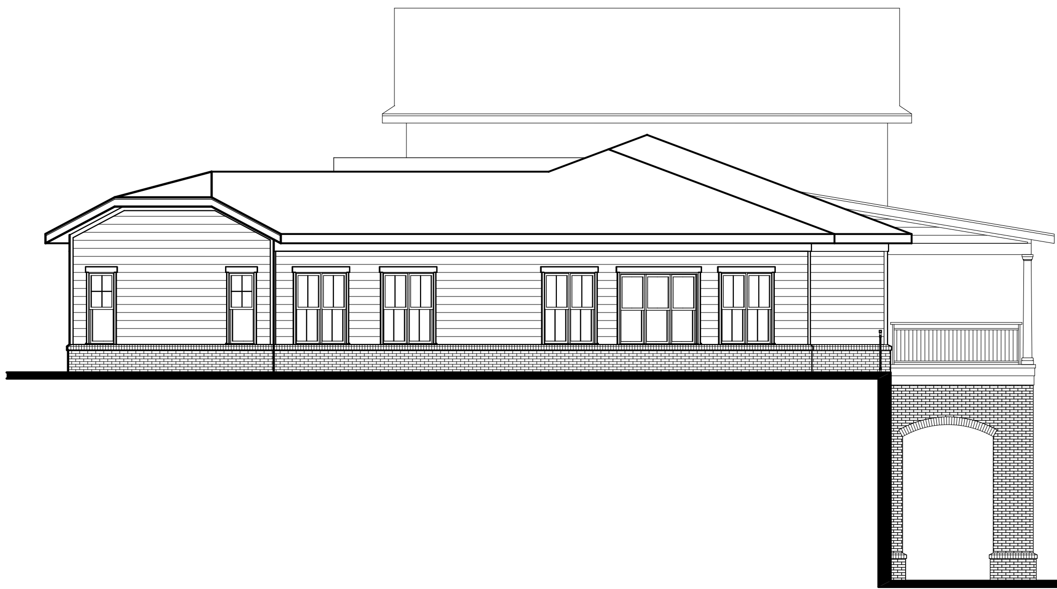
Lease & Amenity Center - Side
