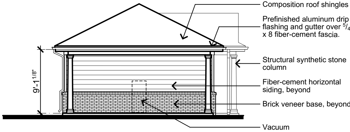
Maintenance Building - Care Care Side
