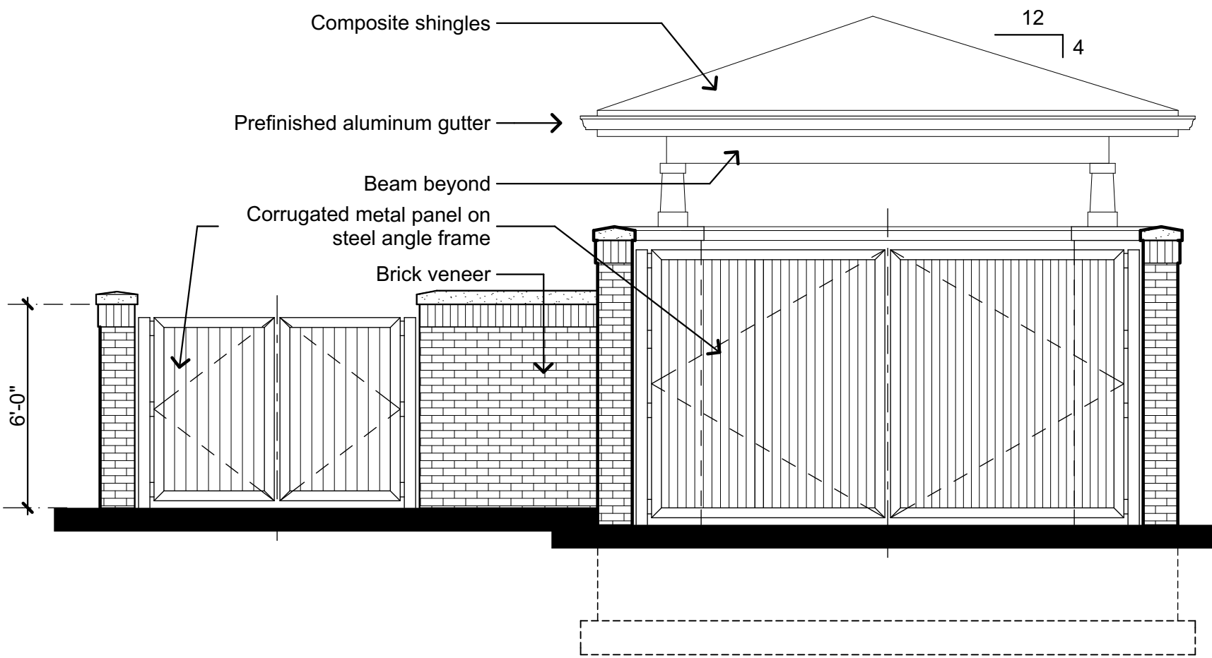
Compactor Elevation - Front
