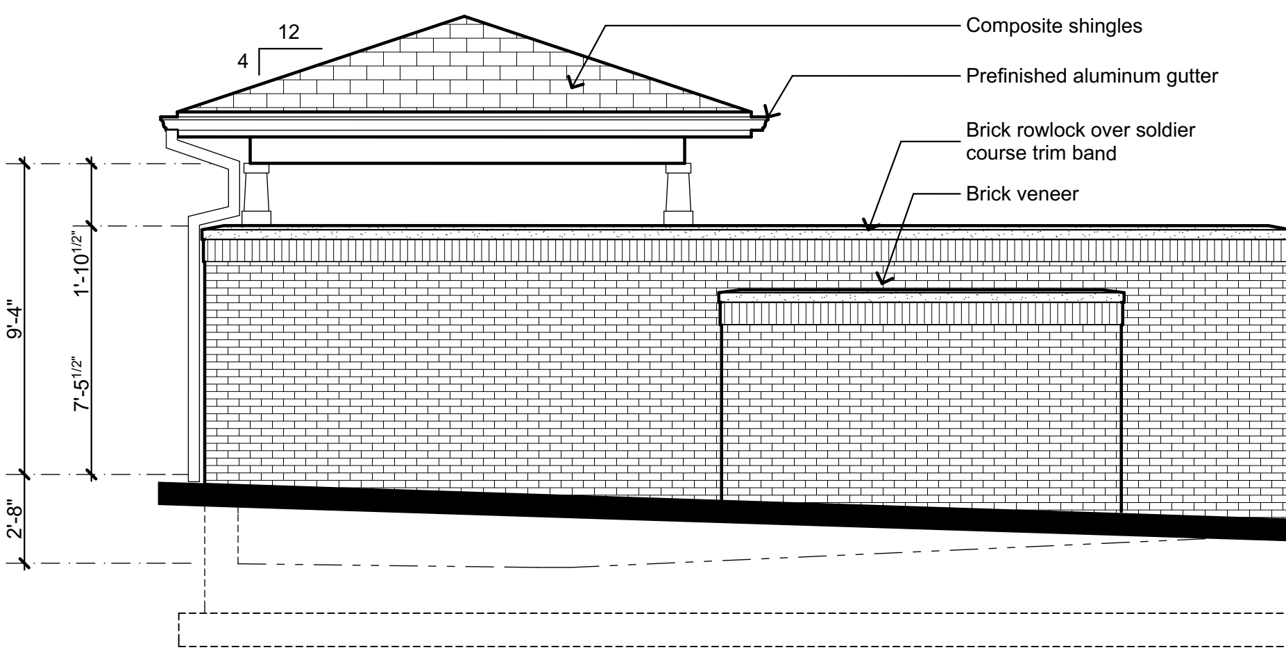
Compactor Elevation - Side
