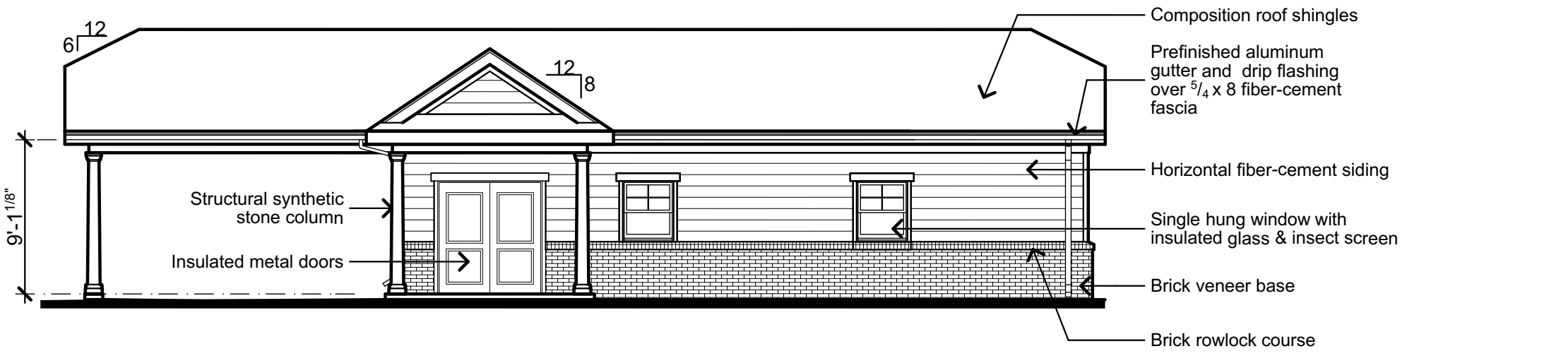
Maintenance Building - Front
