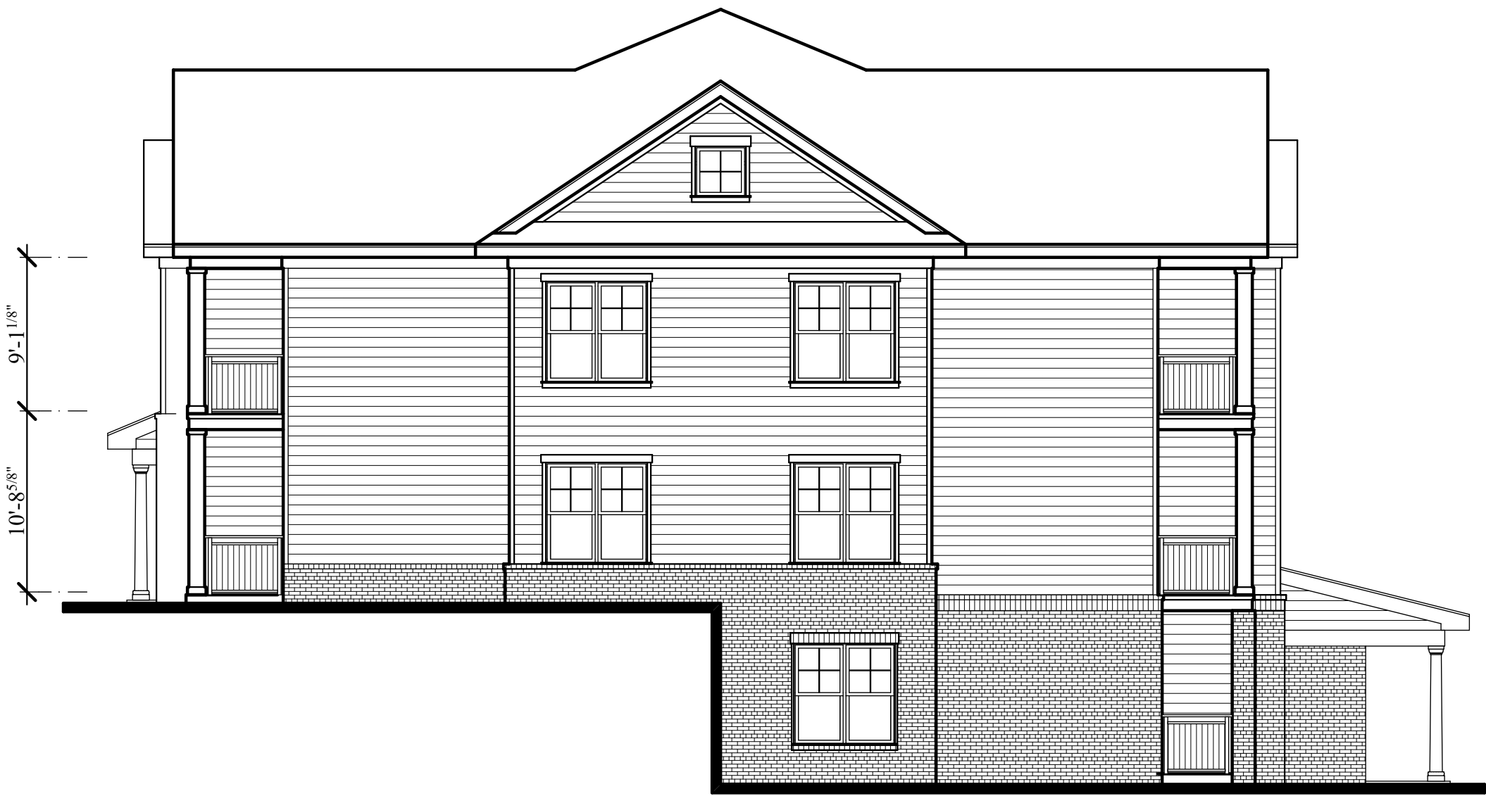
Building Type V
