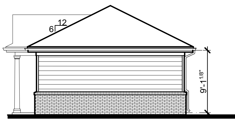
Maintenance Building - Side
