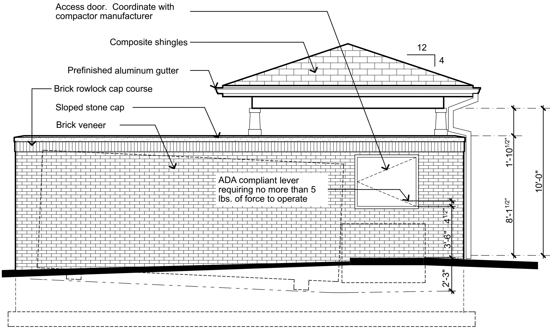
Compactor Elevation - Side
