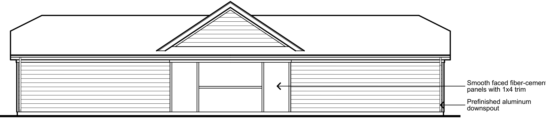
6-Bay Garage - Rear
