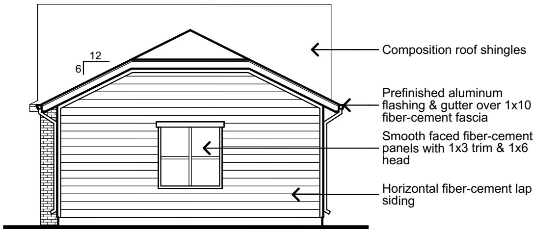
6-Bay Garage - Side
