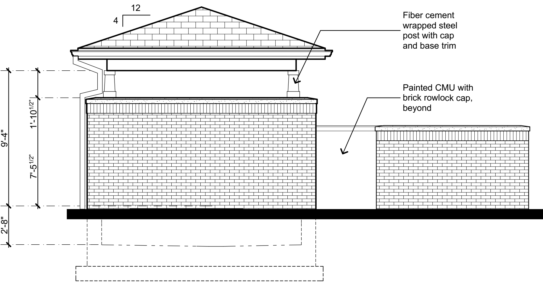
Compactor Elevation - Rear
