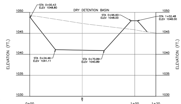
SE BASIN 2 PROFILE SCALE H:1"=20'; V:1"=5' SCALE IN FEET (HORIZONTAL) 0 20 40 SCALE IN FEET (VERTICAL) 0 5 10
