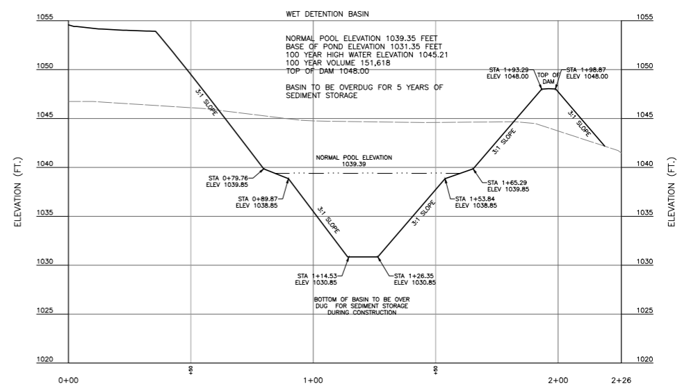
SE BASIN PROFILE SCALE H:1"=20'; V:1"=5' SCALE IN FEET (HORIZONTAL) 0 20 40 SCALE IN FEET (VERTICAL) 0 5 10
