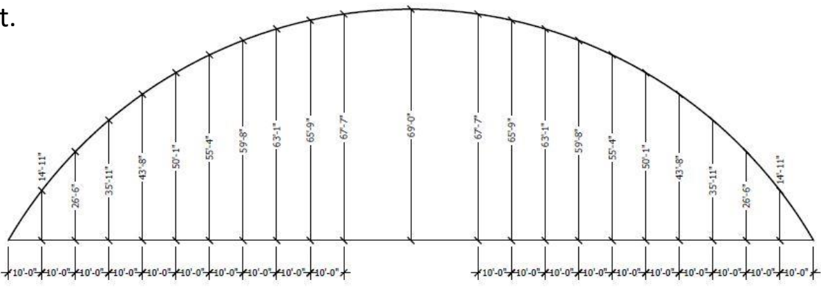
01 DOME PROFILE HEIGHTS SCALE: 1/16" = 1'-0"
