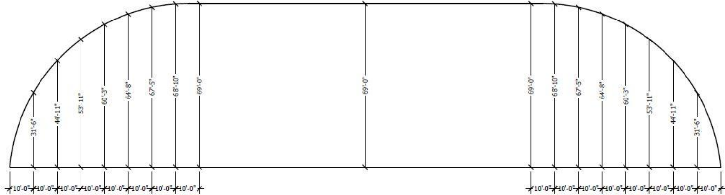
02 DOME PROFILE HEIGHTS SCALE: 1/16" = 1'-0"
