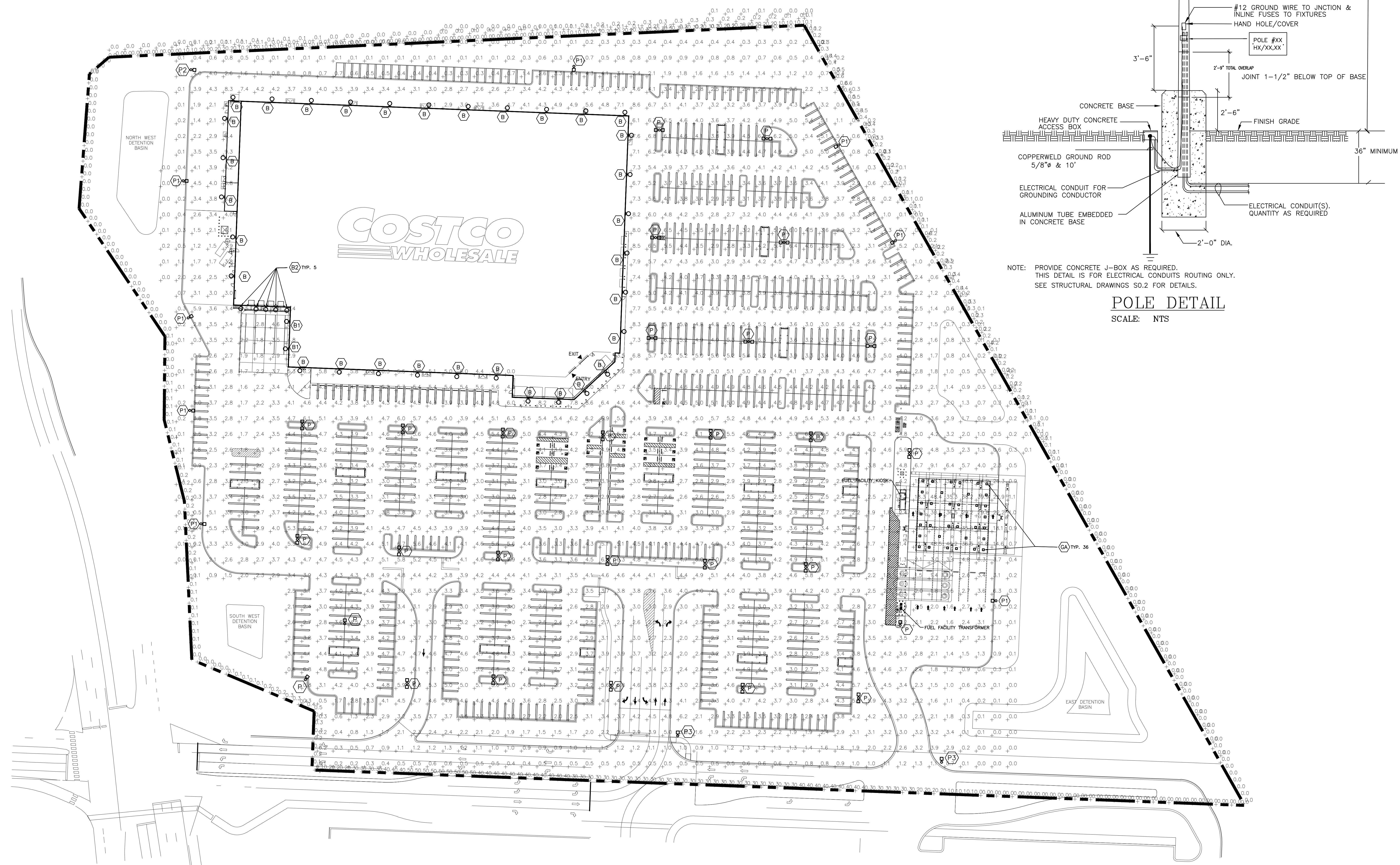
SITE PHOTOMETRIC PLAN SCALE: 1" = 50'-0"
