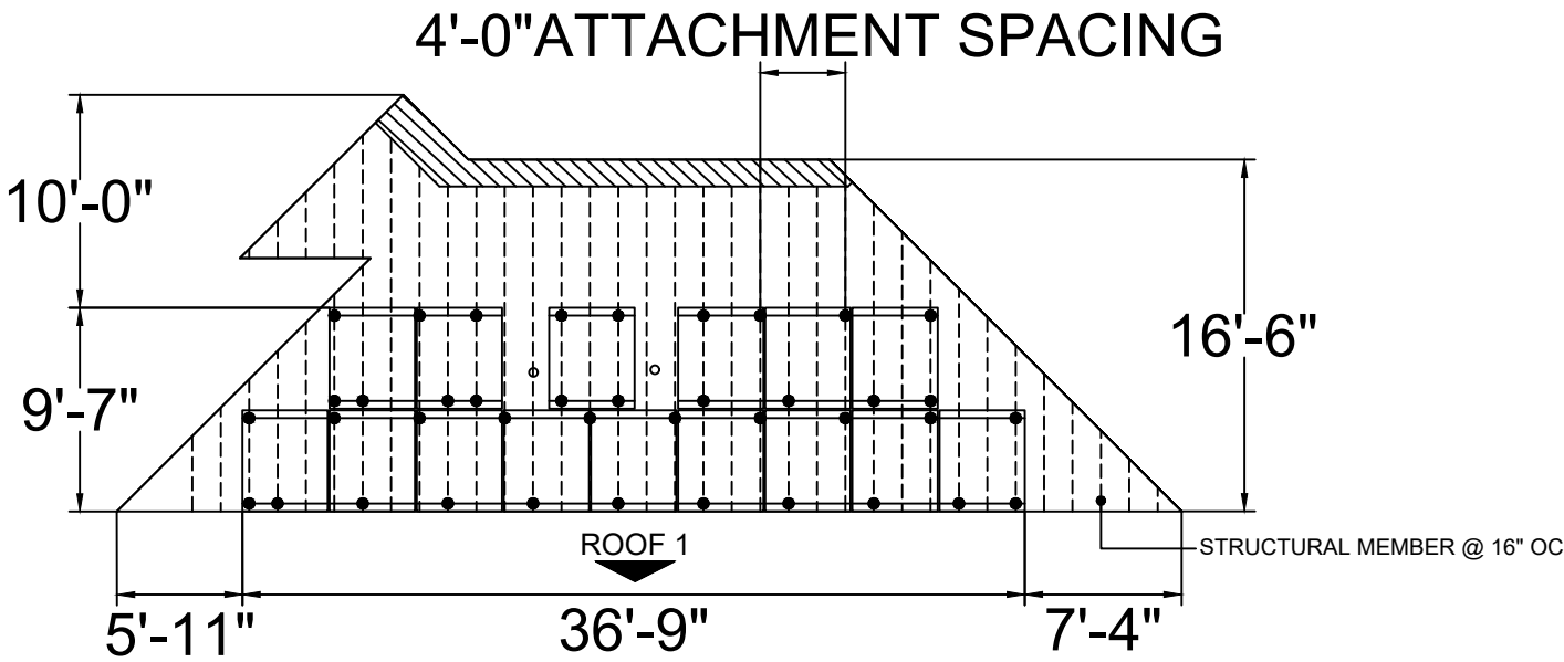
1 ATTACHMENT PLAN SCALE: NTS
