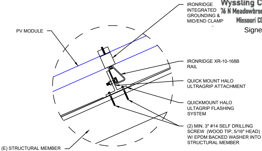
3 ENLARGED VIEW Scale: NTS
