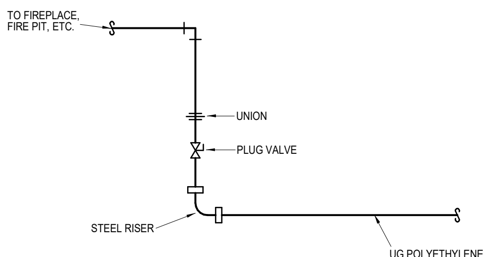
PIPING SCHEMATIC
