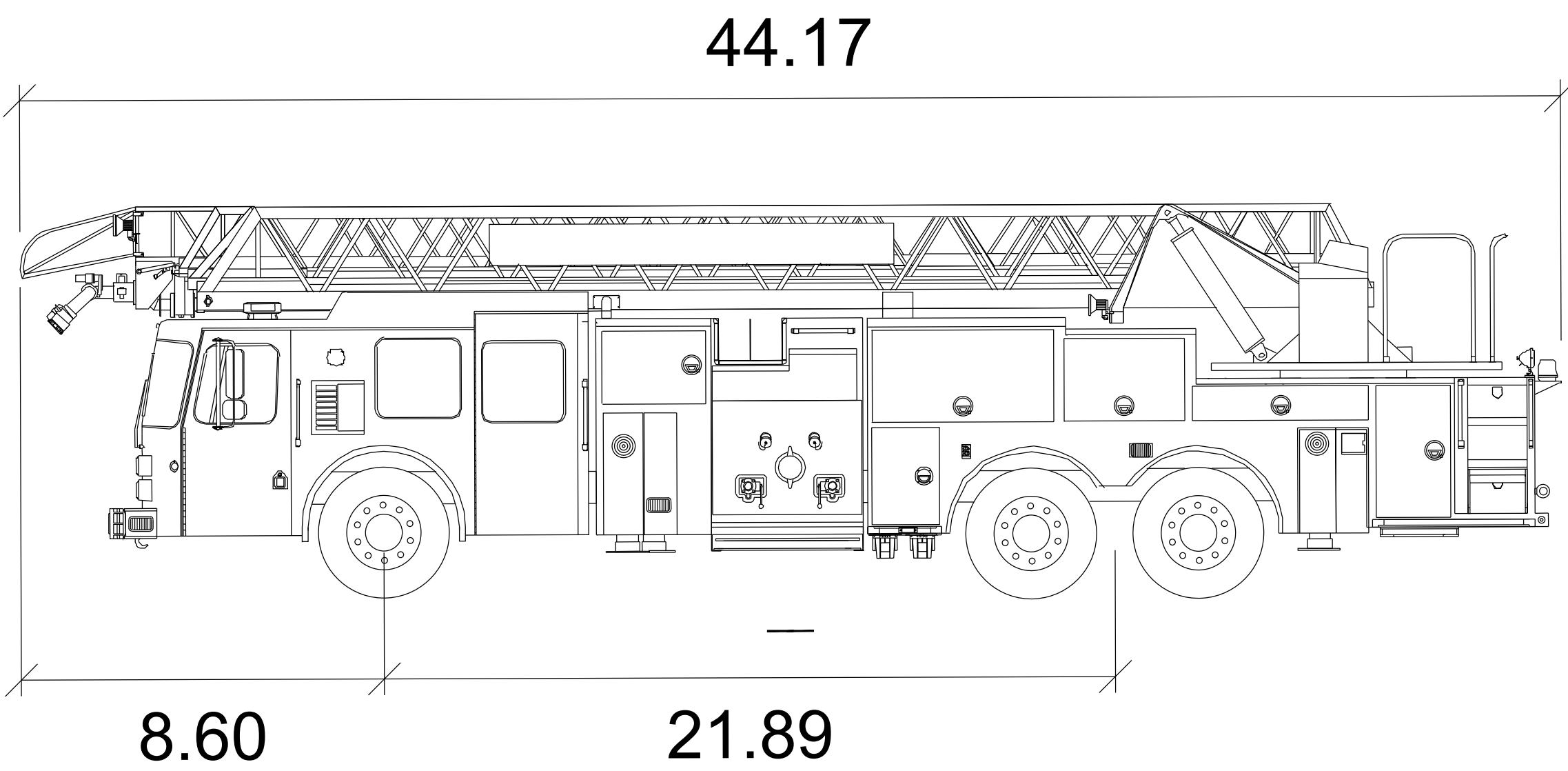
VFCFD 105' AERIAL LADDER PIERCE QUANTUM
