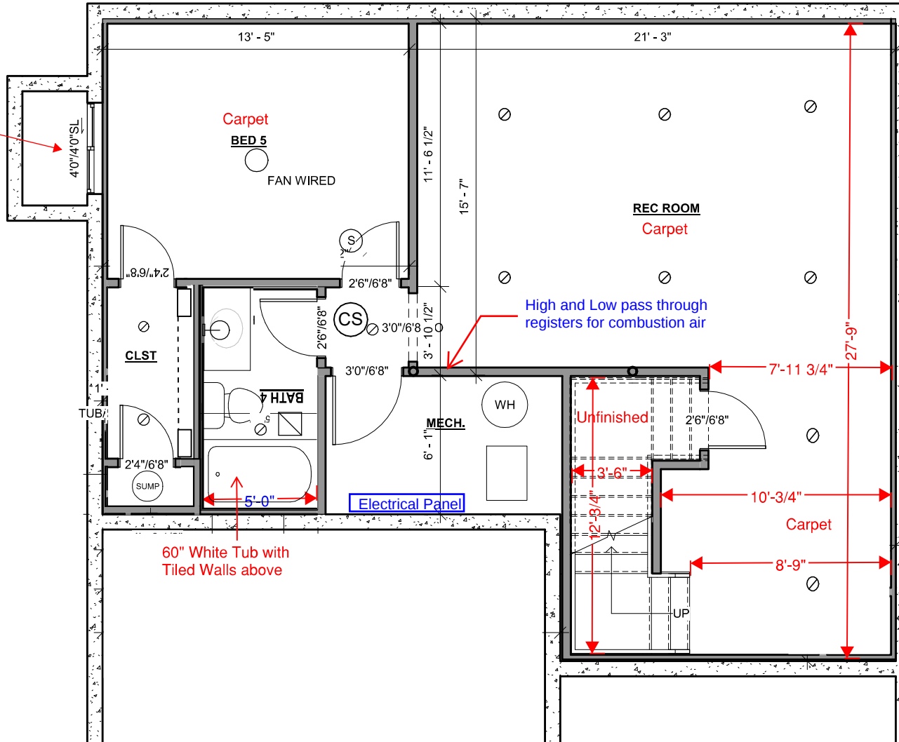
PLAN VIEW - OPT FINISHED LOWER LEVEL ② 1/4" = 1'-0"
