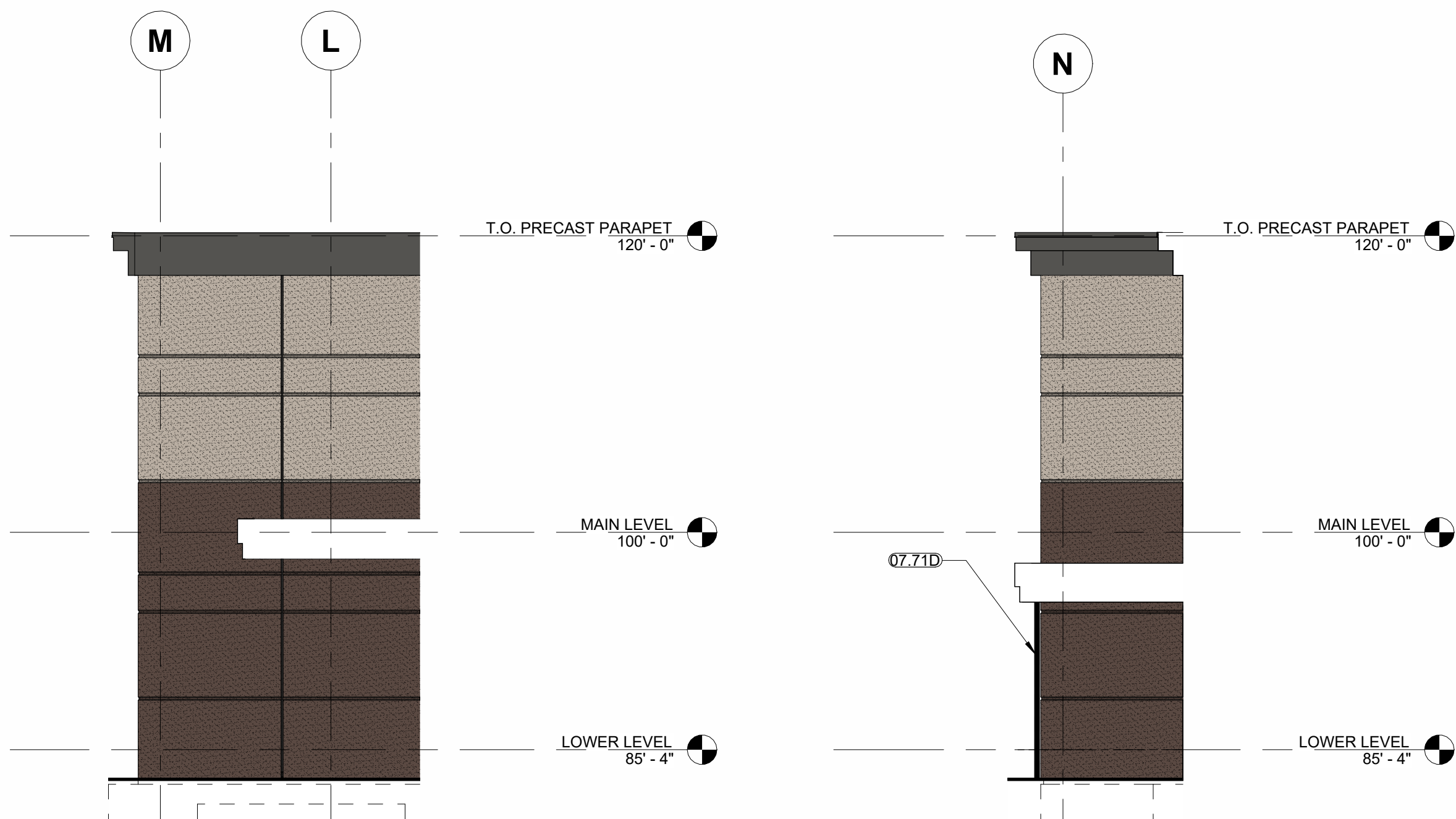
A11 NORTH CORNER ELEVATION 1/8" = 1'-0"
