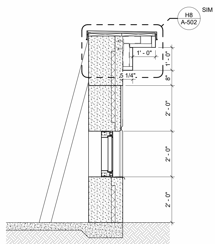
G7 MOCKUP PRECAST WALL SECTION 1/2" = 1'-0"
