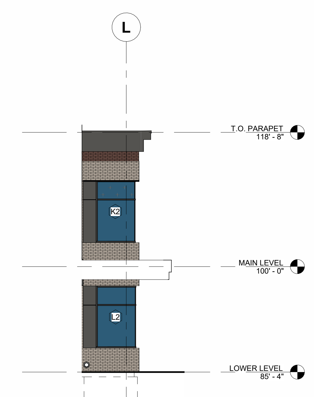
D1 SOUTH CORNER ELEVATION 1/8" = 1'-0"
