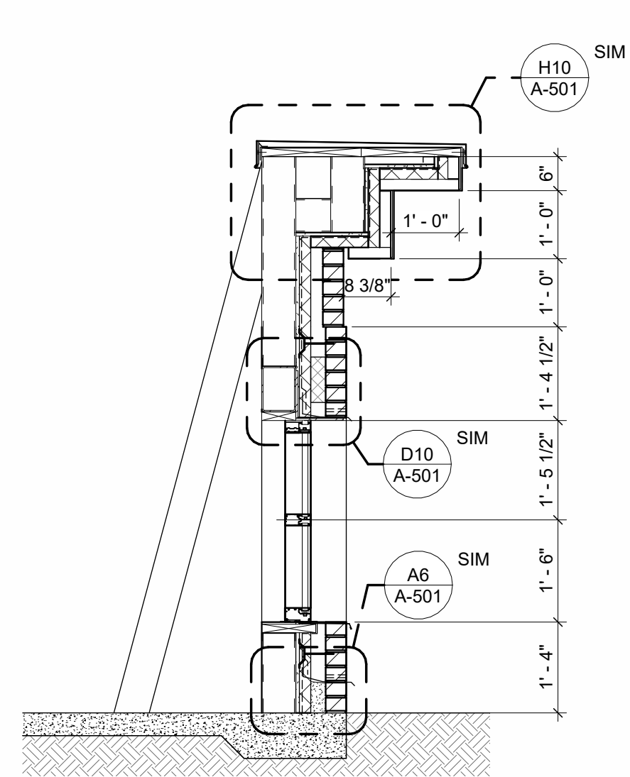
G4 MOCKUP BRICK WALL SECTION 1/2" = 1'-0"
