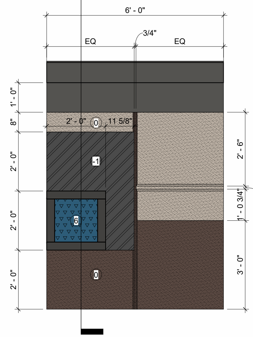
G5 MOCKUP WALL PRECAST 1/2" = 1'-0"
