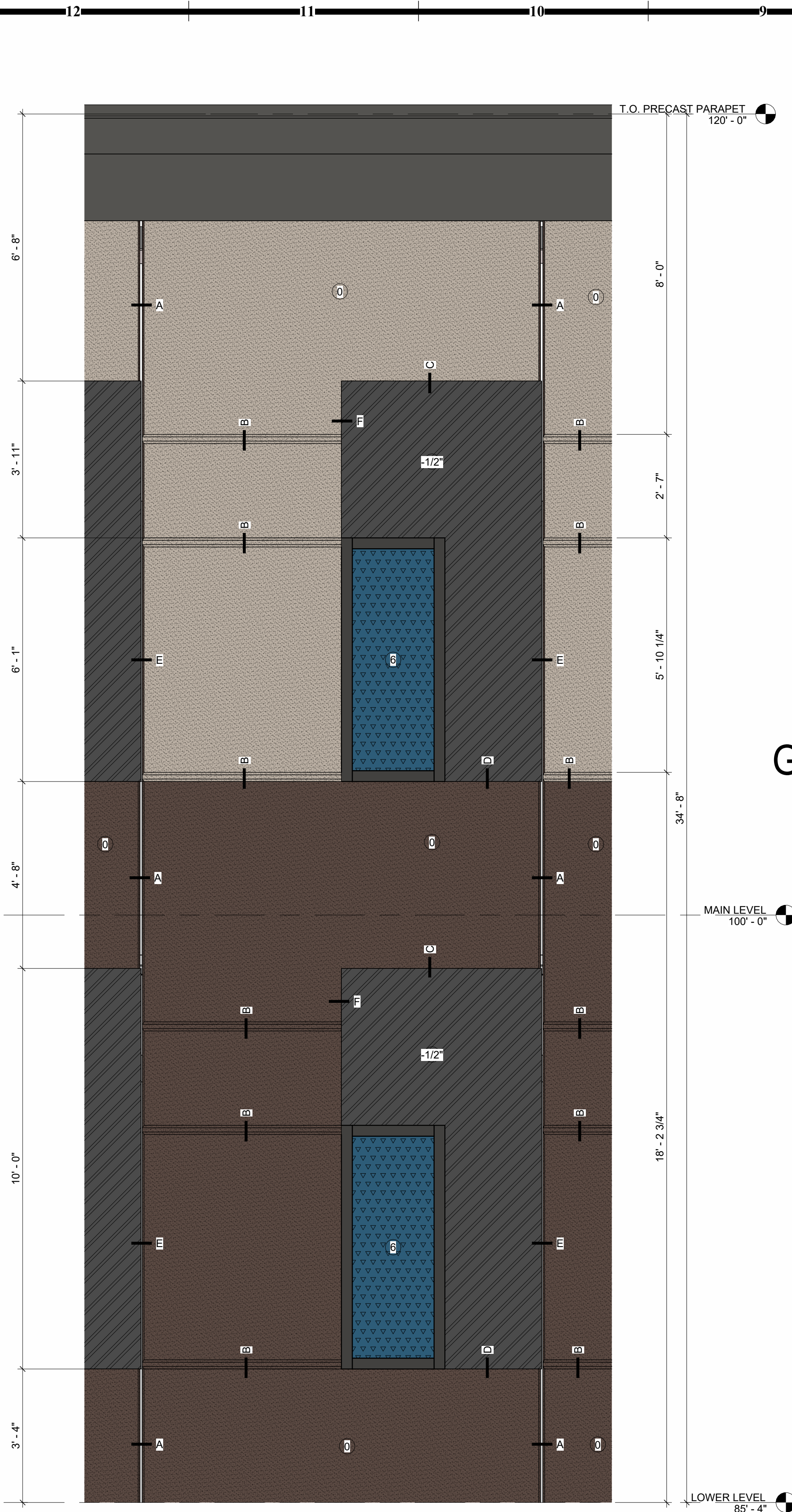
D11 ENLARGED ELEVATION PRECAST 1/2" = 1'-0"
