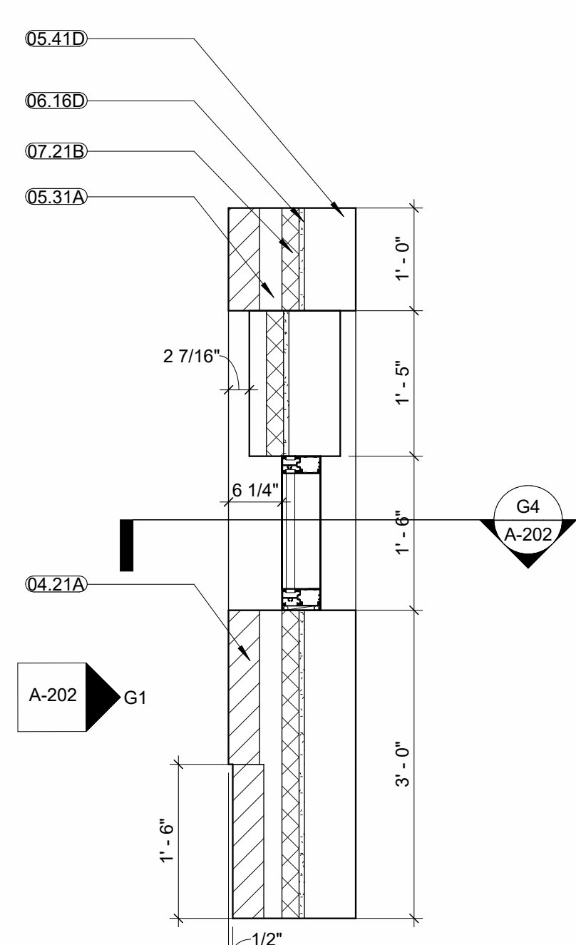
D4 MOCKUP BRICK WALL PLAN 3/4" = 1'-0"
