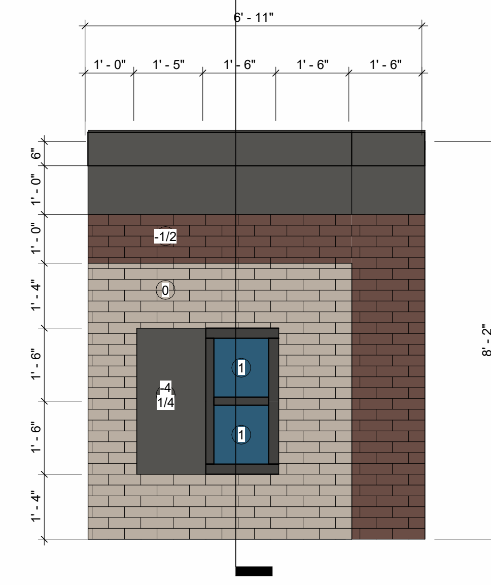
G1 MOCKUP WALL BRICK 1/2" = 1'-0"
