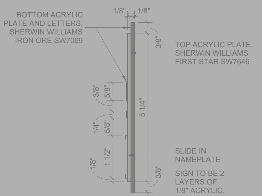
E5 SIGNAGE - ROOM NAME SECTION 6" = 1'-0"
