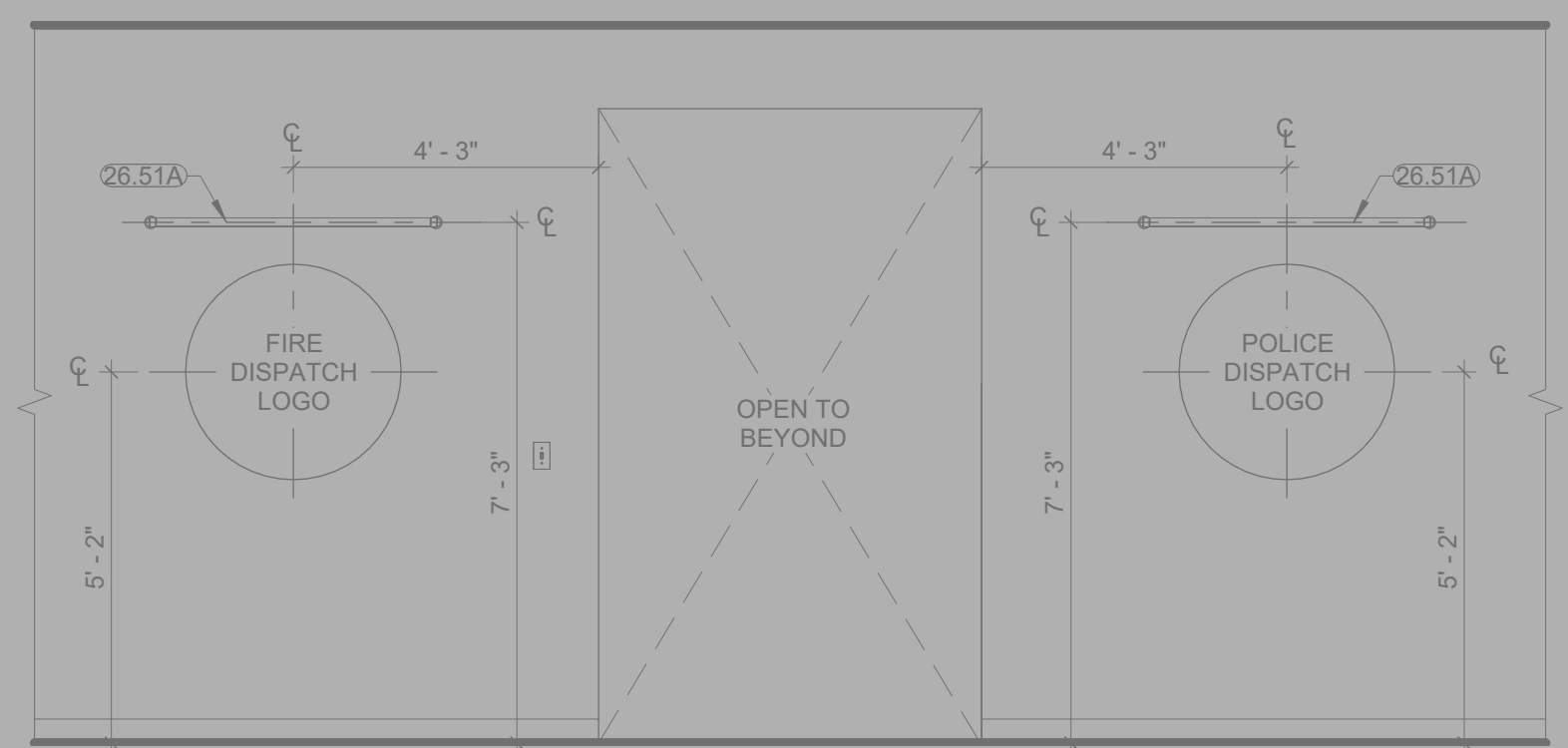
C1 010 COPY/WORK - W SIGNAGE 3/8" = 1'-0"
