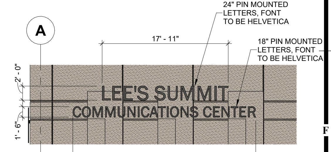
E1 EXTERIOR SIGNAGE - SOUTH 1/8" = 1'-0"
