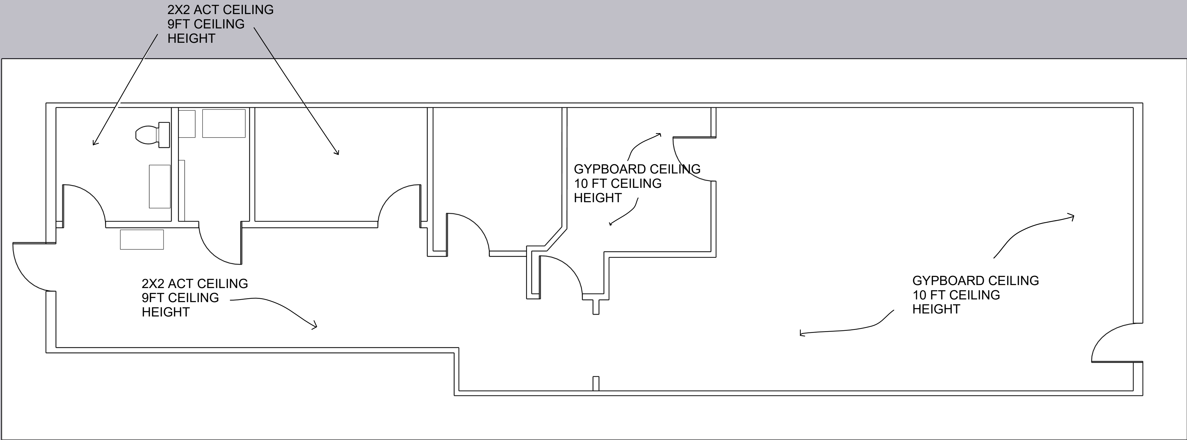
2 FLOOR PLAN REFLECTED CEILING Scale: 1/4" : 1'
