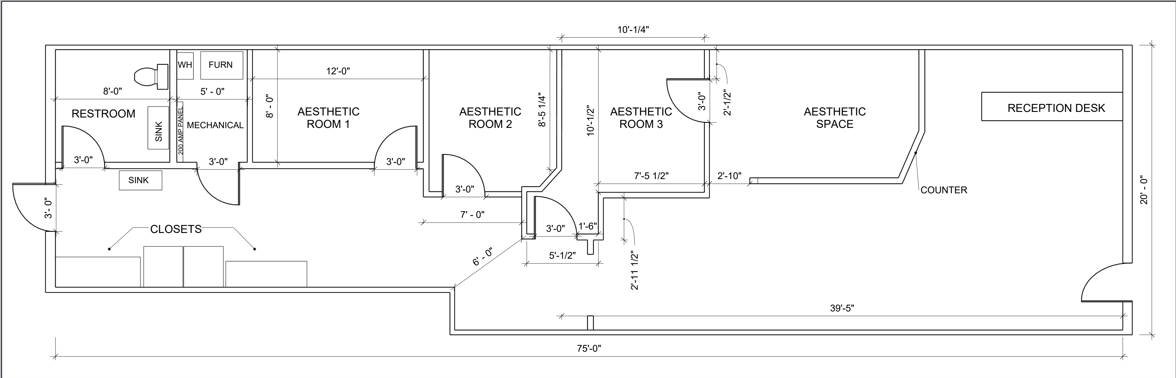
1 FLOOR PLAN Scale: 1/4" : 1'
