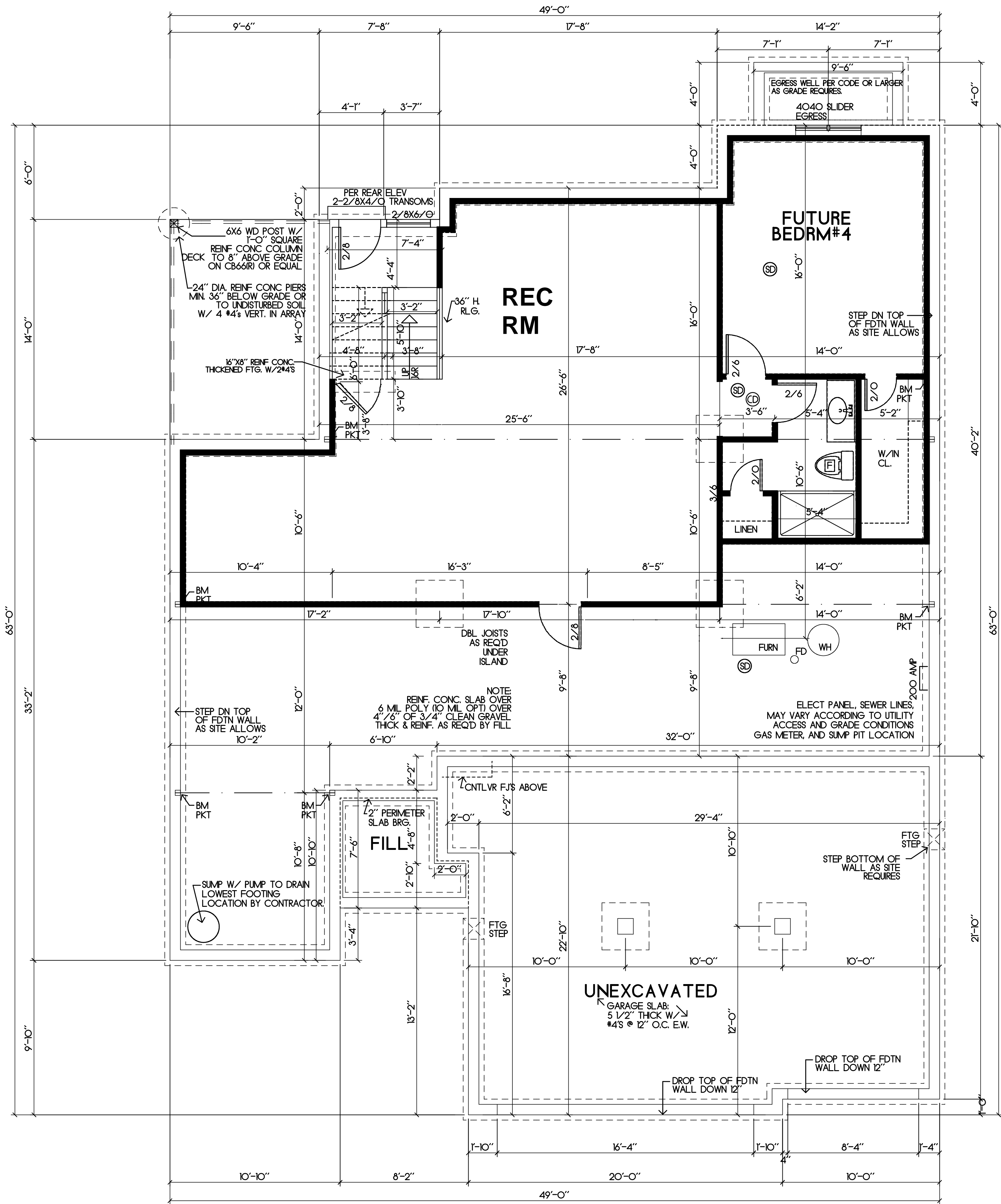
LOWER FLOOR PLAN SCALE: 1/4"=1'-0" AREA: 1020 SF
