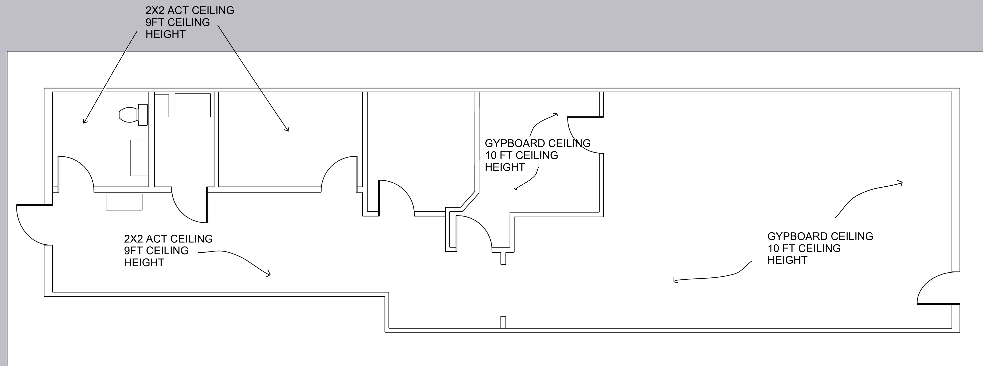
2 FLOOR PLAN REFLECTED CEILING Scale: 1/4" : 1'
