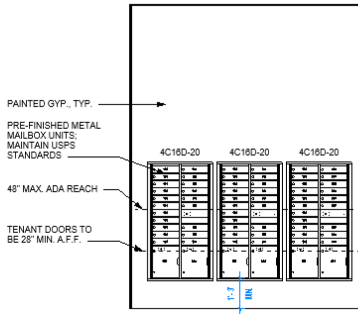
A2 LOBBY MAILBOX ELEVATION \frac{3}{8}" = 1'-0"
