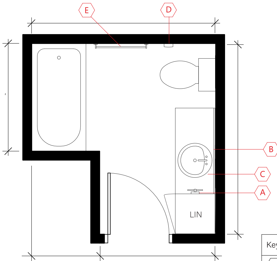
1 BATHROOM ACCESSORY PLAN T2
