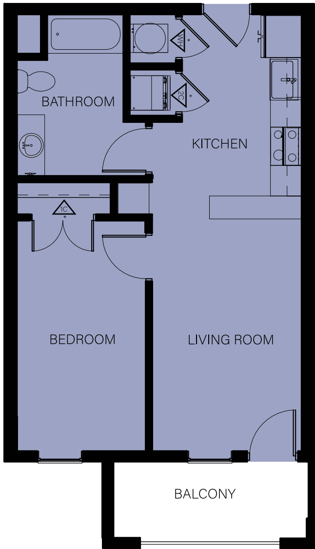
1 S ARA (BALCONY) | STUDIO Unit mirrored for Lot 7
