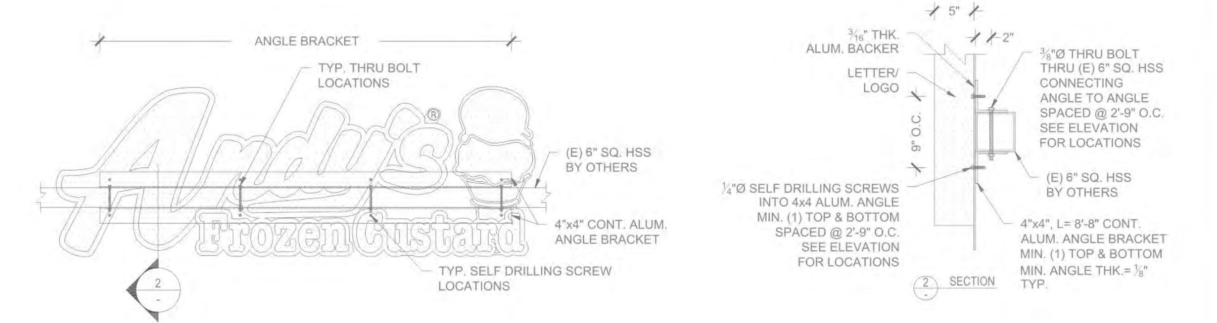
BACK VIEW SCALE: NTS
