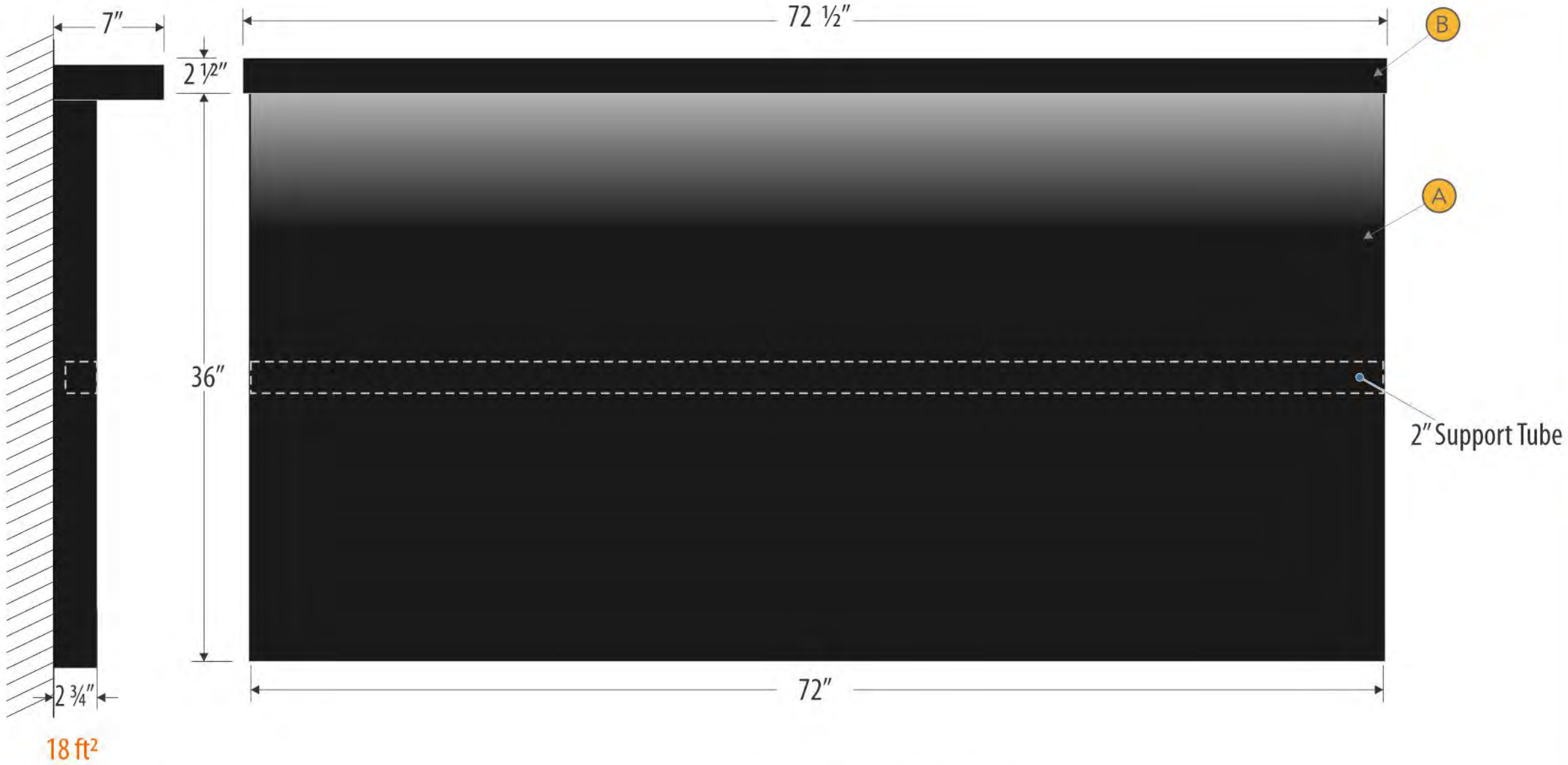
3 Example (Similar) - scale: NTS
