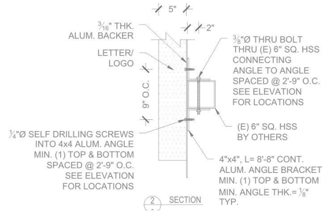
ATTACHMENT VIEW SCALE: NTS
