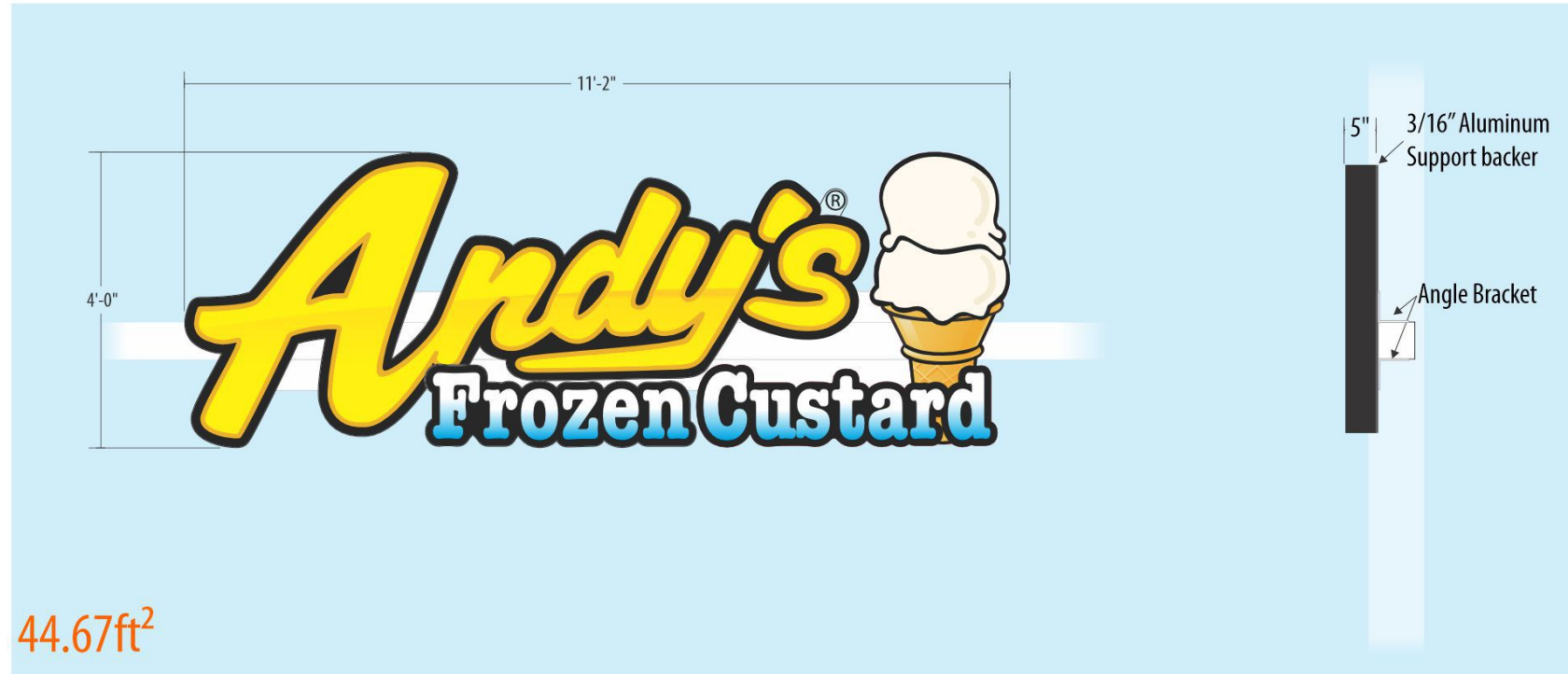
BACK VIEW SCALE: NTS
