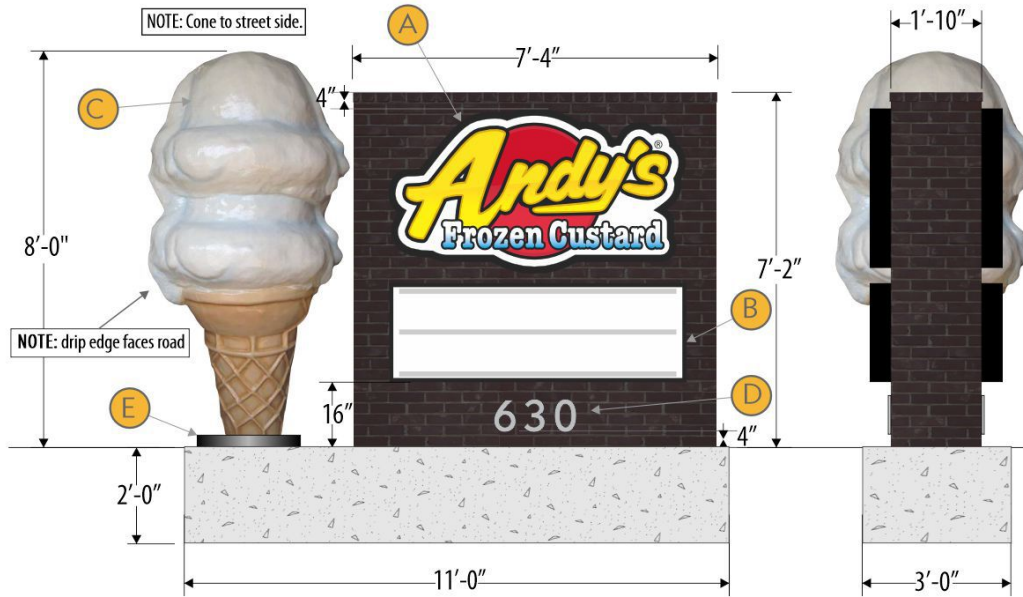
ELEVATION VIEW SCALE: 1/2" = 1'
