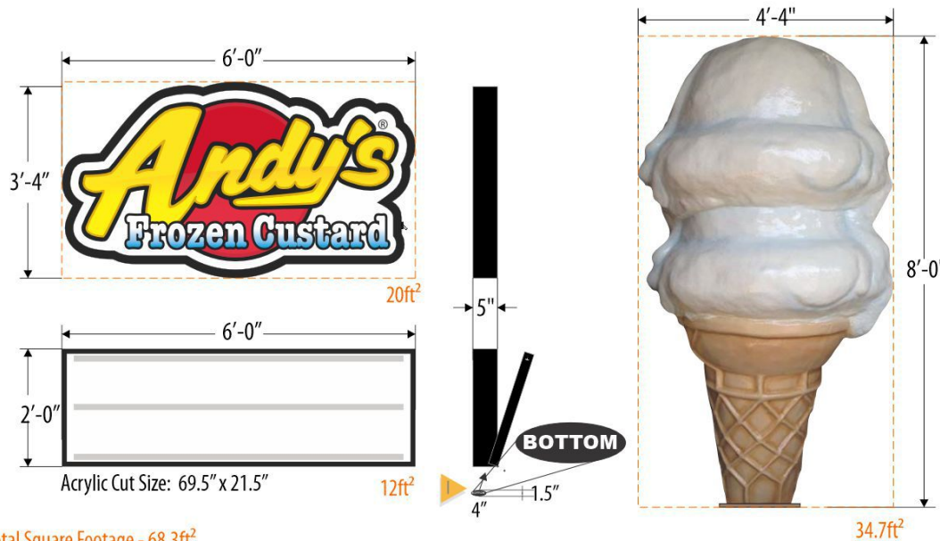
ELEVATION VIEW SCALE: 1/2" = 1'
