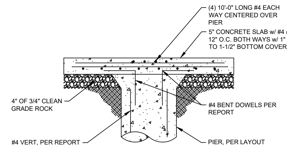
6 S2.1 SLAB SUPPORT PIER DETAIL N.T.S.
