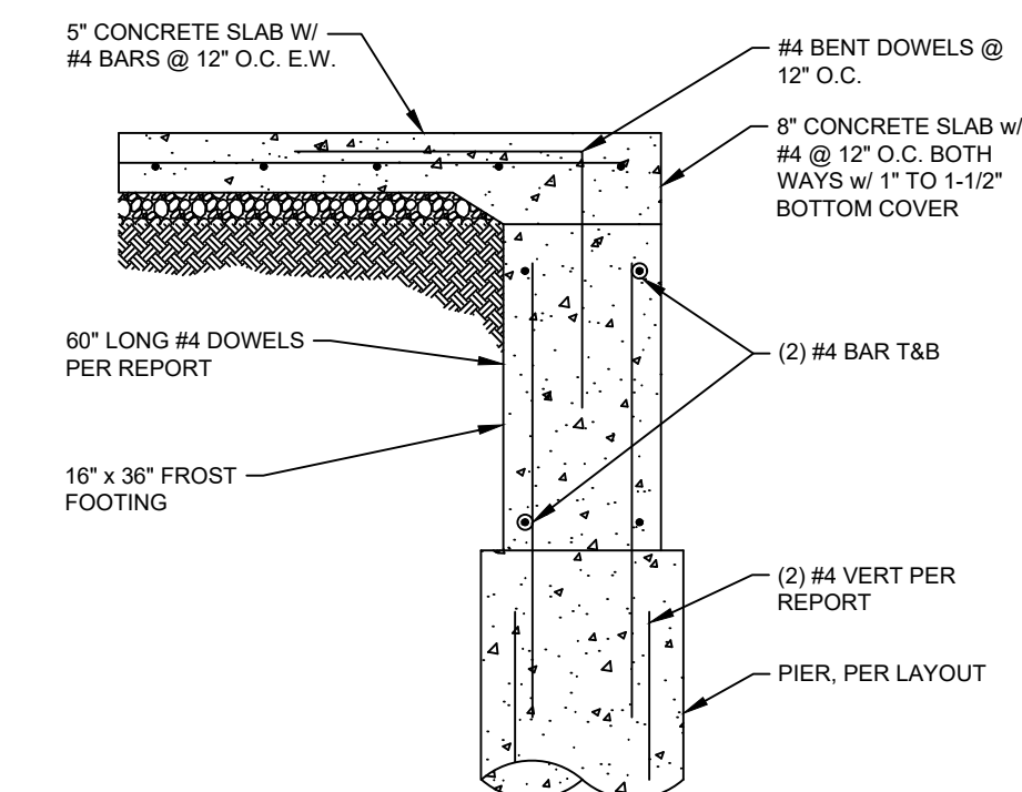
5 S2.1 PIER / FROST FOOTING DETAIL N.T.S.
