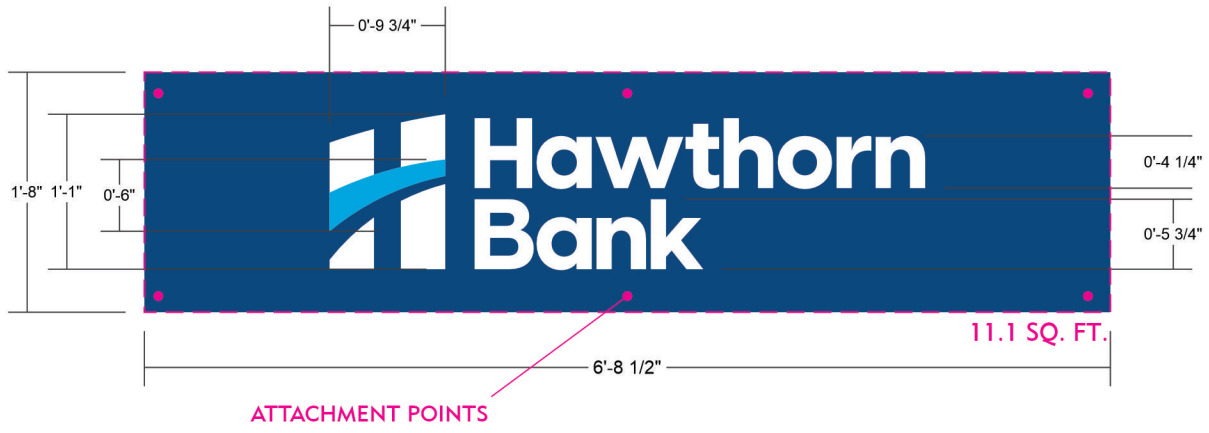
ELEVATION VIEW SCALE: 3/4" = 1'
