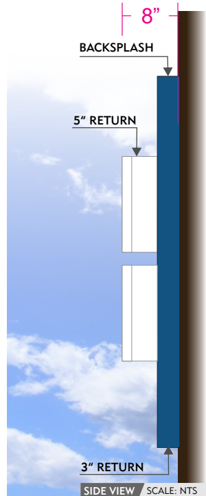
SIDE VIEW SCALE: NTS
