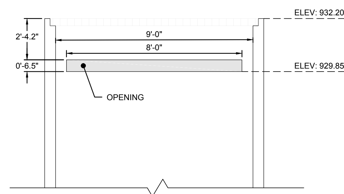
DB2 NE & SW FACES DETAIL NOT TO SCALE
