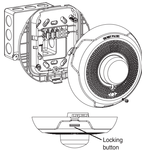
FIGURE 8. MOUNTING
