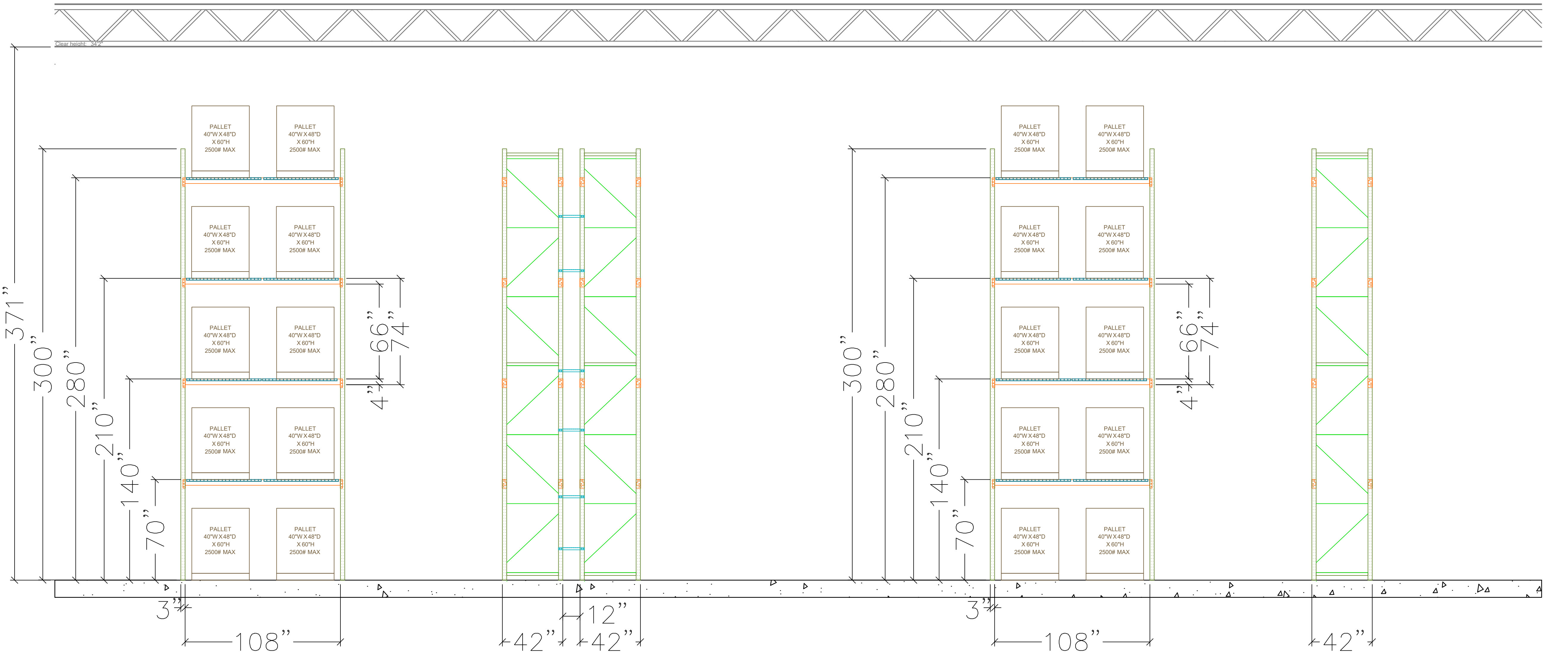
FRONT VIEW "A"
