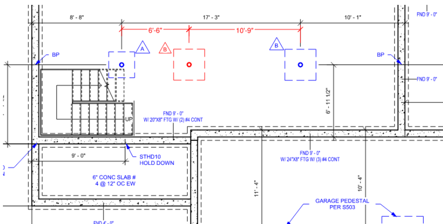
S100 – Foundation Plan
