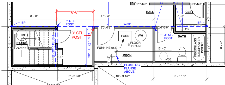
S200 – Lower Level Plan Structural
