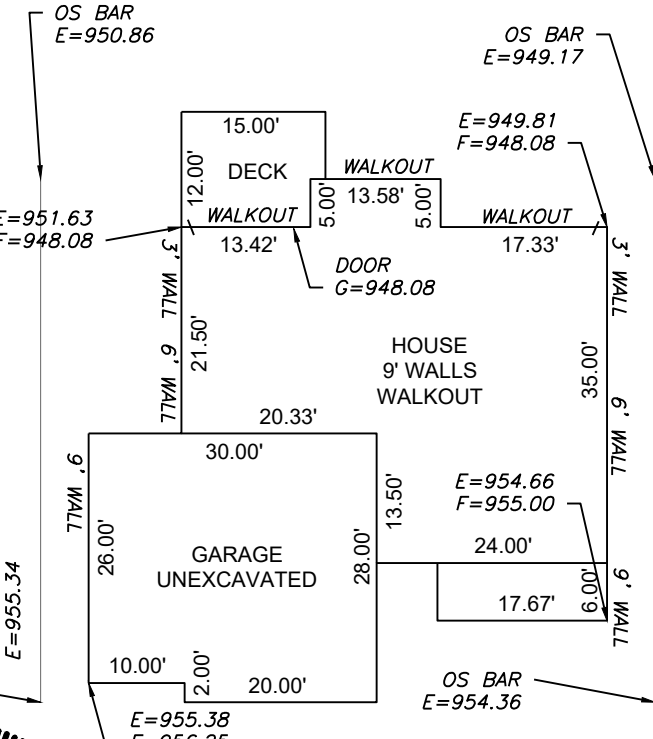
PLAN: THE SILVERTON IV Scale 1"=20'
