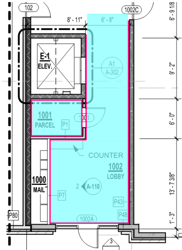
1 ENTRANCE-PACKAGE ROOM | FINISH PLAN MR NOT TO SCALE
