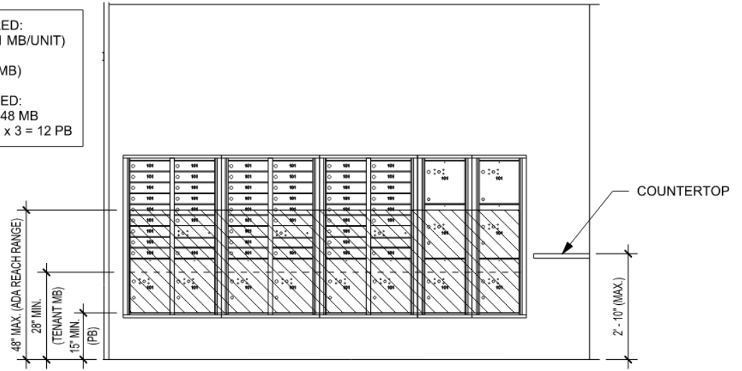
2 MAILBOX | WALL MW NOT TO SCALE
