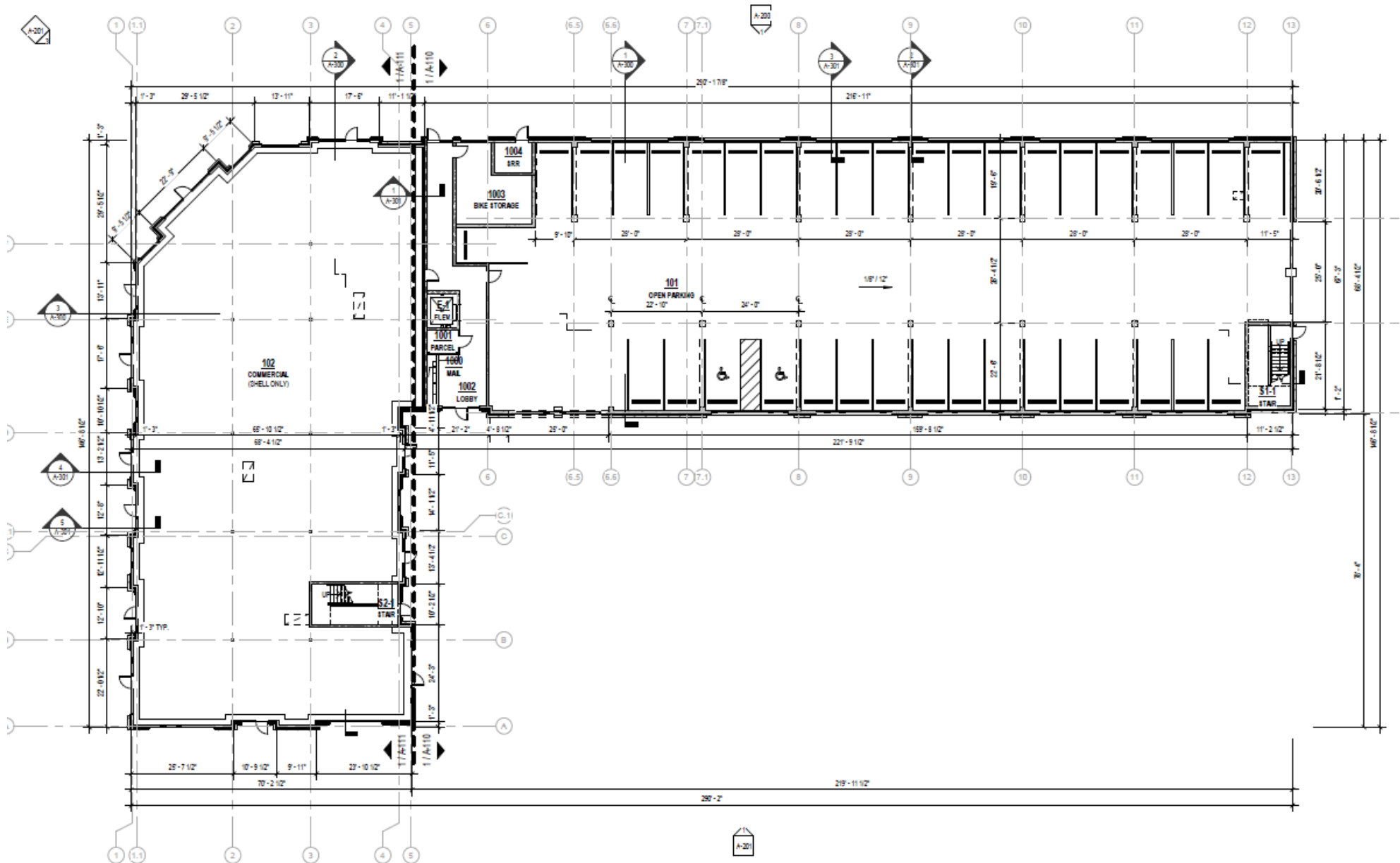
1 L1 LEVEL 1 | FLOOR PLAN NOT TO SCALE
