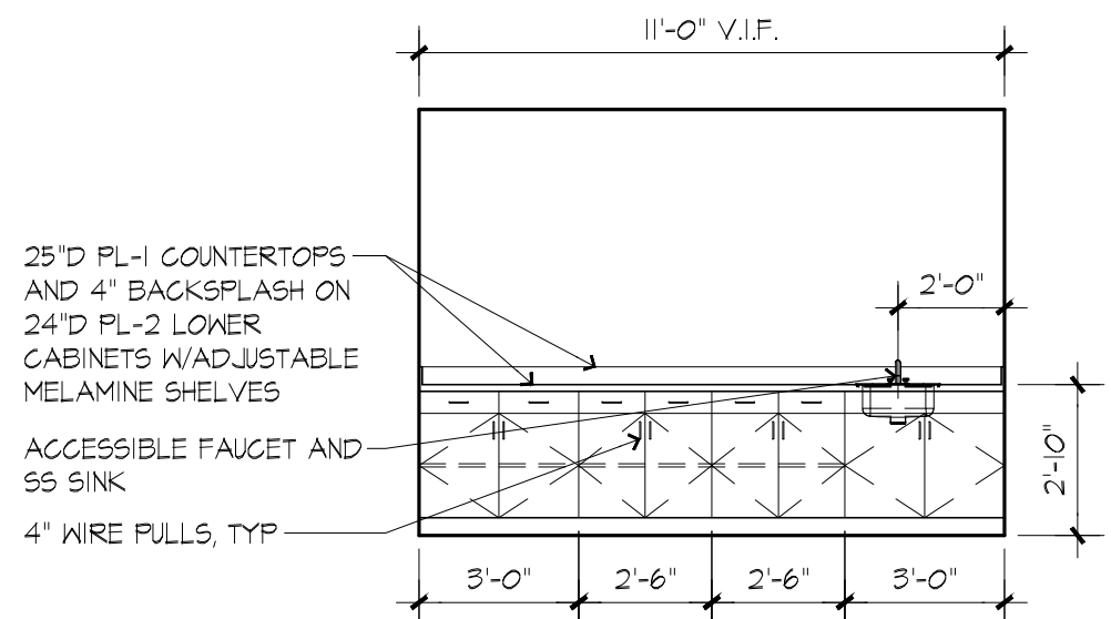
H1 MILLWORK ELEVATION
