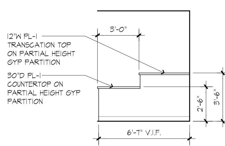
H10 MILLWORK ELEVATION
