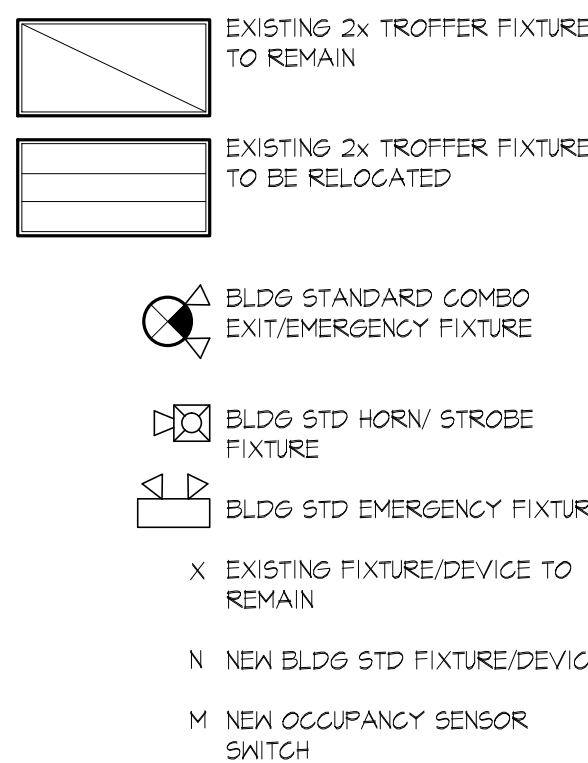
E 14 CEILING LEGEND
