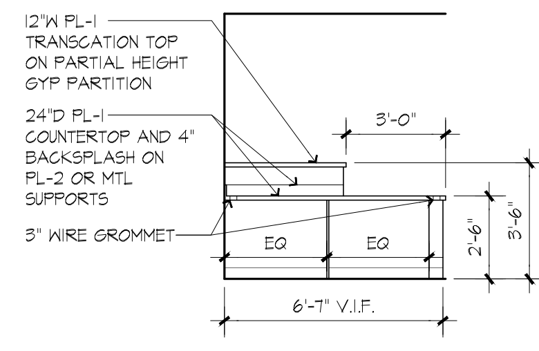
H6 MILLWORK ELEVATION
