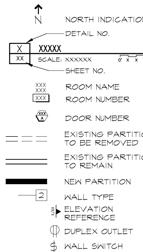
J21 DRAWING LEGEND NO SCALE
