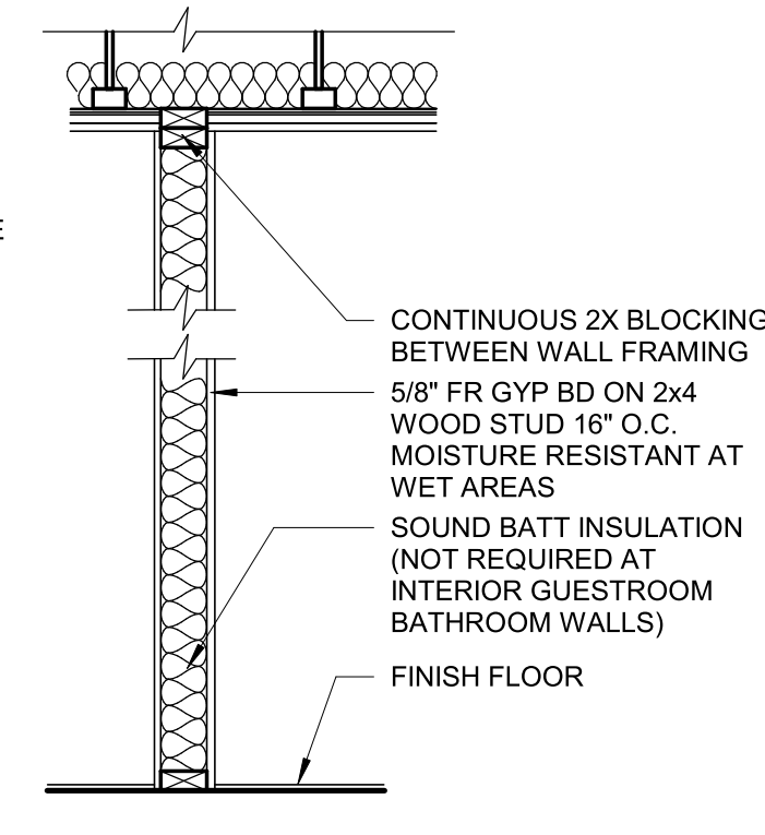
P13 TYP NON BEARING INTERIOR PARTITION WALL NON-RATED
