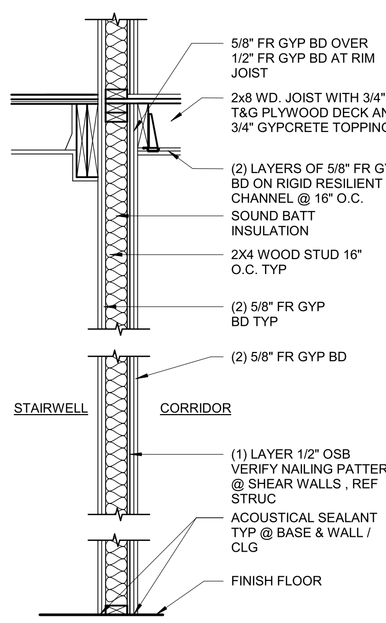
P5 (TYP PARTITION AT STAIRWELL/ CORRIDOR WALL) UL DESIGN #U301 2 HR RATING STC 40 MIN : TEST BASED ON NGC-2363 SEE SHEETS A10.1-A10.2
