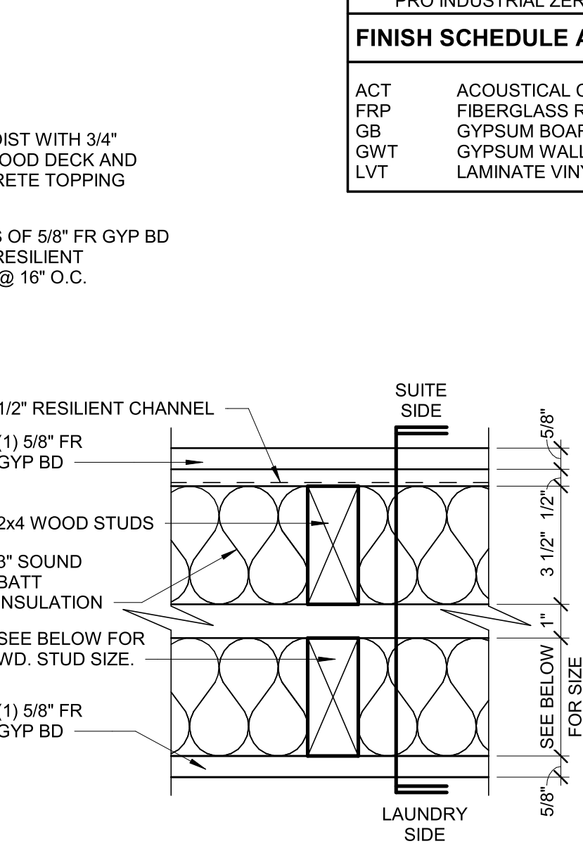
P10 (LAUNDRY /SUITES PARTITION WALL) UL DESIGN #U341 *STAFF LAUNDRY ROOM: 3 1/2" WD STUD WALL *GUEST LAUNDRY ROOM: 5 1/2" WD STUD WALL (COORDINATE FRAMING WITH PLUMBING) SEE SHEET A10.4
