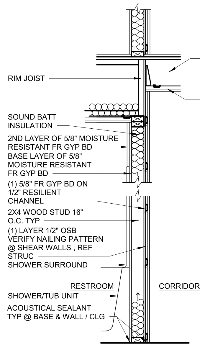
P9 (TYP BATHROOM WALL @ CORRIDOR) UL DESIGN #U327 SEE SHEET A10.3
