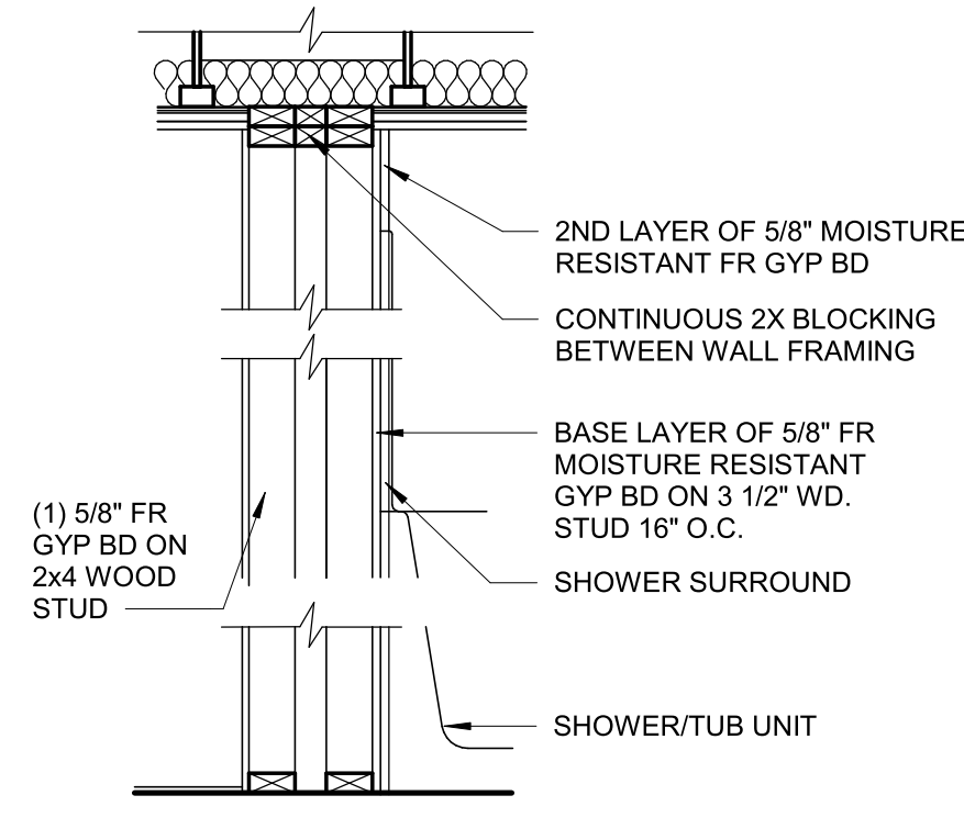
P12 TYP NON BEARING INTERIOR PARTITION WALL AT TUB/SHOWER "BUMP OUT" NON-RATED
