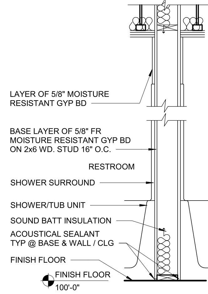
P8 (TYP BATHROOM DEMISING WALL) UL DESIGN #U305 SEE DETAIL A10.3
