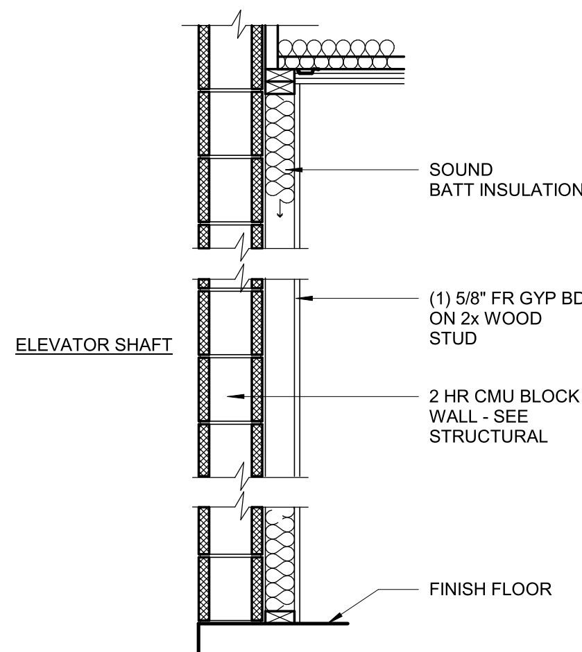
P6 (TYP ELEVATOR /CORRIDOR OR ROOM WALL) UL DESIGN #U905 2 HR RATING SEE SHEET A10.6
