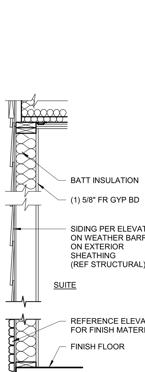
P1 (TYP EXT. WALL) 2x6 WOOD STUD @ 16" O.C. UL DESIGN #U356 SEE SHEET A10.5
