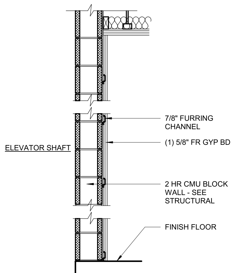
P7 (ELEVATOR/CORRIDOR WALL) UL DESIGN #U905 2 HR RATING SEE SHEET A10.6
