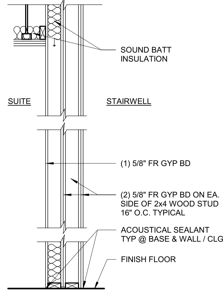
P4 (TYP PARTITION @ STAIRWELL/ CORRIDOR WALL) TYP SUITE SIDE WALL - 2x4 WD STUD UL DESIGN #U301 STC 55 MIN : TEST BASED ON KAISER GYPSUM KG 199 AND GEIGER AND HAMME OC-6FC SEE SHEETS A10.1-A10.2
