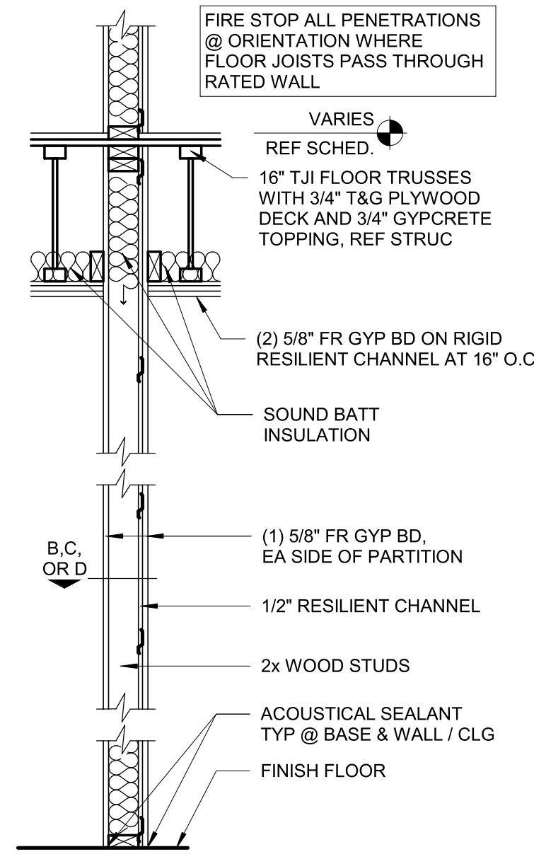
P3 (TYP INTERIOR PARTITION WALL) OMIT RESILIENT CHANNEL AND INSULATION SEE SECTION DETAIL - B UL DESIGN #U305 STC 53 MIN : TEST BASED ON NGC-2009045
