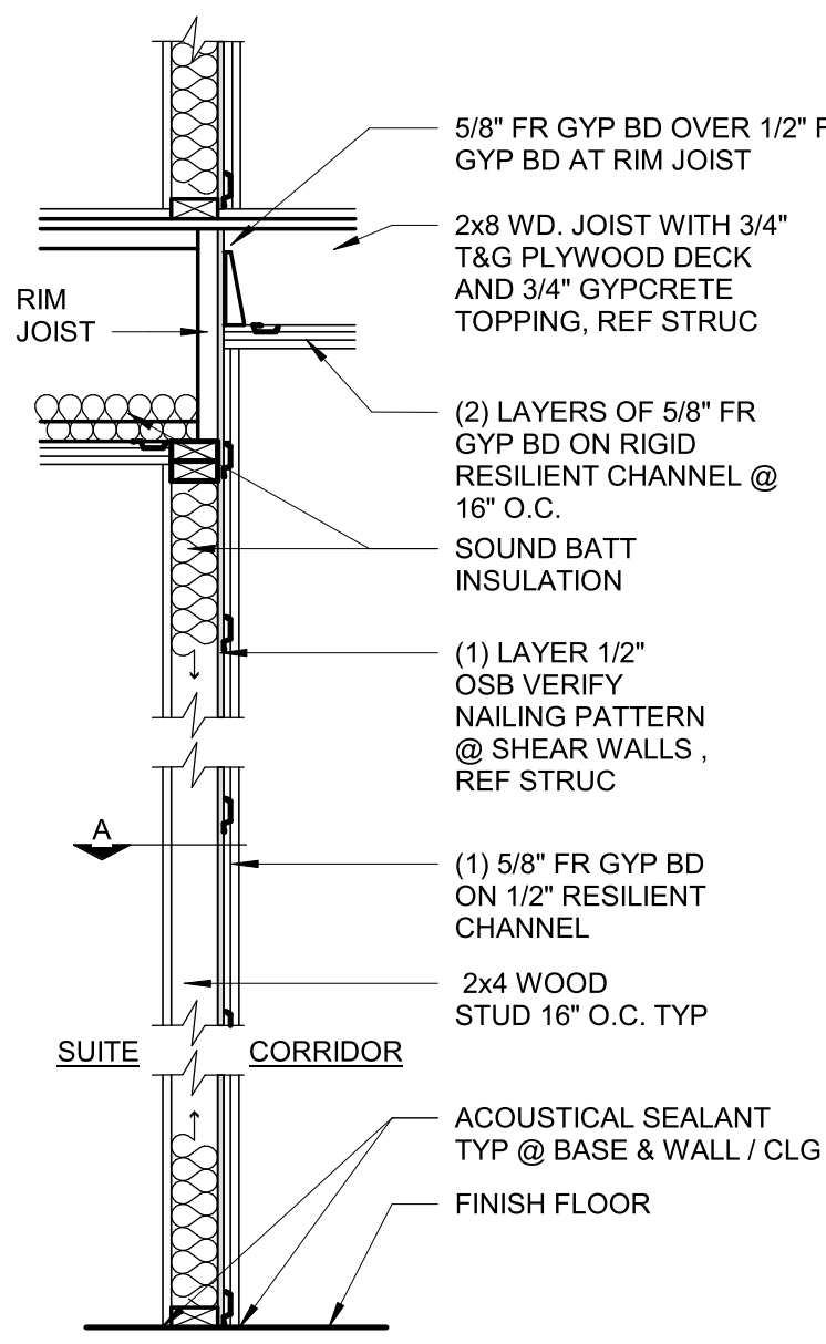
P2 (TYP CORRIDOR WALL) UL DESIGN #U327 SEE SHEET A10.3
