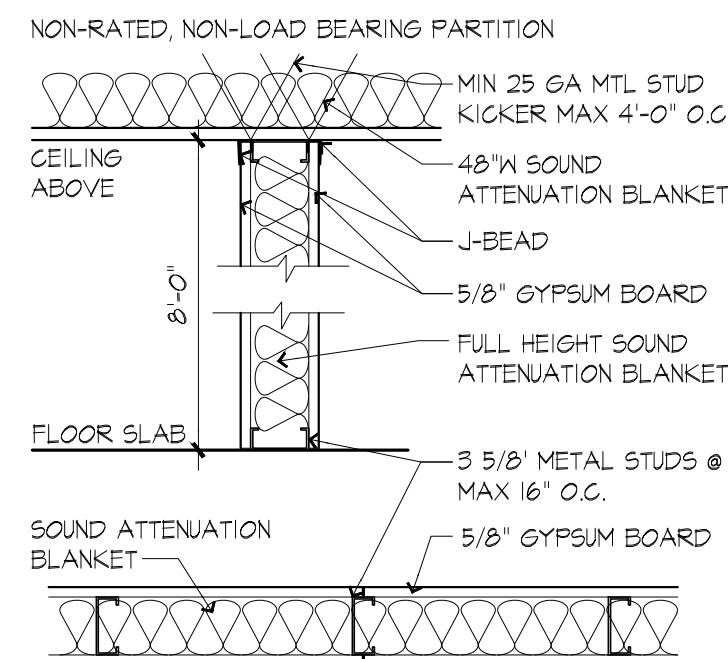
DESCRIPTION 3 5/8" MIN 25 GA. MTL STUDS TO UNDERSIDE OF SUSPENDED CEILING GRID, 16" O.C. BRACE TO STRUCTURE. FOUR FOOT WIDE, 5/8" GYPSUM BOARD BOTH SIDES OF STUDS. FULL THICKNESS, FULL HEIGHT SOUND ATTENUATION IN STUD CAVITY. 48"X SOUND ATTENUATION ON CEILING CENTERED ON PARTITION. SEAL ALL OPENINGS.
