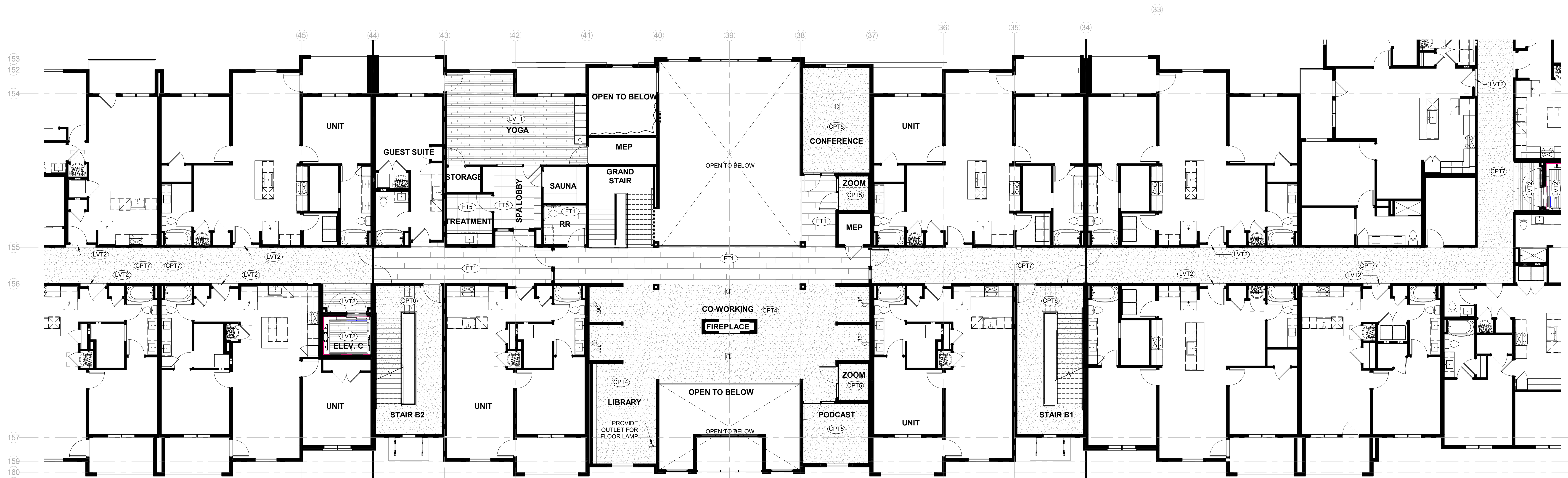
2 Level 2 - Flooring Plan 1/8" = 1'-0"
