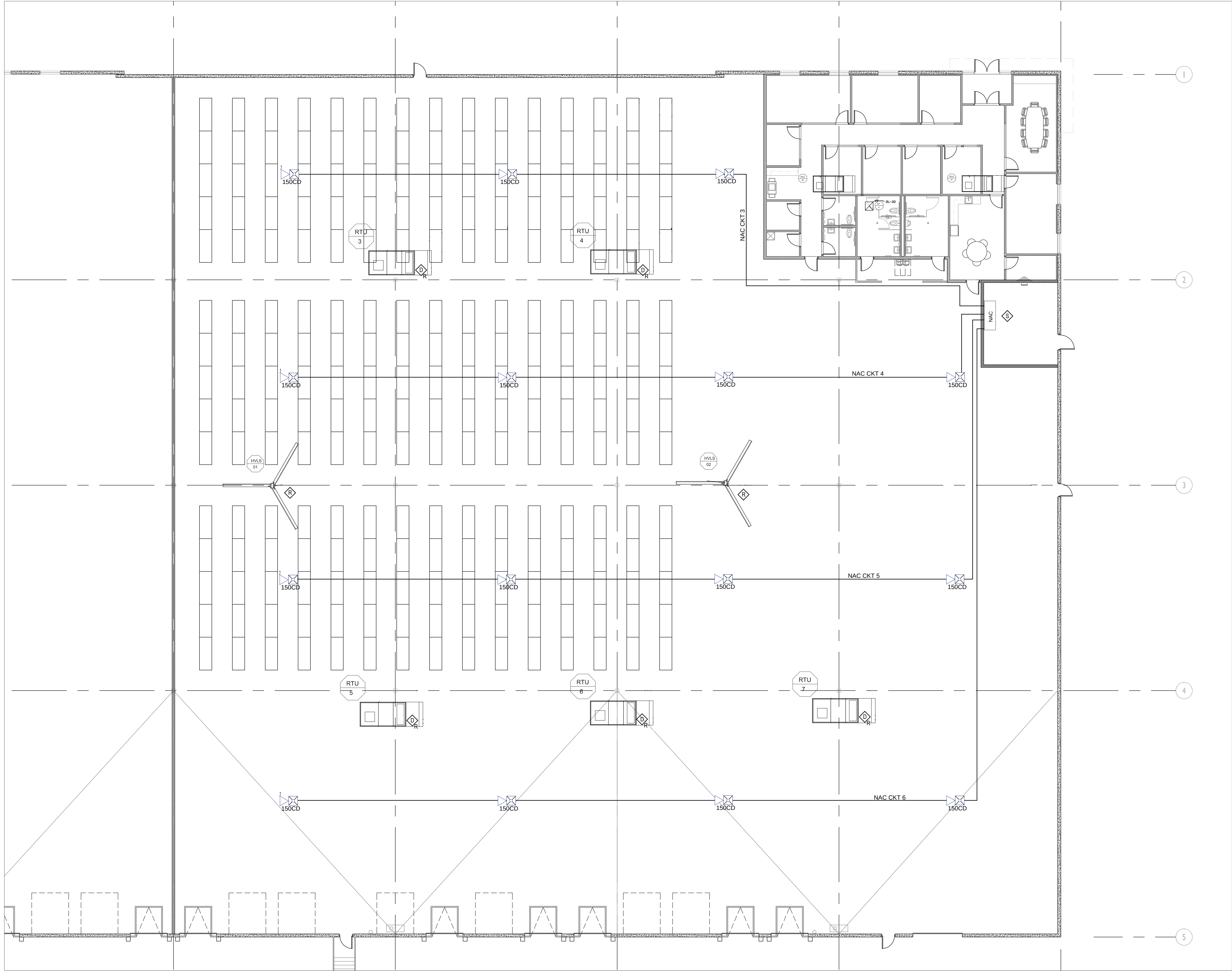
1 WAREHOUSE FIRE ALARM LAYOUT 3/32" = 1'
