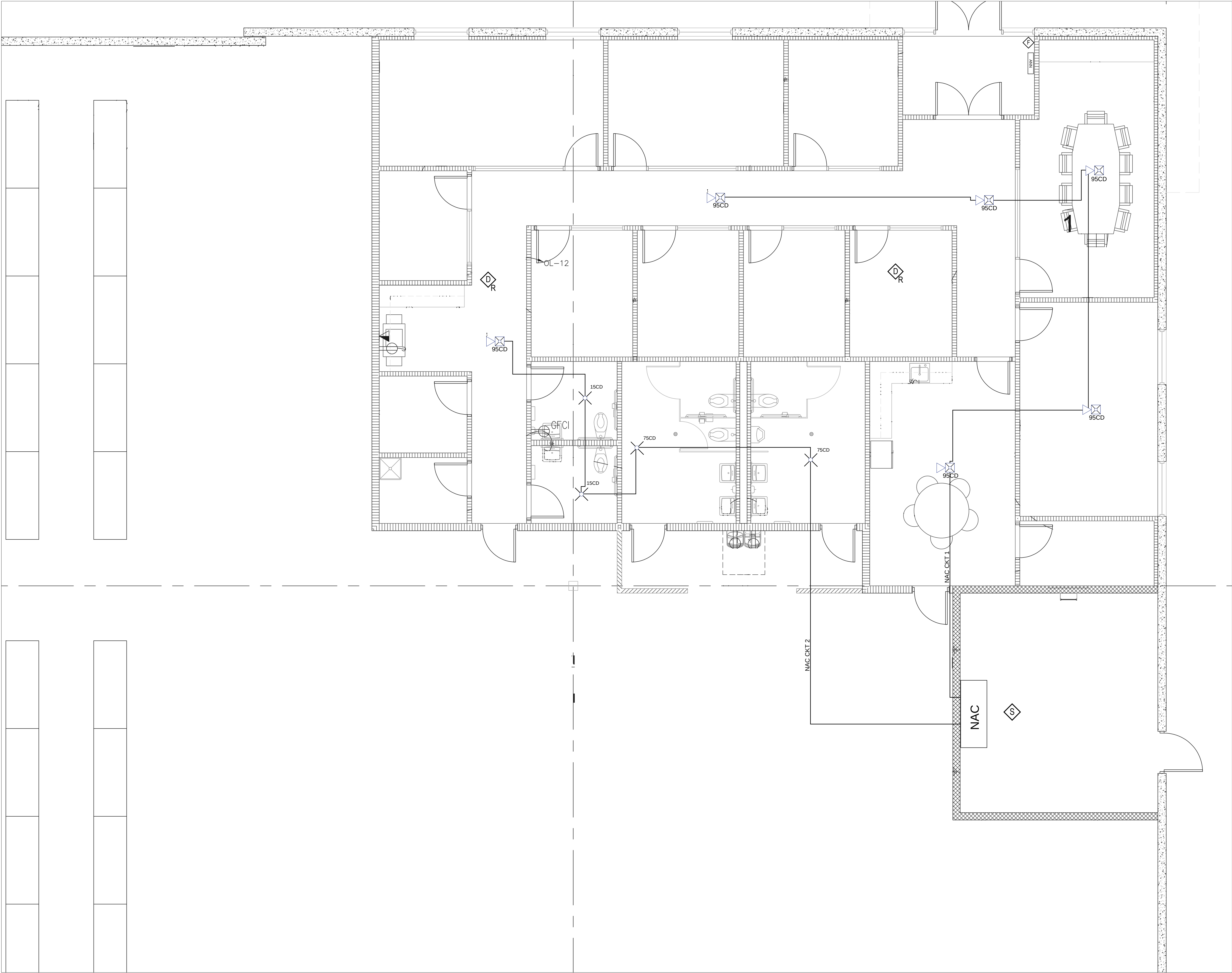
1 OFFICE FIRE ALARM LAYOUT 1/4" = 1'
