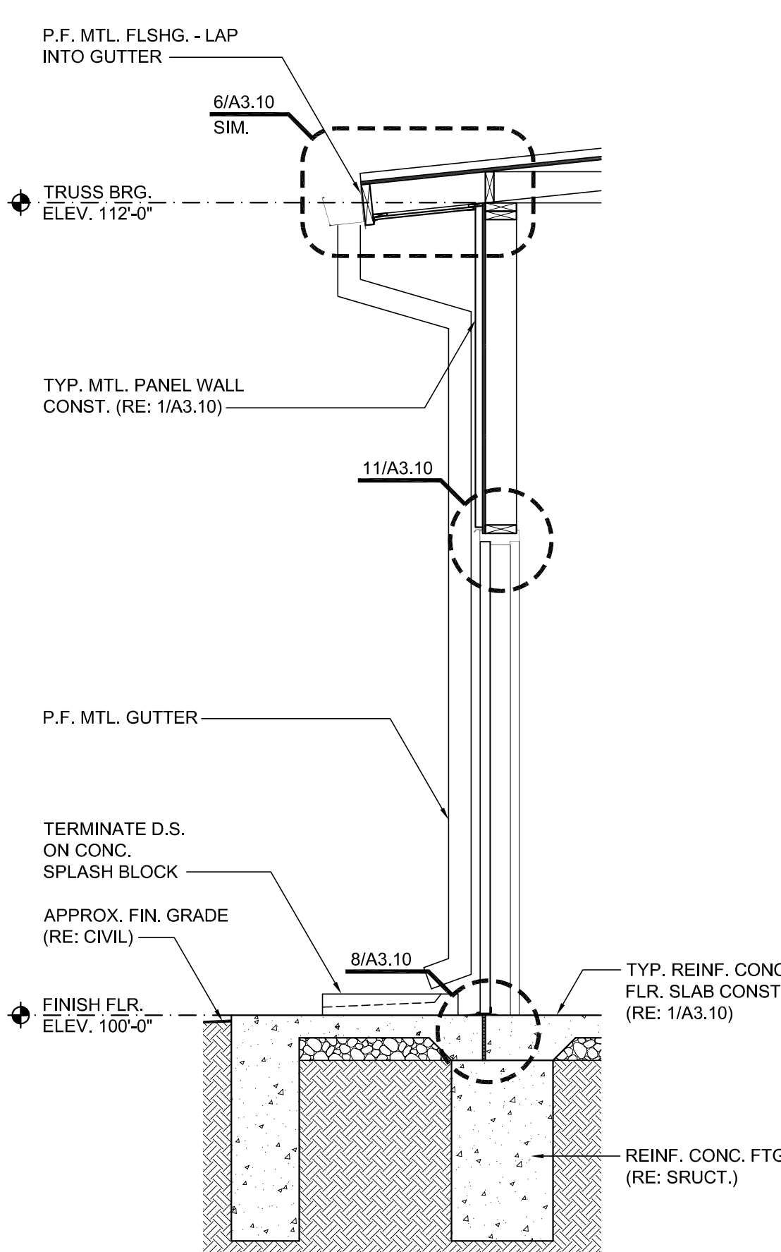
3 WALL SECTION 1/2"=1'-0"
