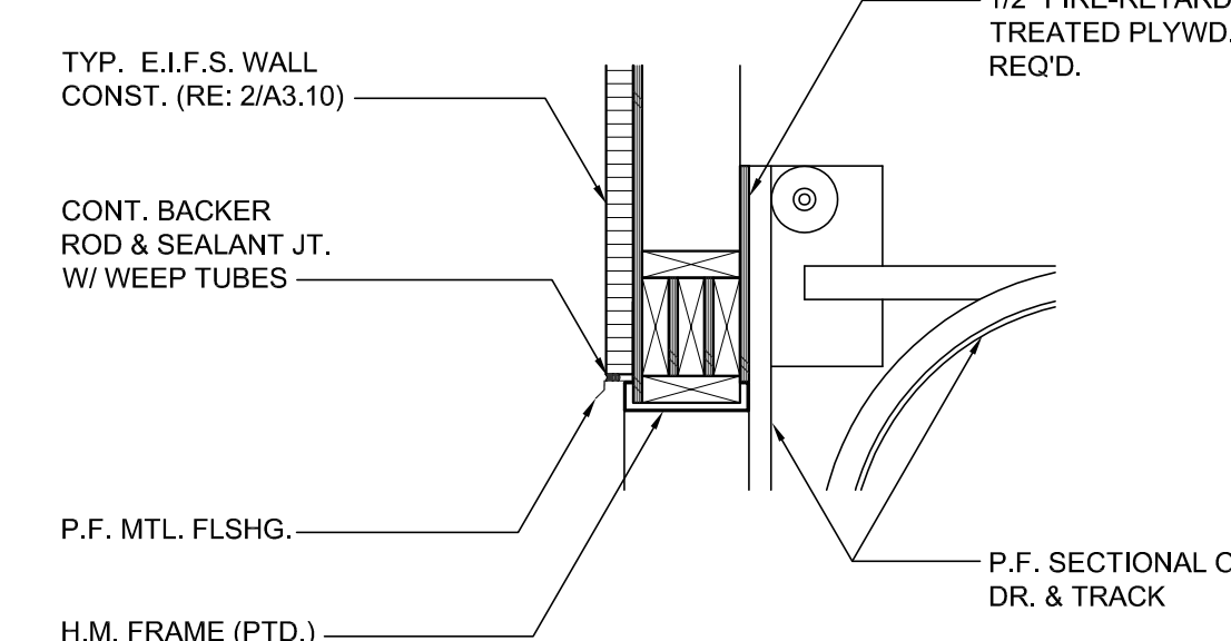
9 HEAD DETAIL 1" = 1'-0"
