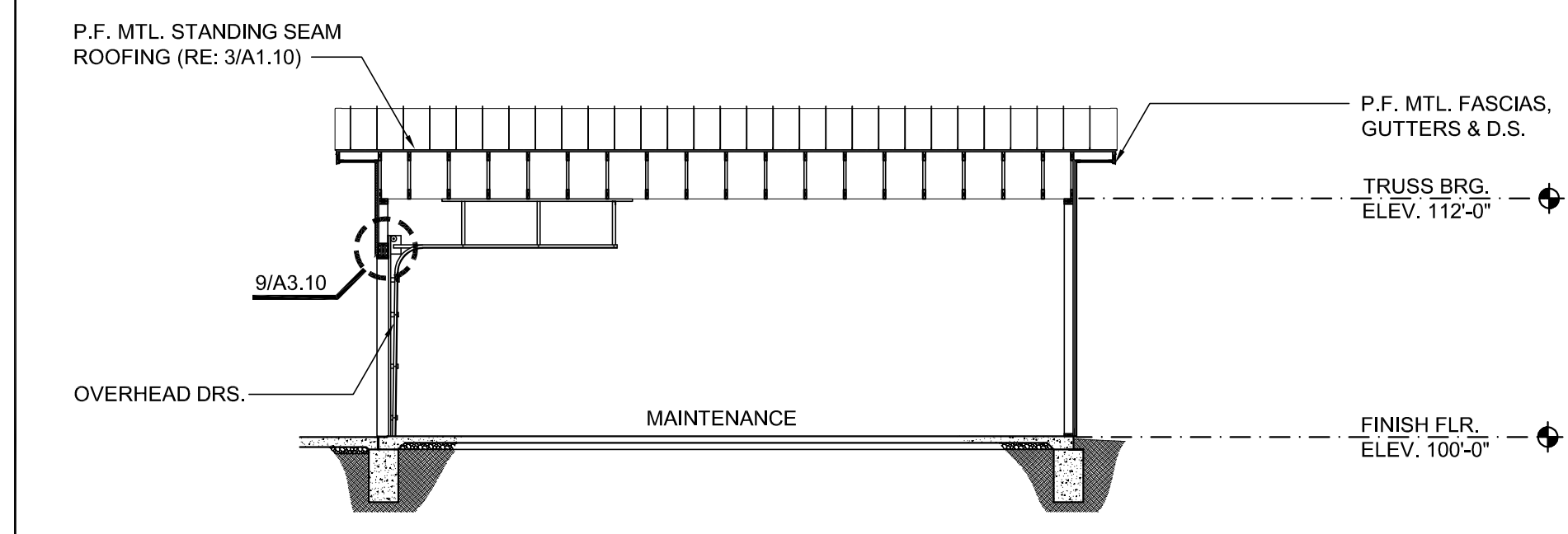
6 BUILDING SECTION A2.10 1/8"=1'-0"
