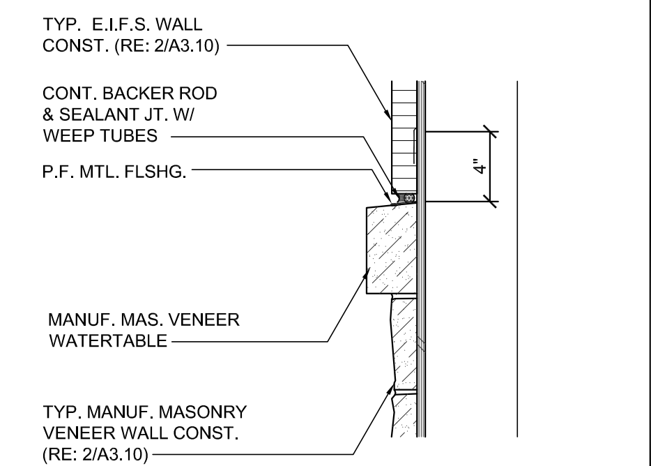
5 DETAIL 1 1/2" = 1'-0"
