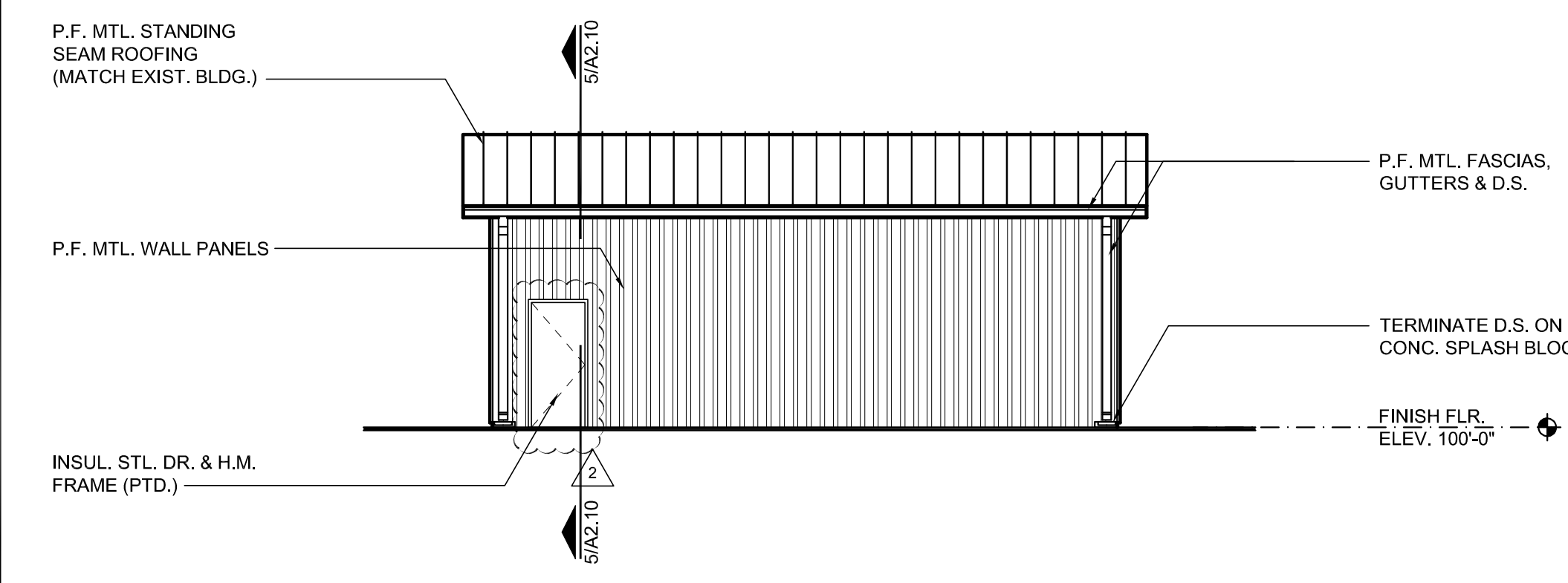
2 SOUTH ELEVATION A2.10 1/8"=1'-0"
