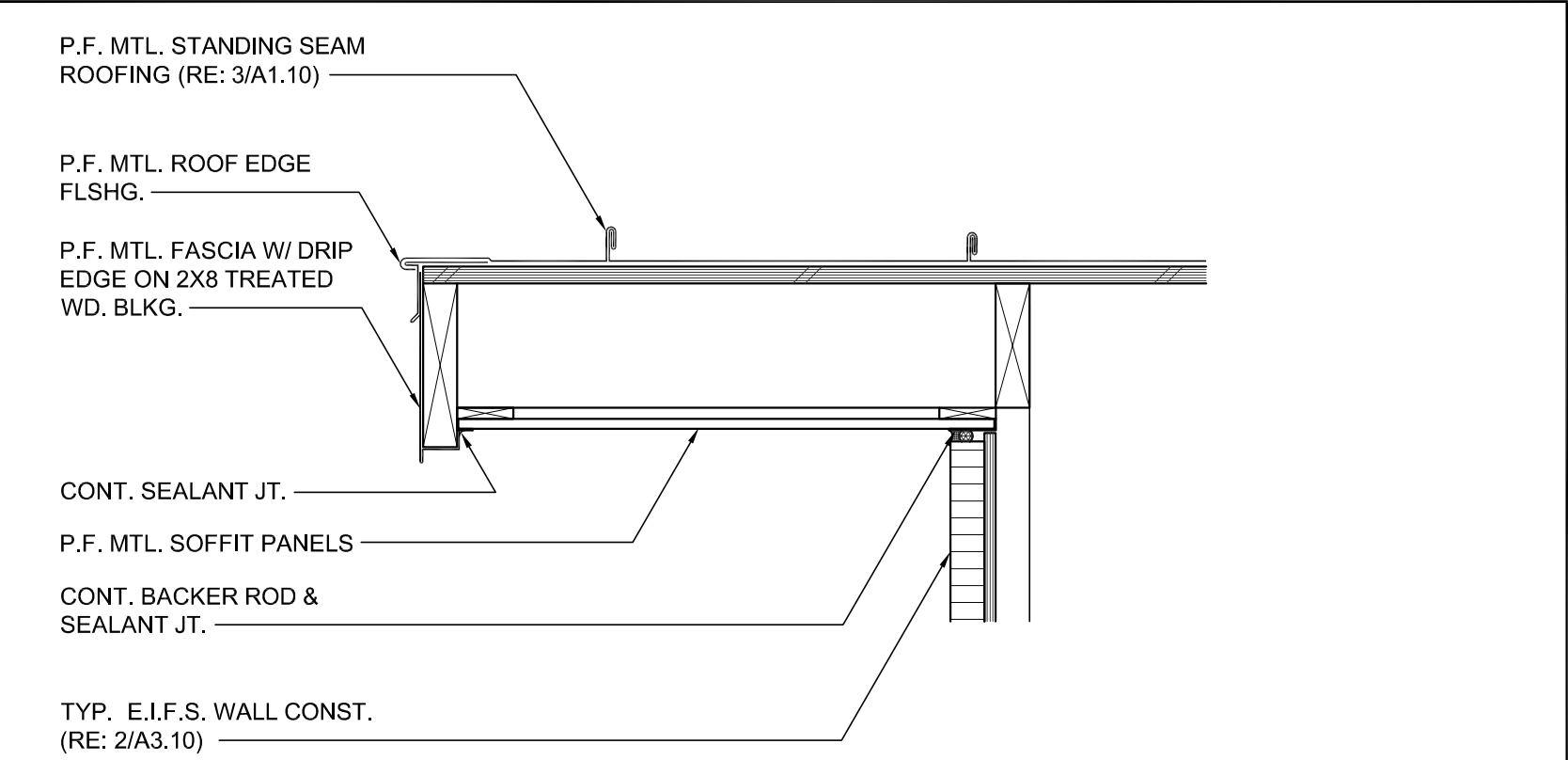
6 DETAIL 1 1/2" = 1'-0"
