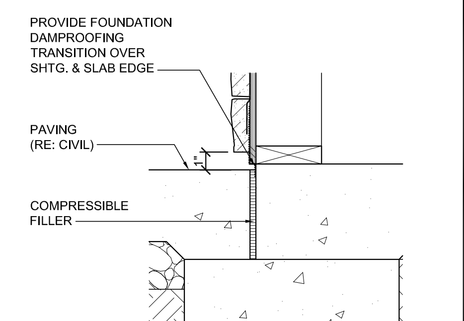
4 DETAIL 1 1/2" = 1'-0"
