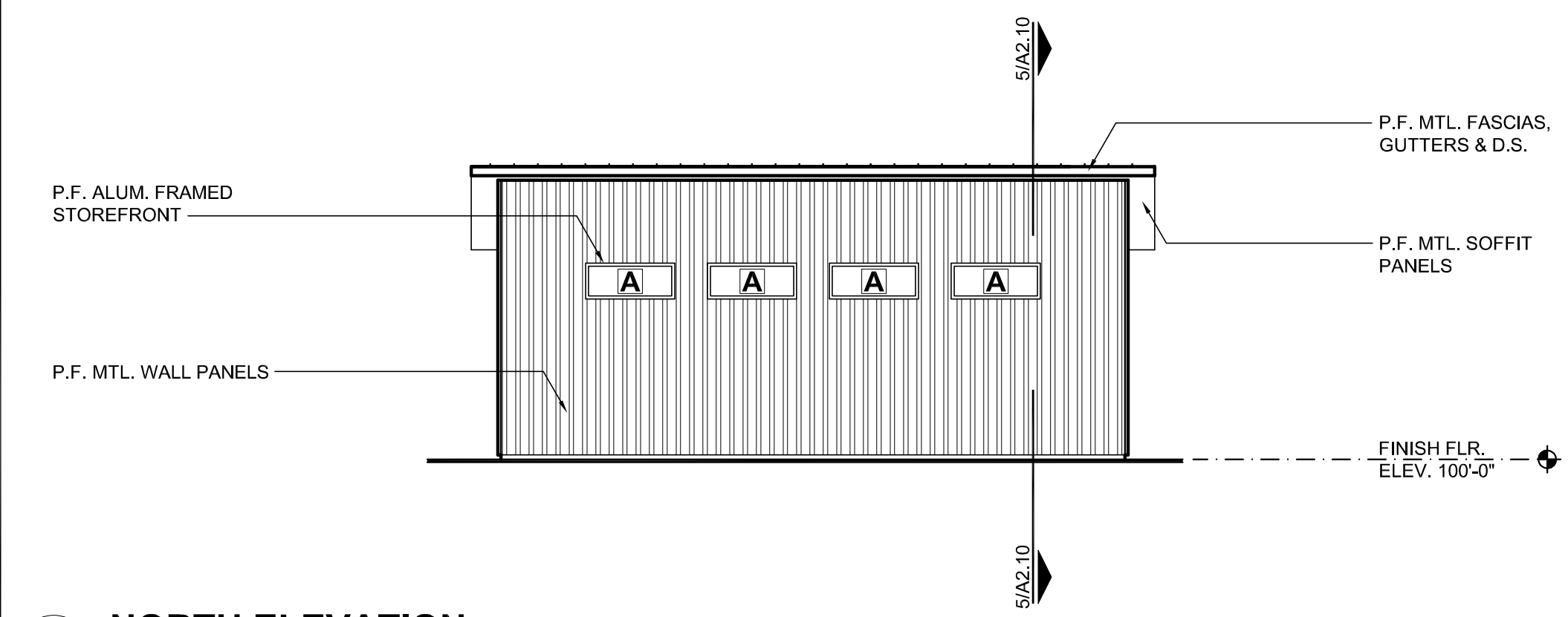
4 NORTH ELEVATION A2.10 1/8"=1'-0"
