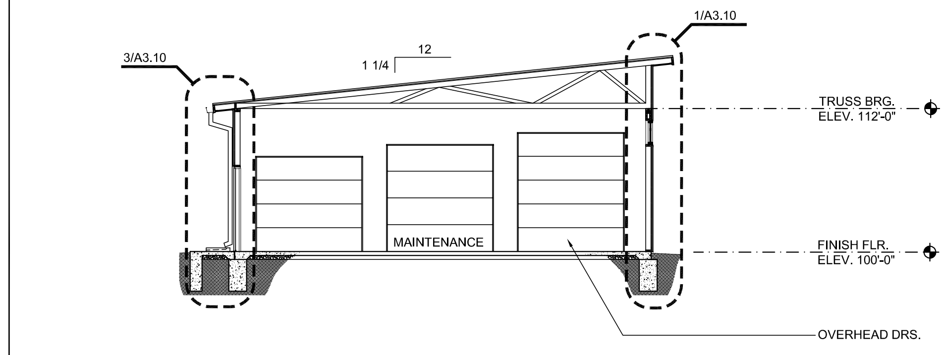
5 BUILDING SECTION A2.10 1/8"=1'-0"
