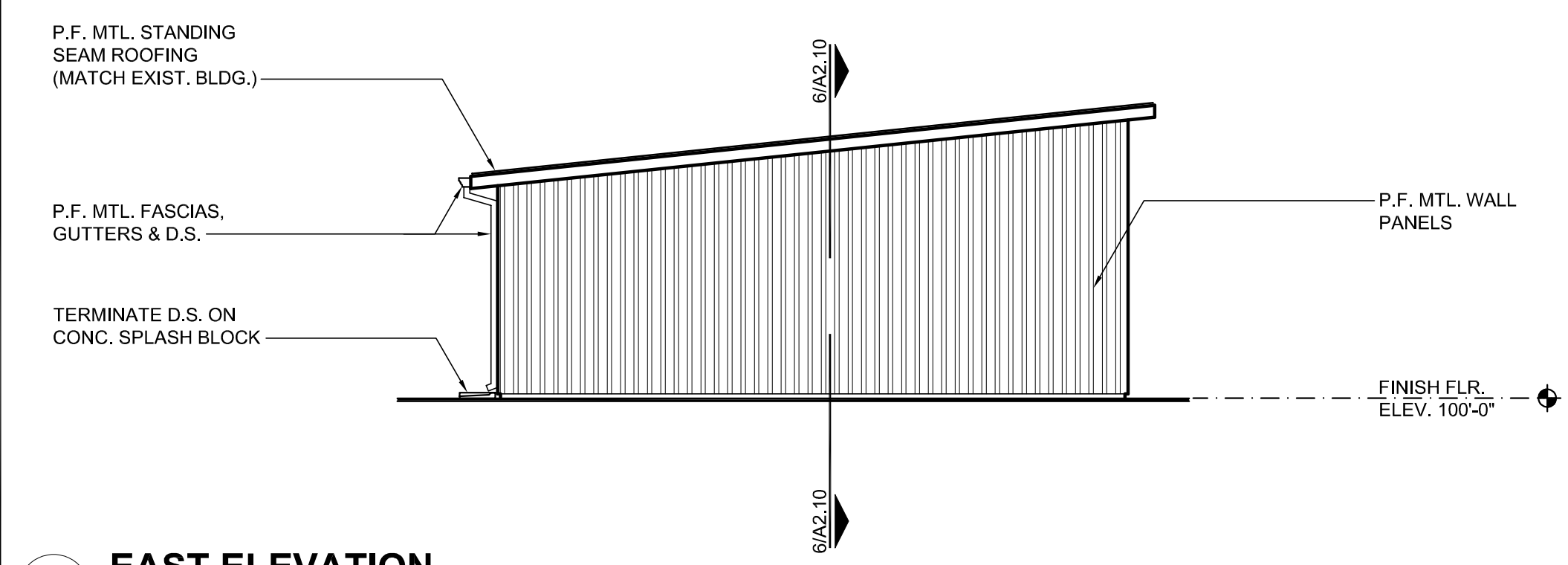
3 EAST ELEVATION A2.10 1/8"=1'-0"
