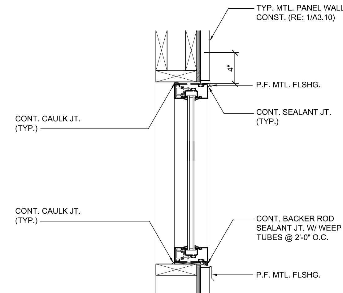
12 DETAIL 1 1/2" = 1'-0"
