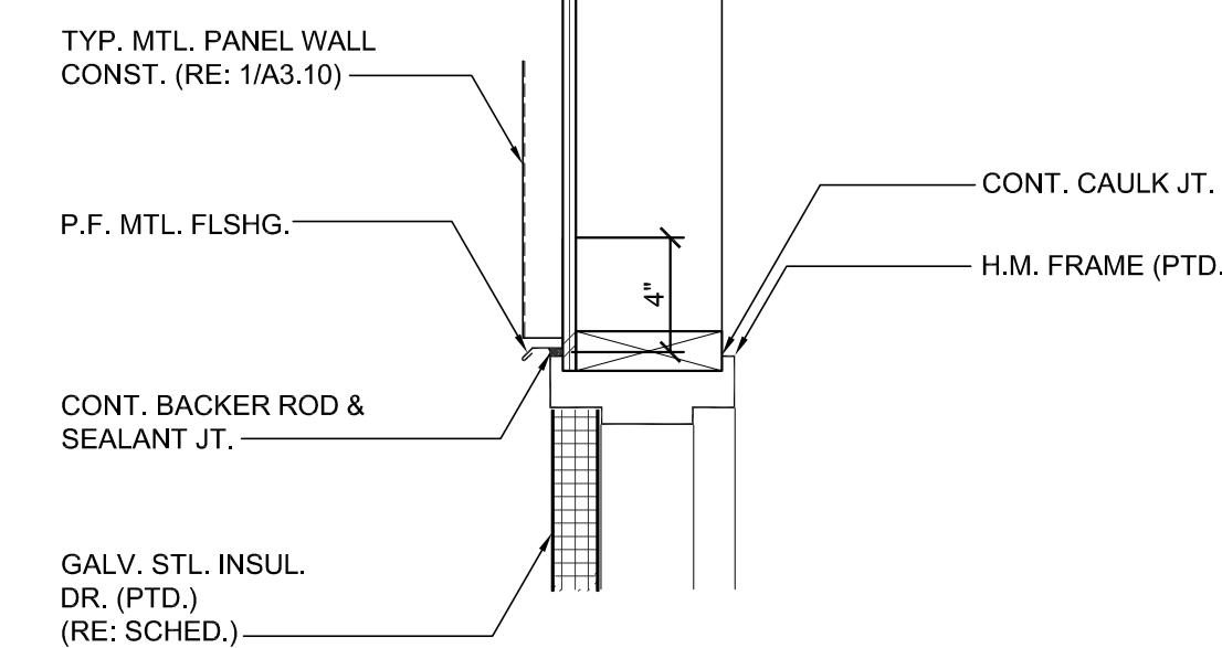
11 HEAD DETAIL 1 1/2" = 1'-0"
