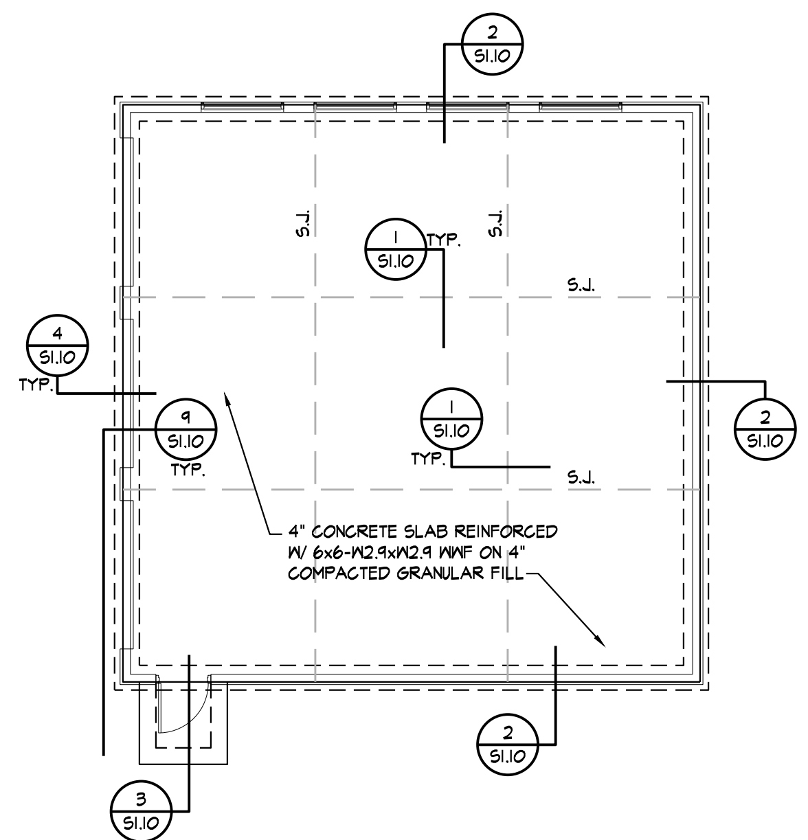
FOUNDATION PLAN 1/8" = 1'-0"
