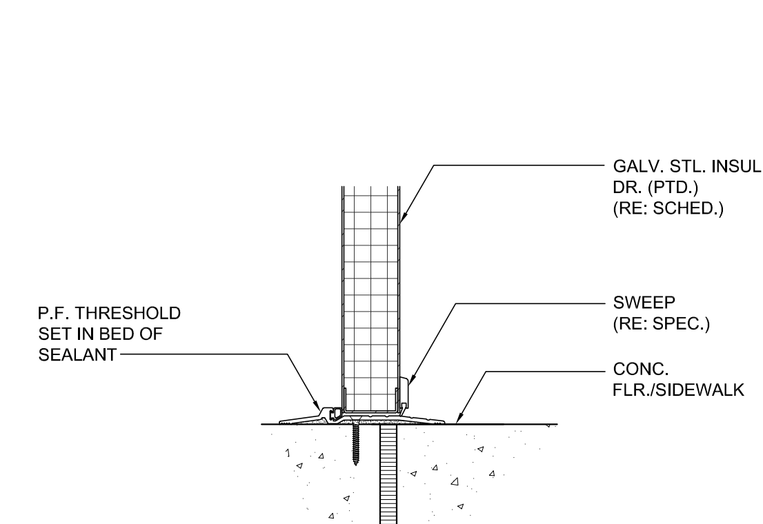
8 DETAIL 3" = 1'-0"
