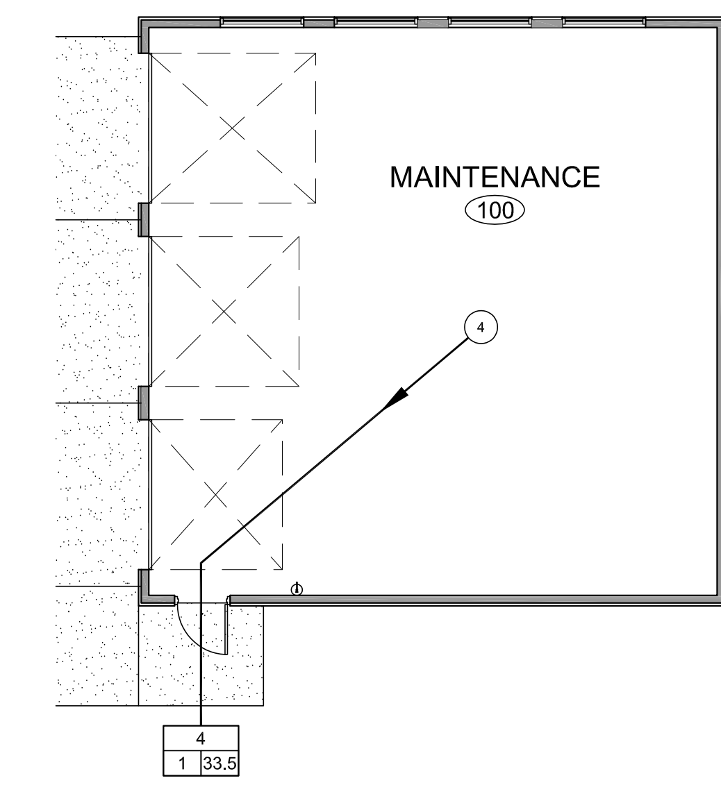
EGRESS PLAN 1/8"=1'-0"
