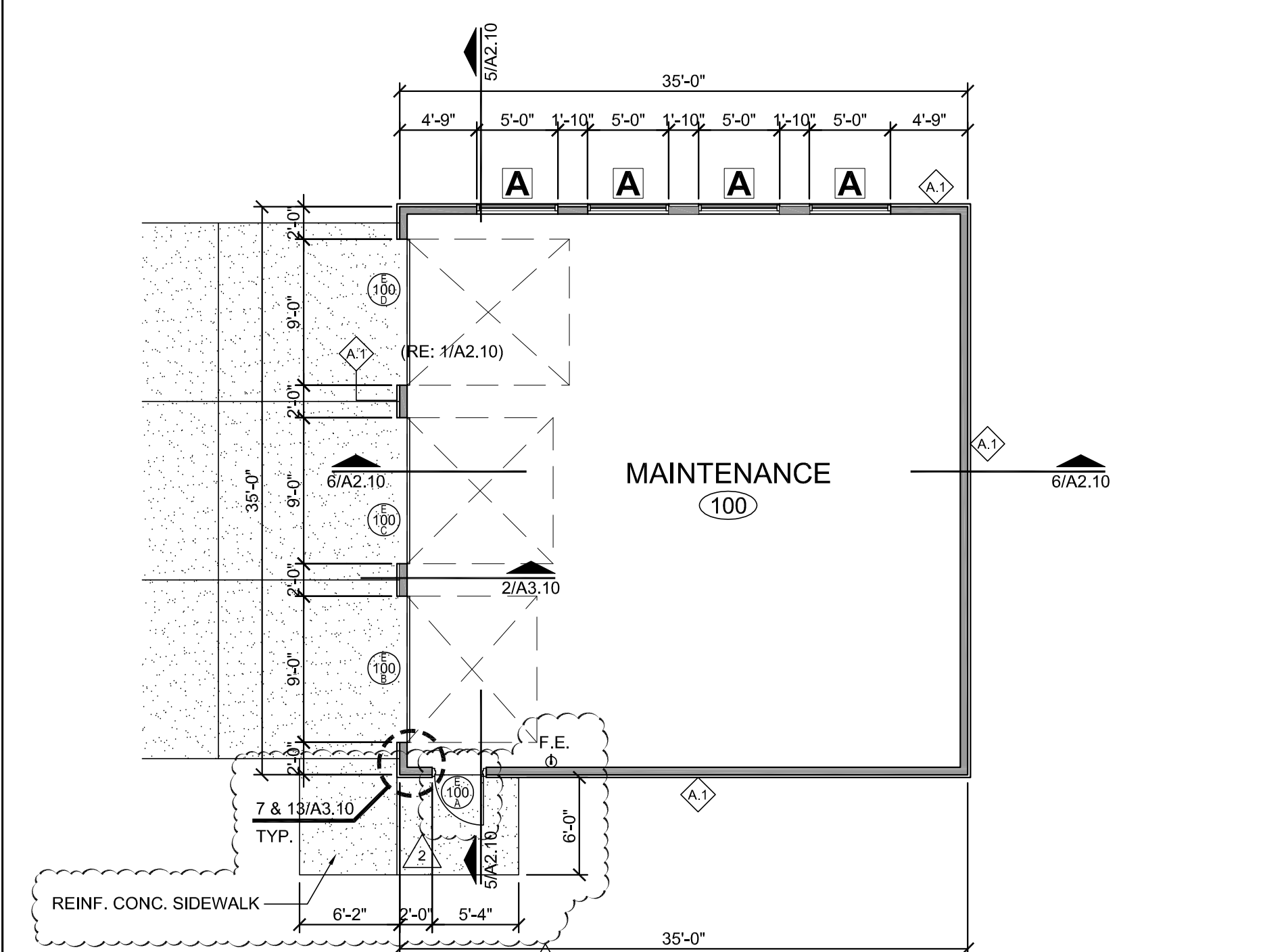
FLOOR PLAN 1/8"=1'-0"
