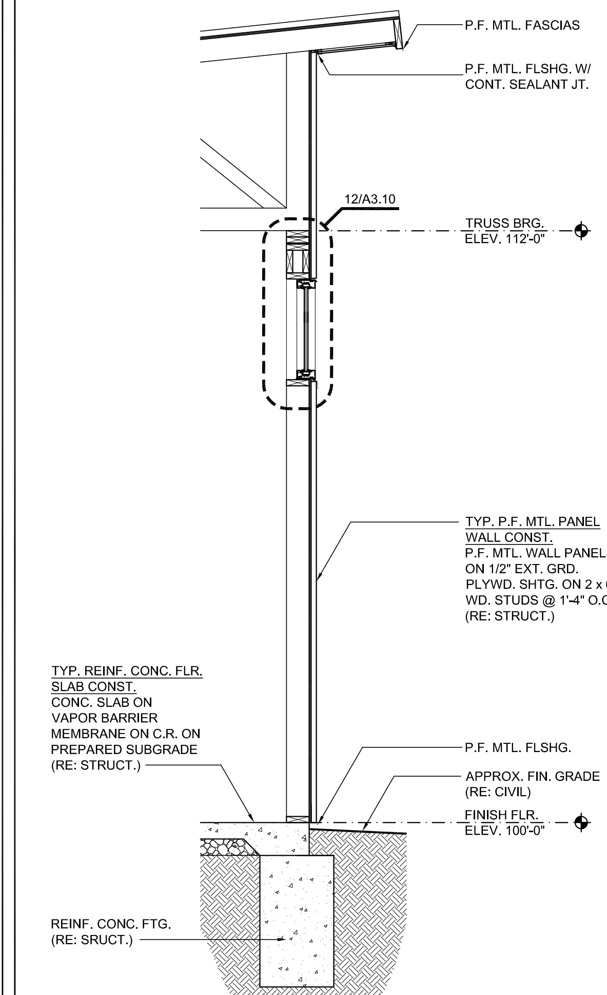
1 WALL SECTION 1/2"=1'-0"
