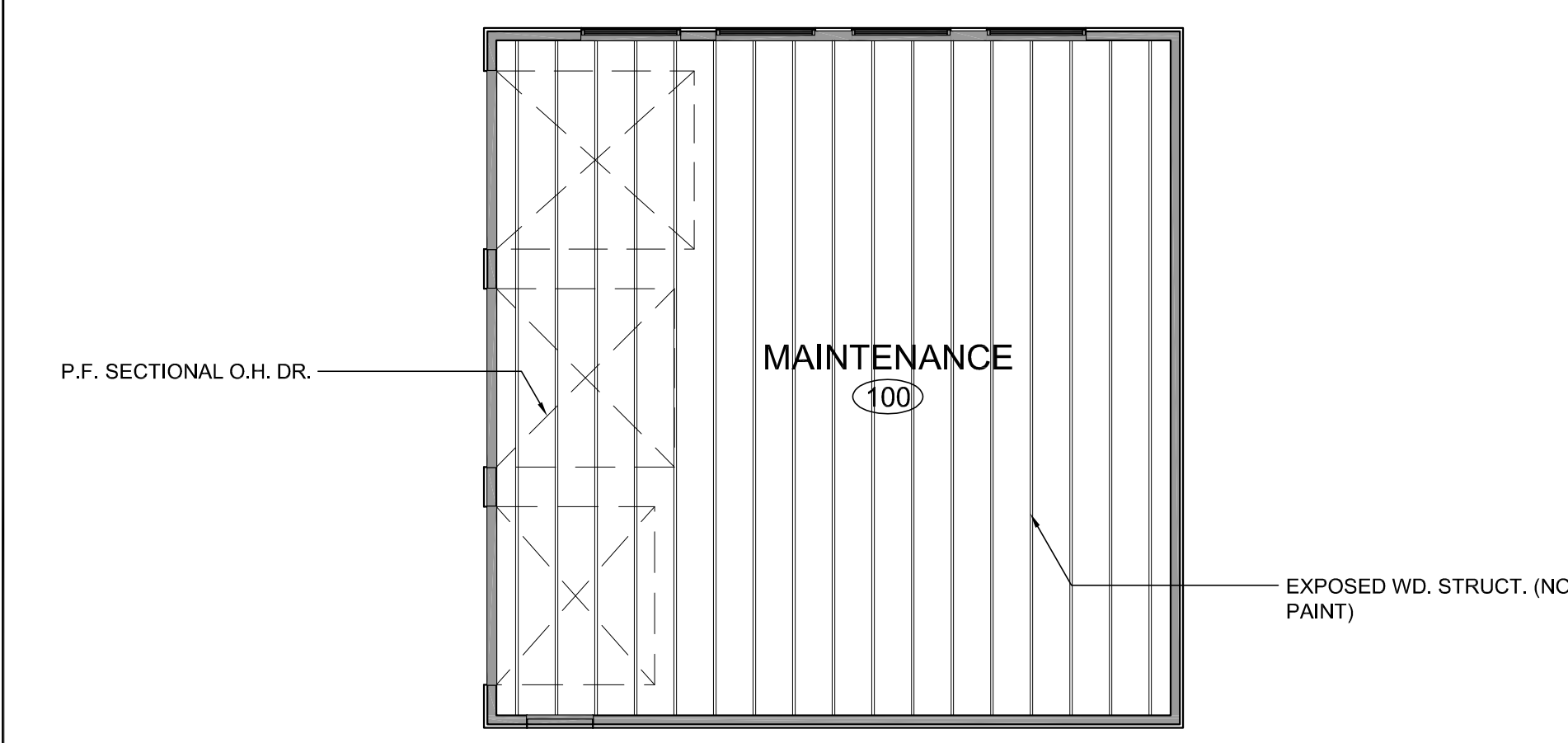
REFLECTED CEILING PLAN 1/8"=1'-0"
