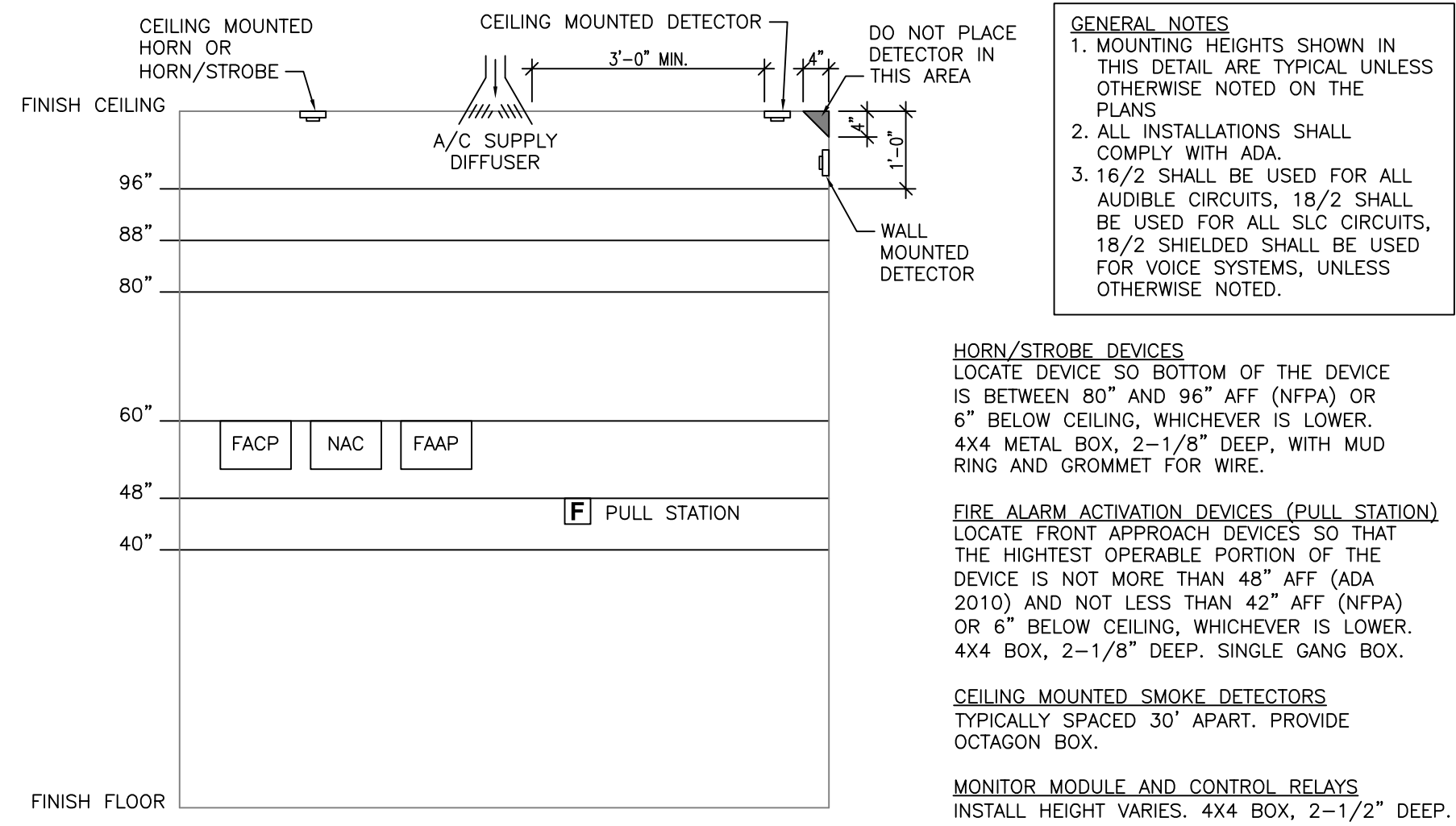
TYP. MTG. HEIGHTS DETAIL
