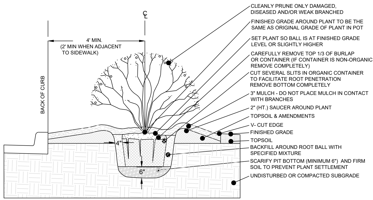
TYP. SHRUB PLANTING ADJACENT TO CURB NO SCALE
