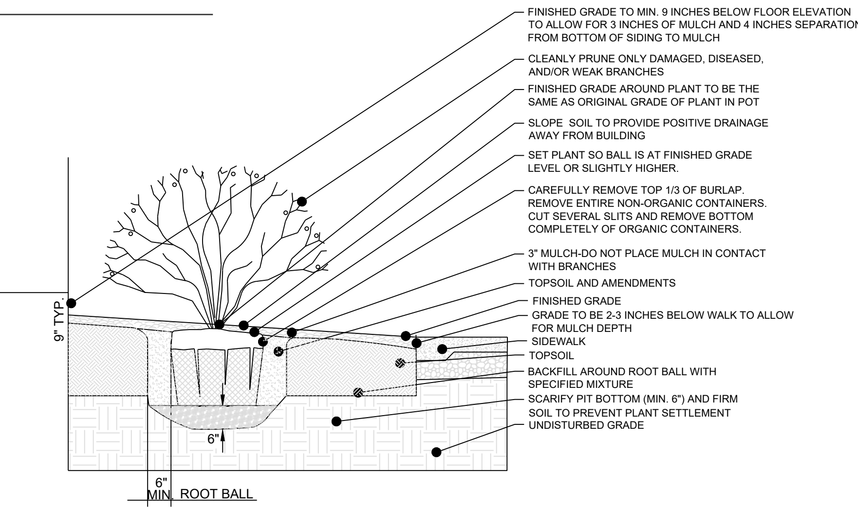
TYP. SHRUB PLANTING ADJACENT TO BUILDING NO SCALE
