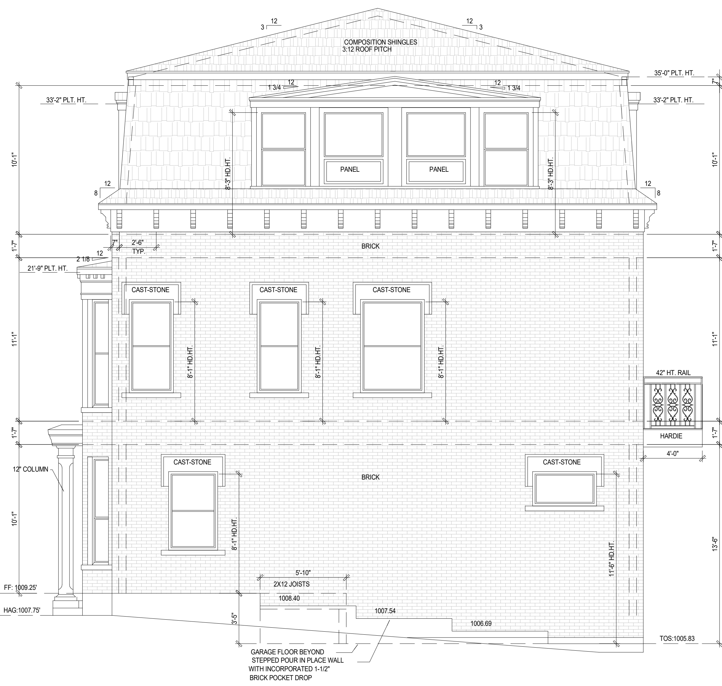
01 | BUILDING 2 - RIGHT ELEVATION 1/4" = 1'-0"
