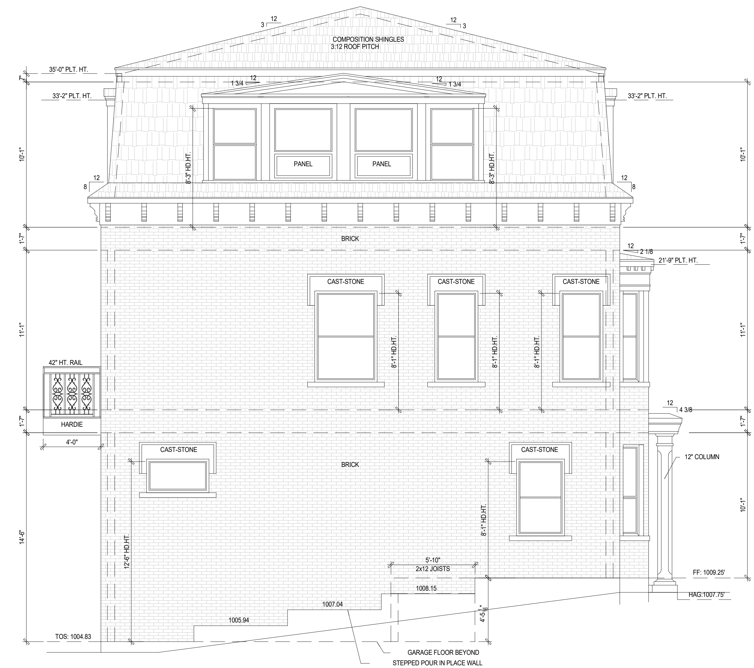
03 | BUILDING 2 - LEFT ELEVATION 1/4" = 1'-0"
