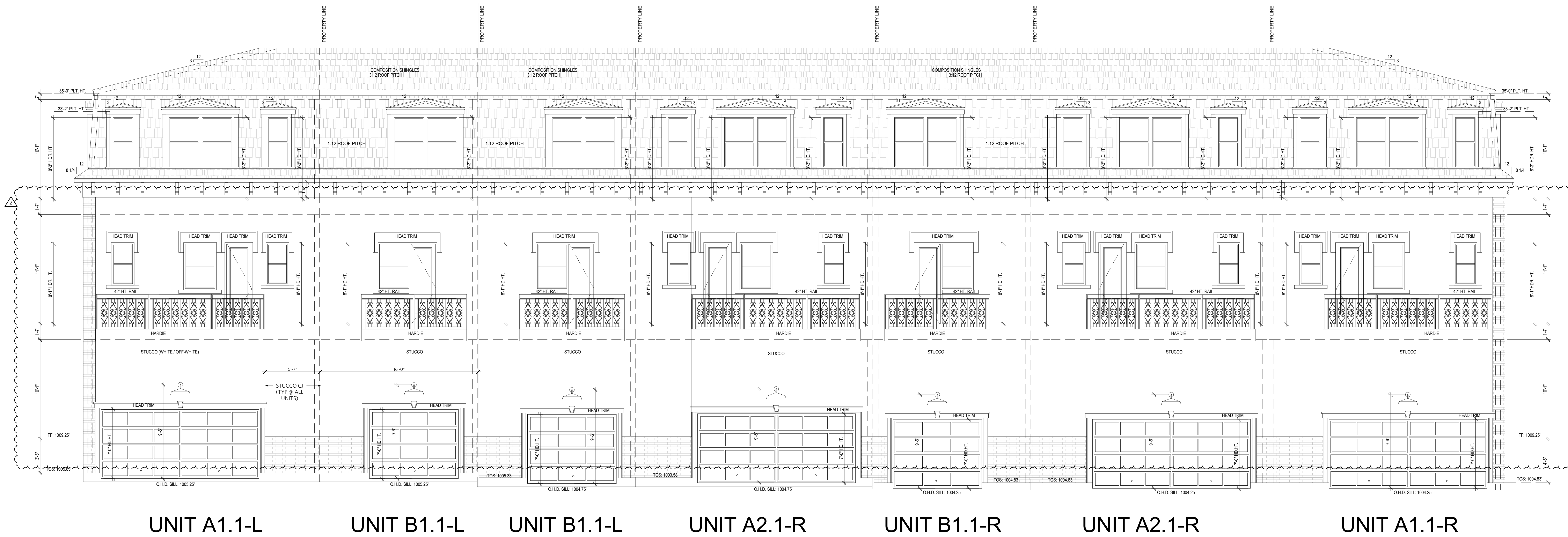
04 | BUILDING 2 - REAR ELEVATION 1/4" = 1'-0"
