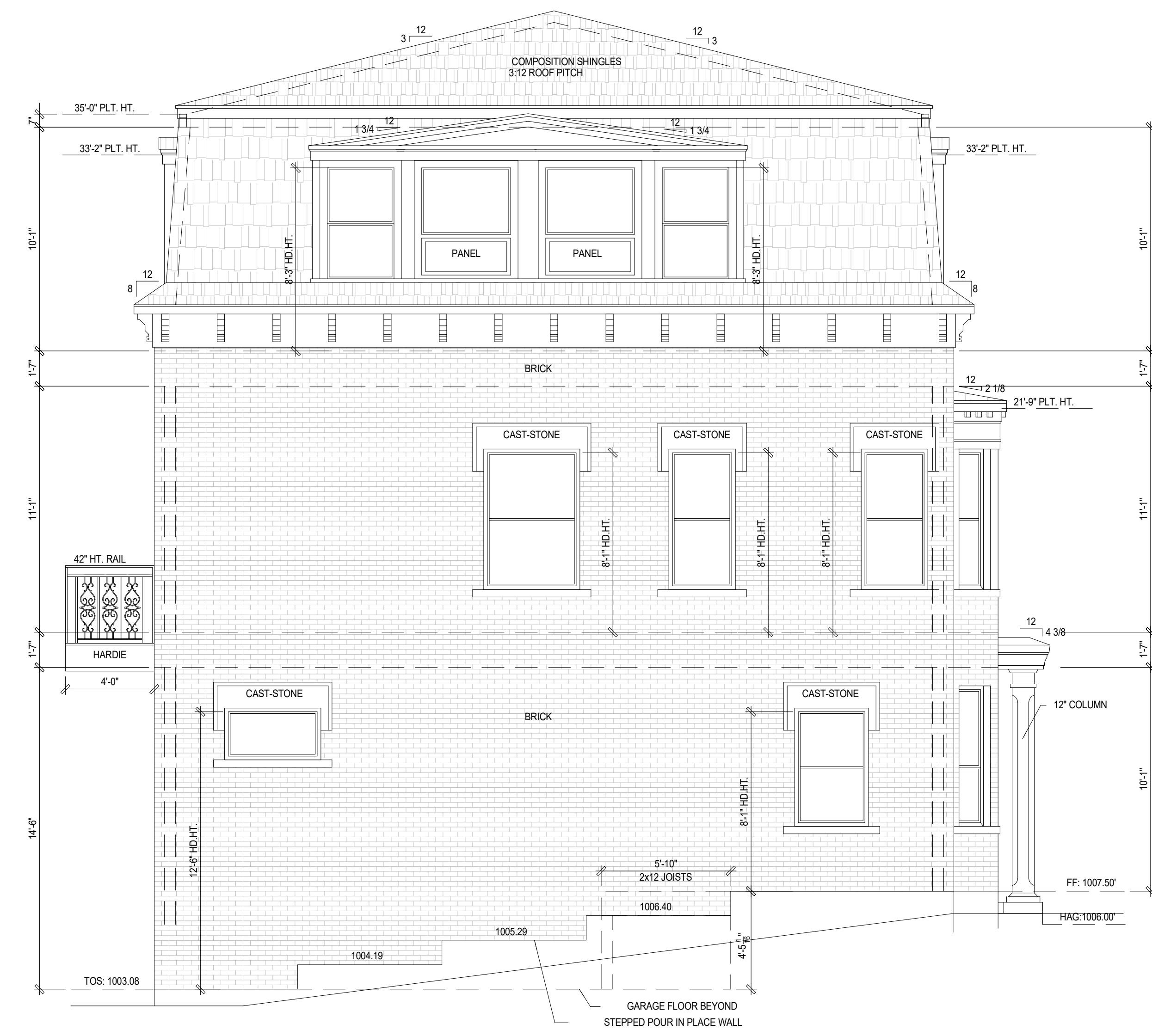
03 | BUILDING 1 - LEFT ELEVATION 1/4" = 1'-0"
