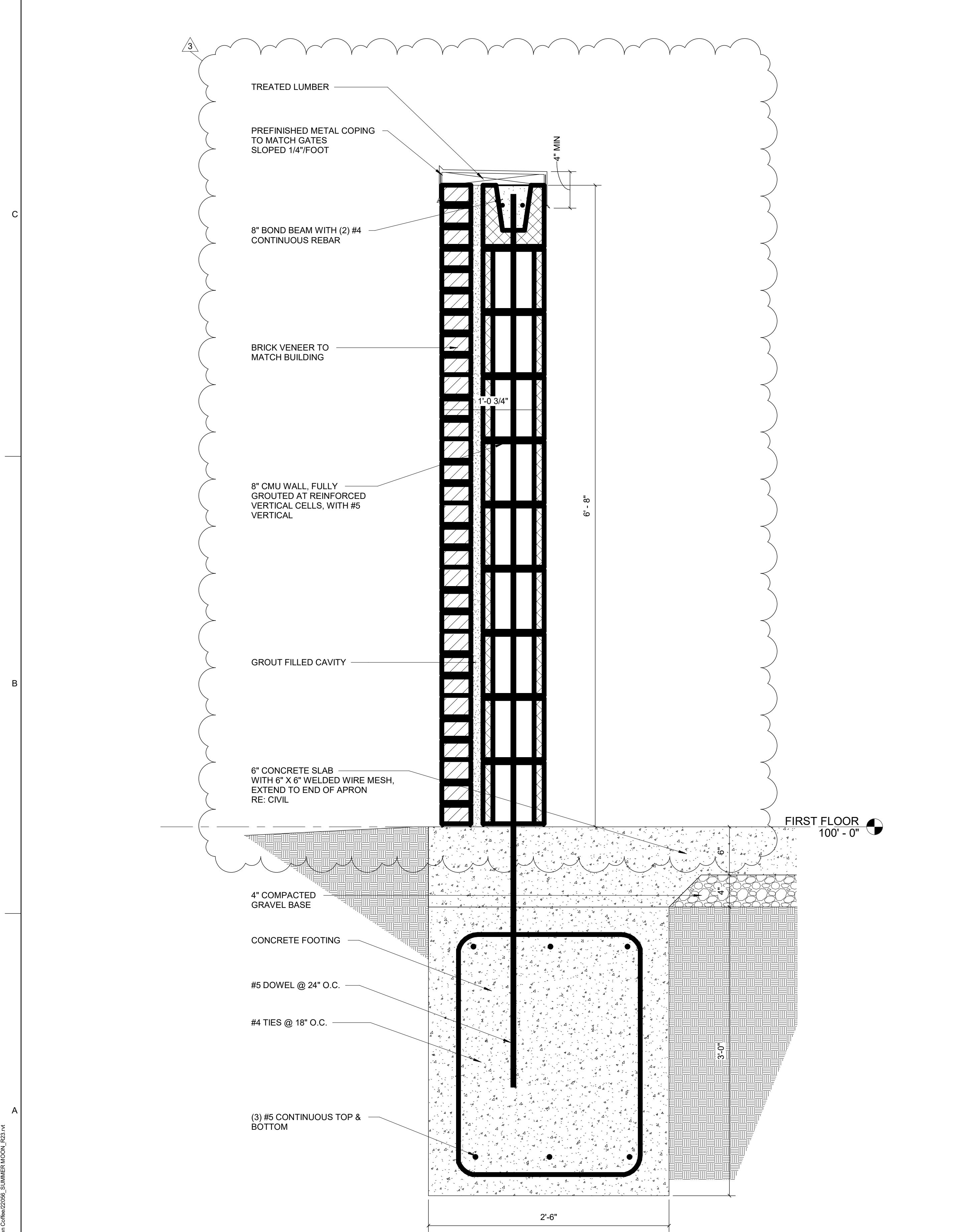
D5 TRASH ENCLOSURE SOUTH
