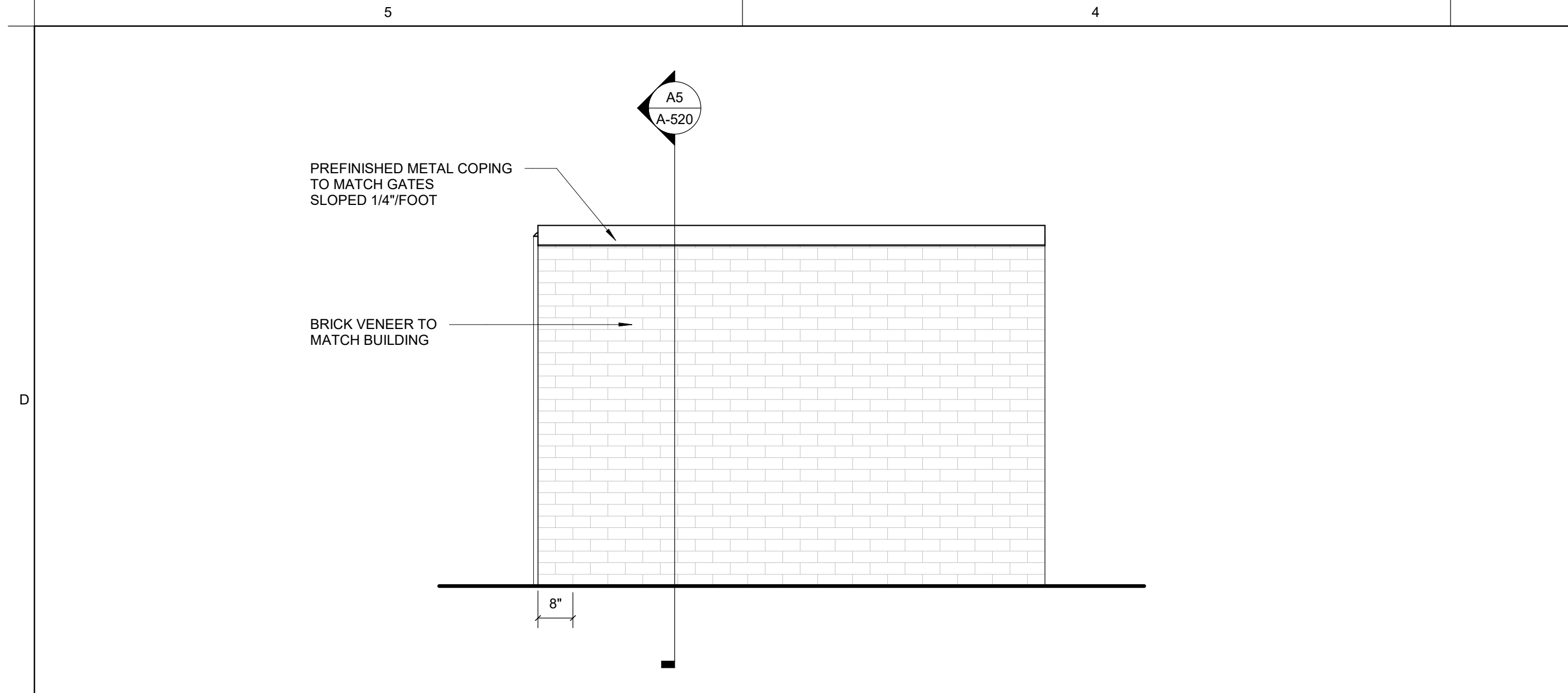
D5 TRASH ENCLOSURE SOUTH
