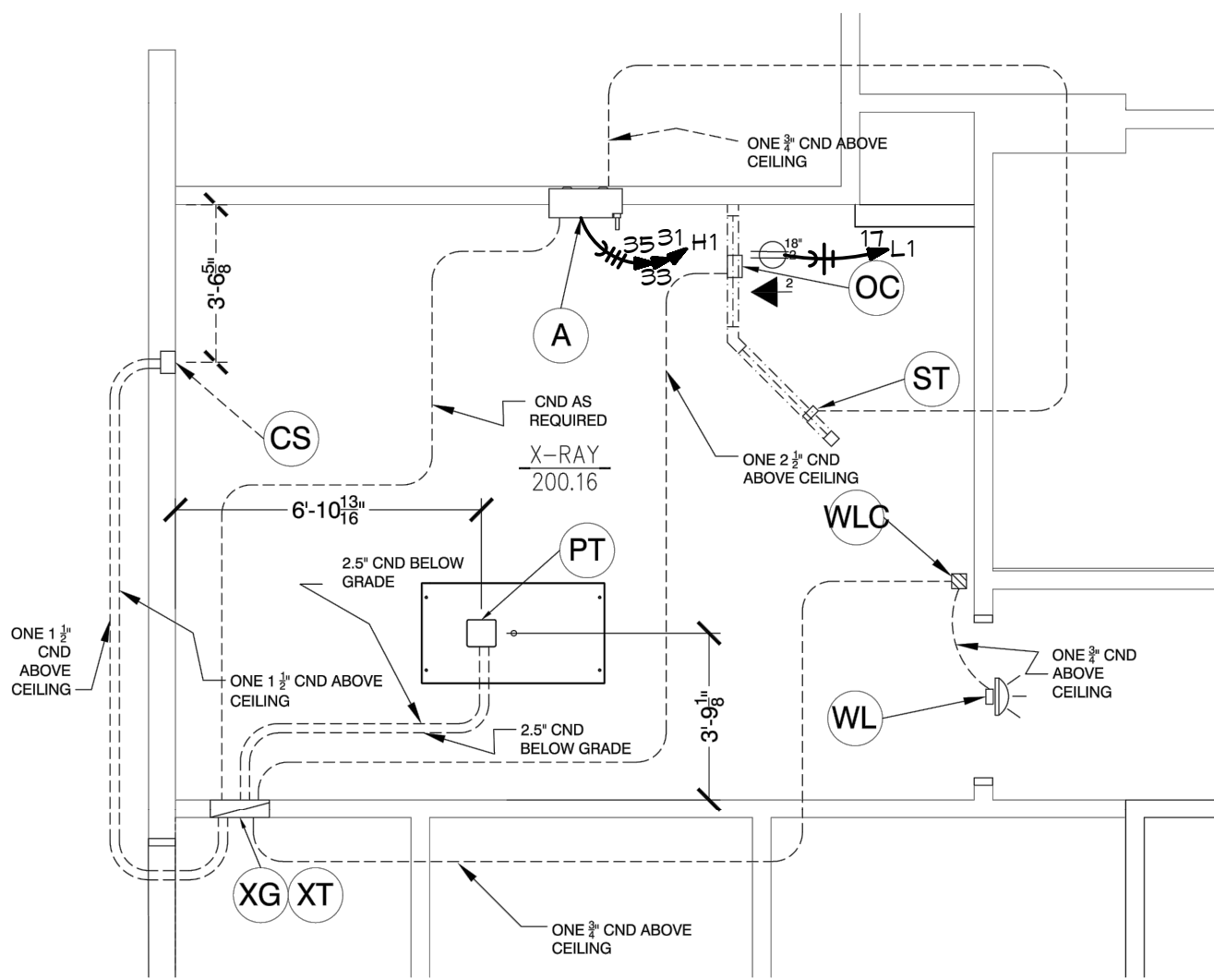
ELECTRICAL LAYOUT GE PROTEUS SCALE: 1/4" = 1'-0" MINIMUM CEILING HEIGHT: 9'-0"
