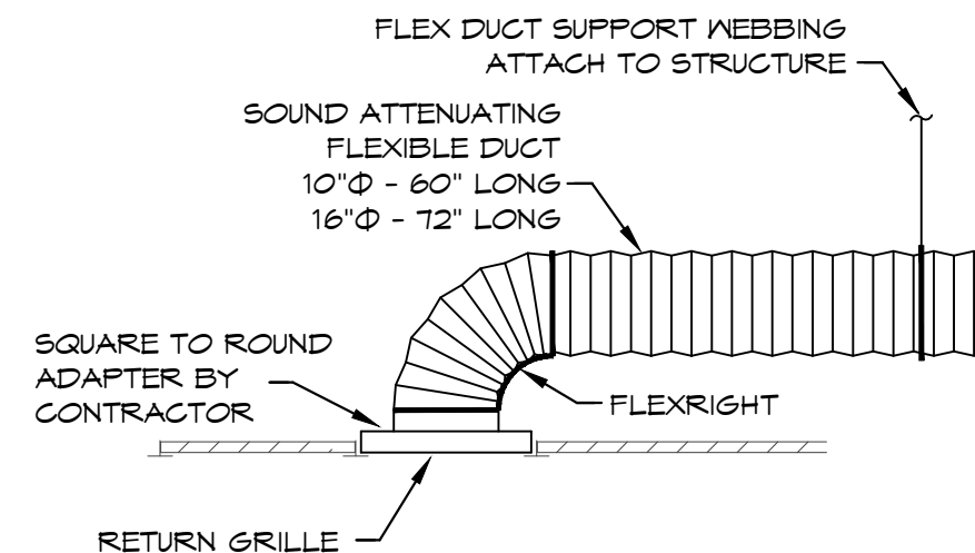
ACUSTICAL RETURN BOOT DETAIL SCALE: NONE
