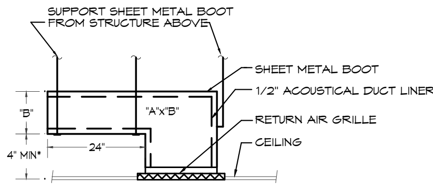
RA SOUND BOOT DETAIL NO SCALE
