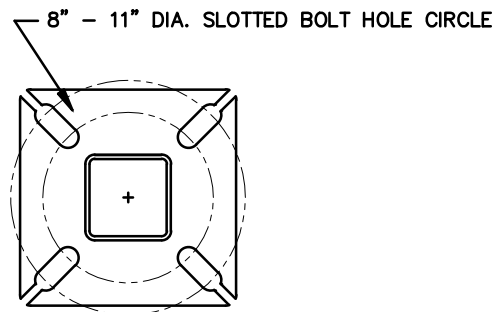
4" BASE PLATE DETAIL
