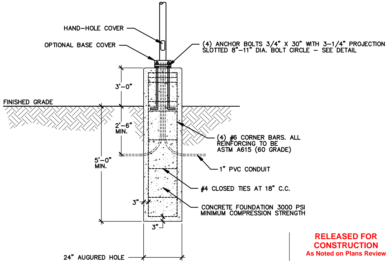
4" POLE, 24"Ø BASE DETAIL
