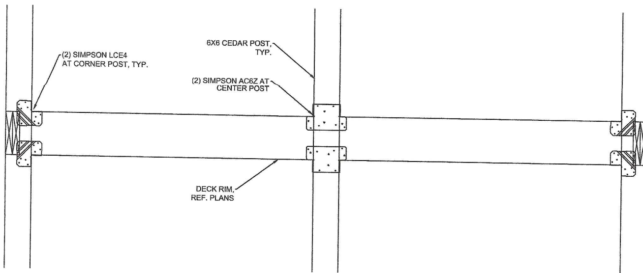
Figure 1.0 – Post Splice Repair
