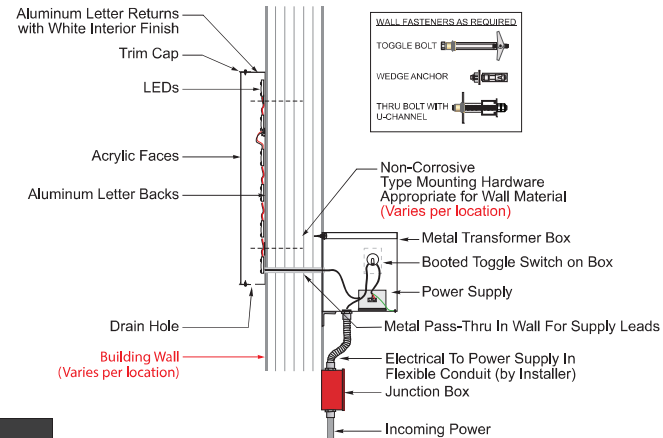
FACE LIT CHANNEL LETTER - REMOTE (EXTERIOR)
