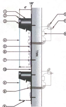
FACE-LIT CHANNEL LETTERS - FLUSH MOUNTED SCALE: NTS
