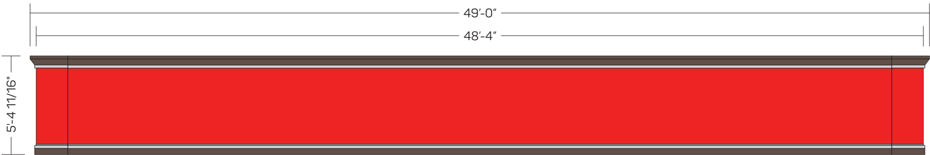
EXISTING 5'-4 11/16" X 48'-4"
