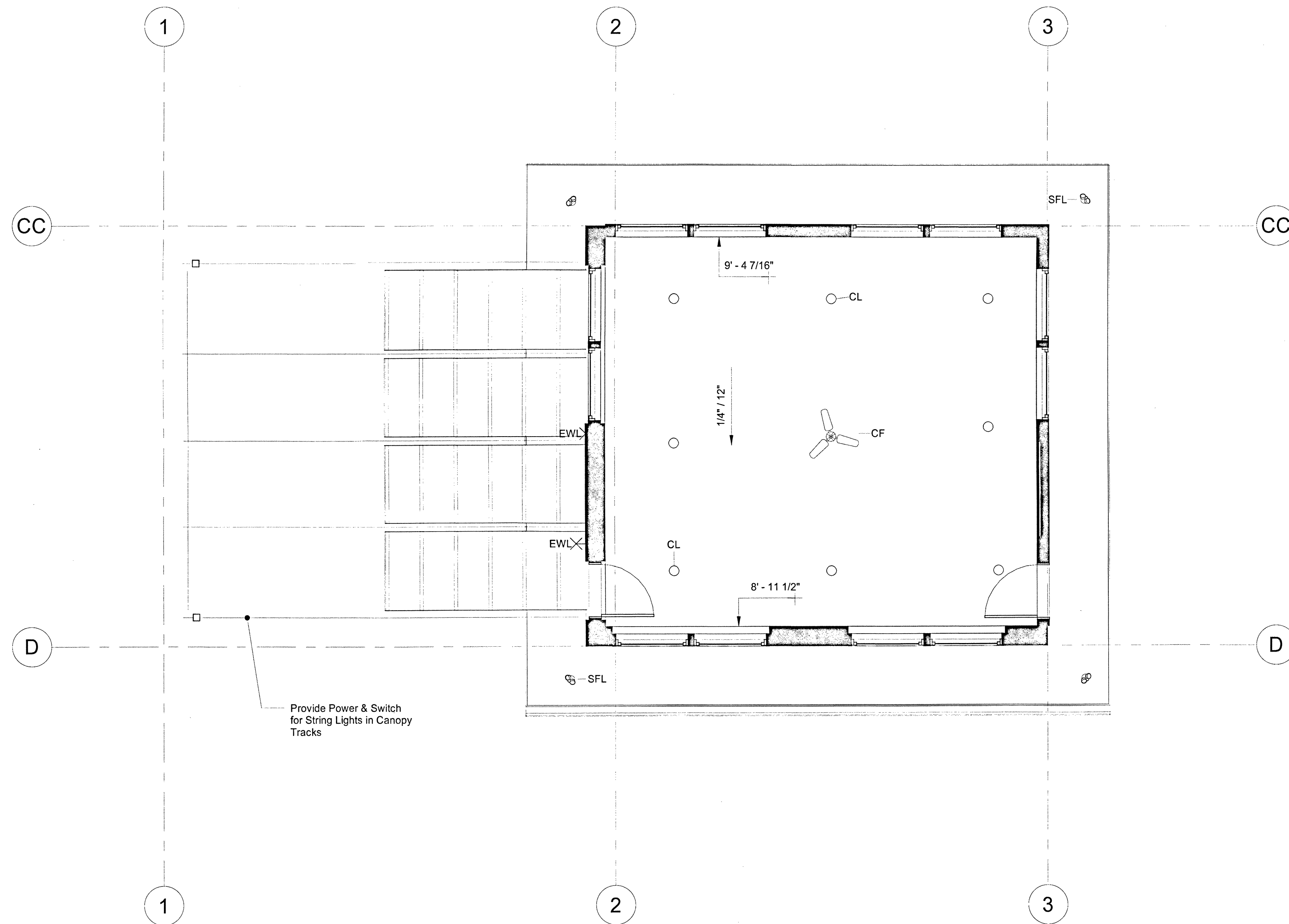
1 Upper Floor Ceiling POLan 1/4" = 1'-0"
