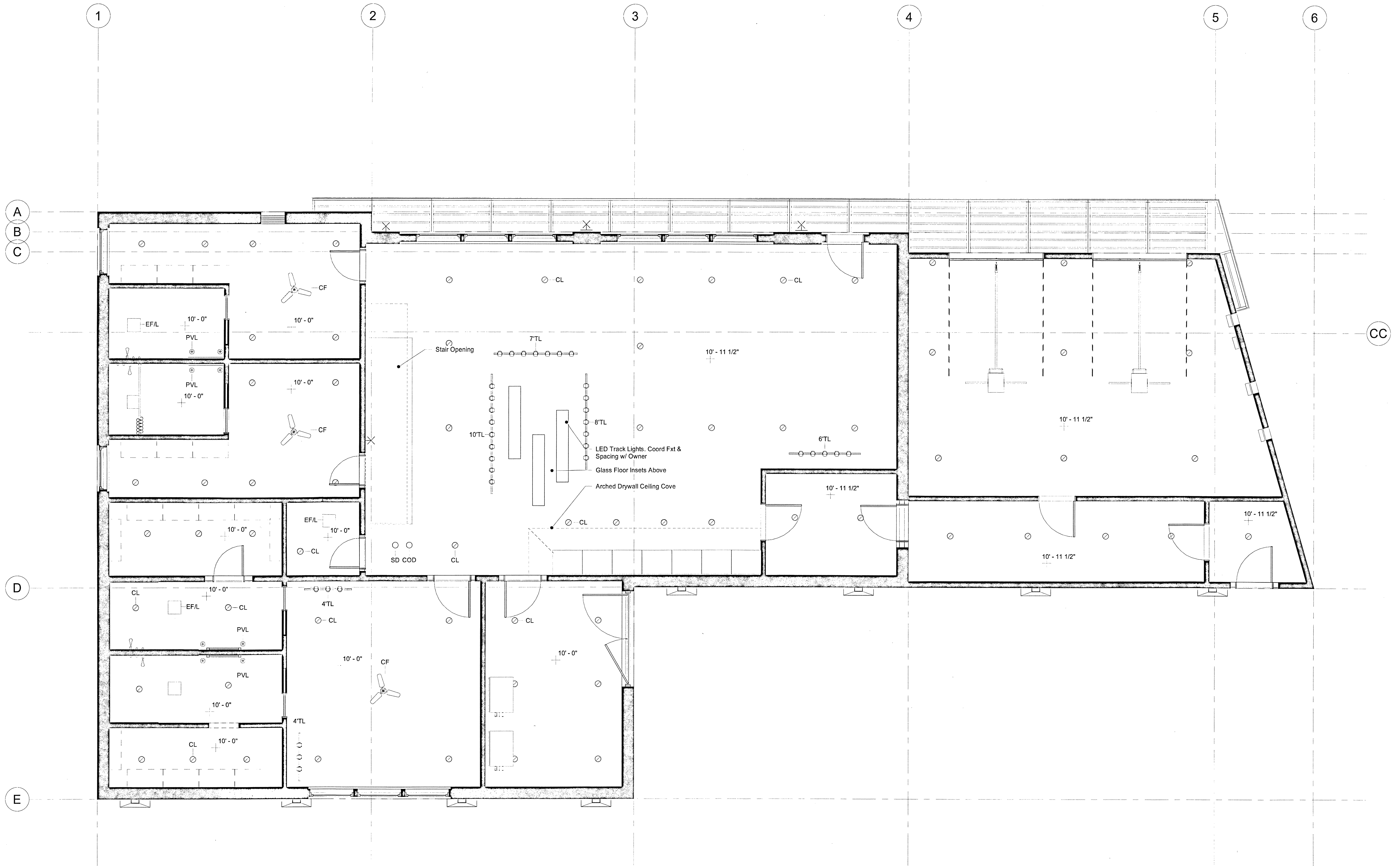
1 Main Floor Ceiling Plan 1/4" = 1'-0"
