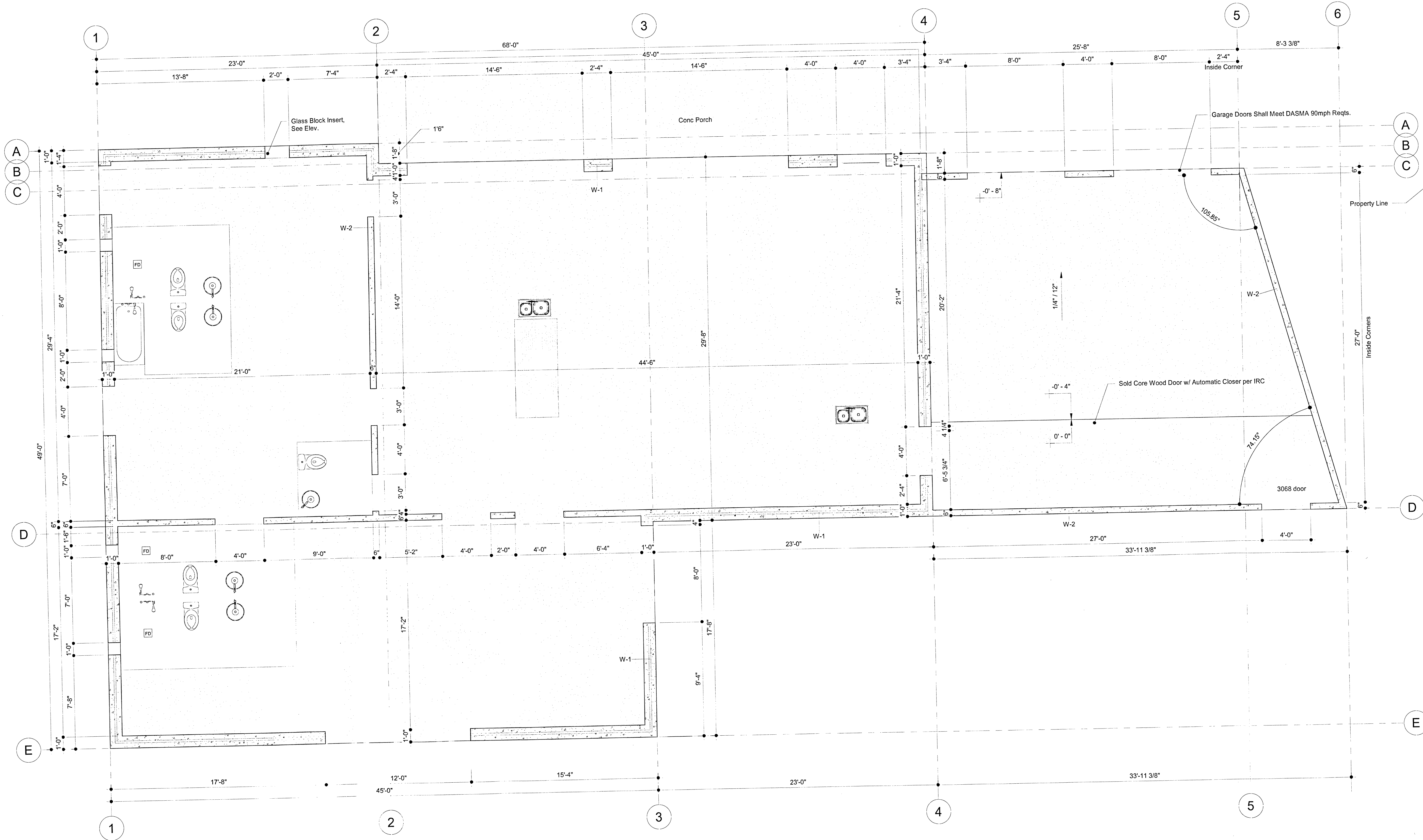
1 Main Concrete Layout 1/4" = 1'-0"
