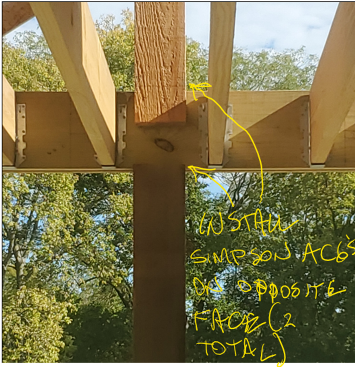
Figure 3 – Middle post
