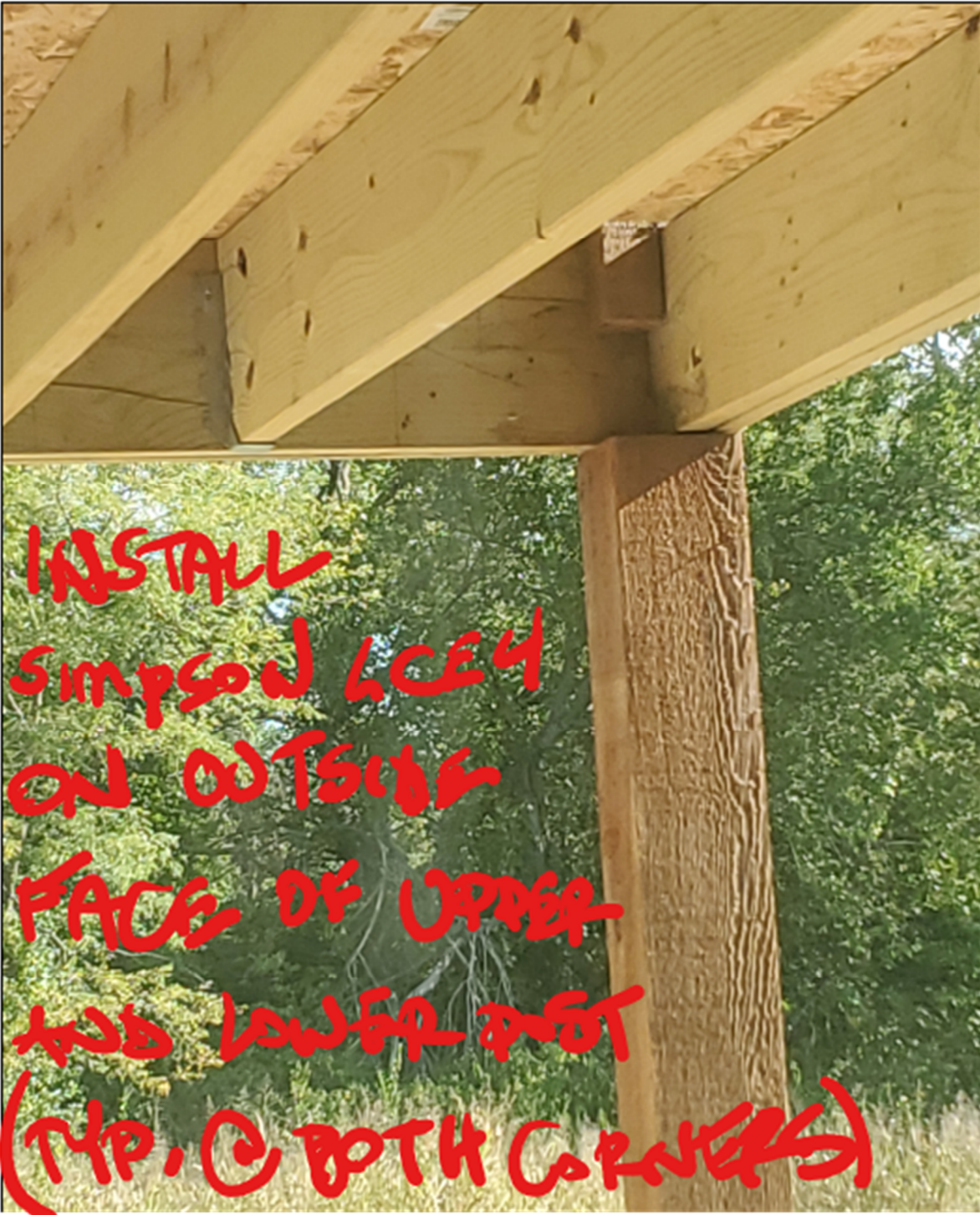
Figure 2 – Corner Posts
